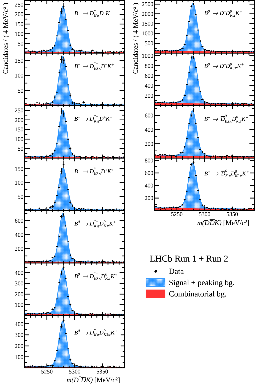
Figure 2: Fits to the invariant-mass distributions m(D^{(*)}\bar{D}K) of (left) B \rightarrow D^* \bar{D} K and (right) B \rightarrow D \bar{D} K for the combined Run 1 and Run 2 samples. The stacked components are (red) combinatorial background and (blue) signal shape.
