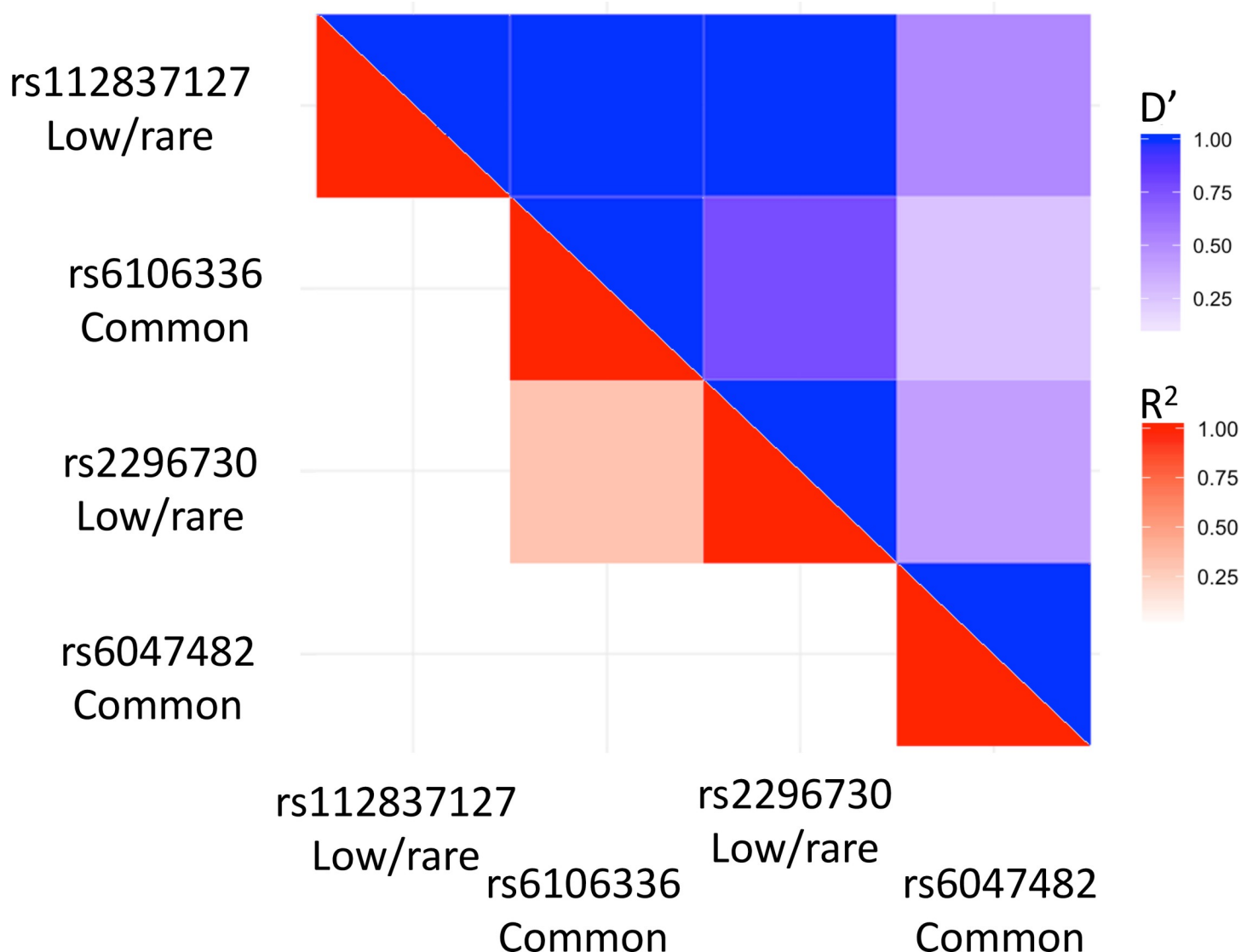
Fig 2. Patterns of Linkage Disequilibrium (LD) for rare, low-frequency and common variants associated with EwS at the chromosome 20p11.22–23 susceptibility locus. R 2 values are in shades of red while D' values are in shades of blue, with darker values indicating higher degree of LD. All LD measures were estimated in LDlink using 1,000 Genomes Project European populations as the reference panel.
