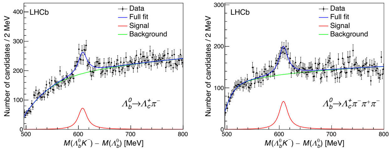
FIG. 4. Distribution of reconstructed \delta M_K = M(\Lambda_b^0 K^-) - M(\Lambda_b^0) in \Xi_b(6227)^- \rightarrow \Lambda_b^0 K^- candidate decays, with (left) \Lambda_b^0 \rightarrow \Lambda_c^+ \pi^- and (right) \Lambda_b^0 \rightarrow \Lambda_c^+ \pi^- \pi^+ \pi^- candidates. The fit projections are overlaid.
