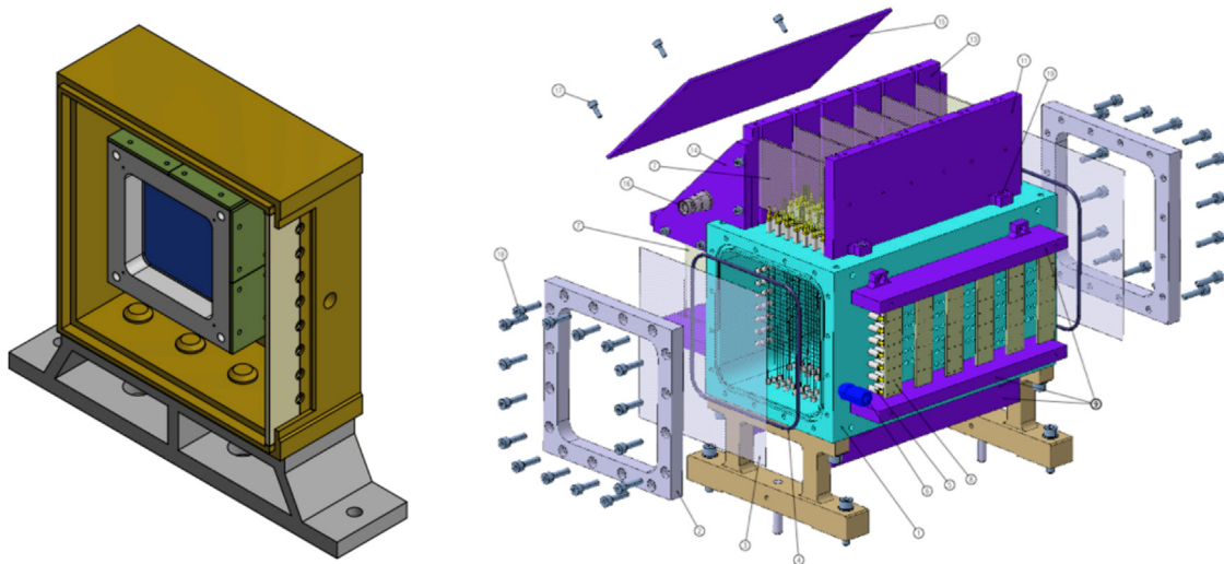
FIGURE 2 | Left: Start Counter detector inside the plastic box. The aluminum mechanical structure holds the EJ-228 plastic scintillator foil (in dark blue). Right: Technical drawing of the Beam Monitor drift chamber. The two orthogonal views x - y of the wires are clearly visible. Two enclosing mylar windows held by aluminum frames are shown as well.
