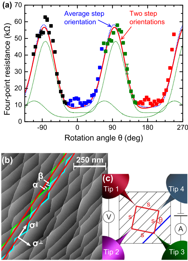
FIG. 3 (color online). (a) Four-point resistance measured on a Si(111)-(7 × 7) surface in the square configuration [shown in (c)] with s = 50 \mu\text{m} as a function of rotation angle \theta between the average step orientation and the line connecting the current injecting tips (the colored data points). The fits to the data using either only one average step direction or a superposition of two step orientations (the respective parts are shown as green dotted lines) are indicated as a dotted blue line and a solid red line, respectively. (b) STM image of the Si(111)-(7 × 7) surface showing the representative step arrangement on the sample. Two adjacent step edges are highlighted (the solid green and blue lines), consisting of two main step directions indicated by the angles \alpha and \beta relative to the average step orientation (the solid red lines).
