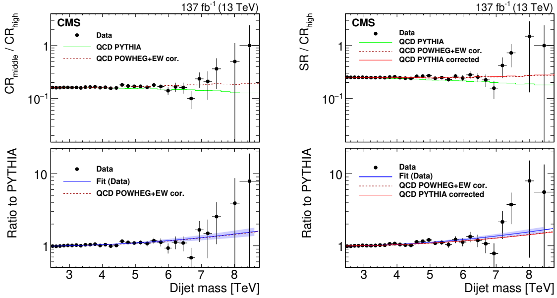
Figure 4. The ratio R_{\text{aux}} , the auxiliary transfer factor, calculated for data, PYTHIA, and POWHEG with electroweak corrections (left, upper panel). The double ratio of the same quantities in the upper left panel to R_{\text{aux}} from PYTHIA, along with the fit of the double ratio for data with the correction function (left, lower panel). The ratio R , the transfer factor, calculated for data, PYTHIA, POWHEG with electroweak corrections, and corrected PYTHIA (right, upper panel). The double ratio of the same quantities in the upper right panel to R from PYTHIA, along with the fit of the double ratio for data with a correction function, and corrected PYTHIA using \text{CR}_{\text{middle}} (right, lower panel). The fits in the two lower panels agree with each other within their uncertainty at 95% CL (shaded bands).
