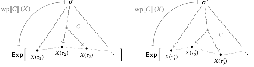
Fig. 1. The weakest preexpectation \text{wp}[C](X) maps every initial state \sigma to the expected value of X , measured with respect to the final distribution over states reached after termination of program C on input \sigma . \text{wp}[C] is backward-moving in the sense that it transforms an X: \Sigma \rightarrow \mathbb{R}_{\geq 0}^\infty , evaluated in final states after termination of C , into \text{wp}[C](X): \Sigma \rightarrow \mathbb{R}_{\geq 0}^\infty , evaluated in initial states before execution of C .
