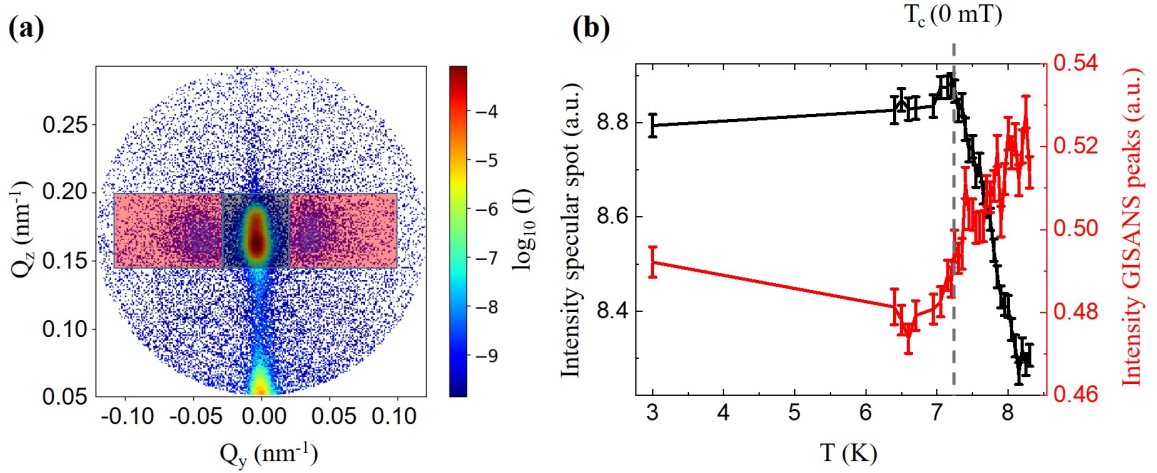
Figure 7.1: (a) Q_y - Q_z -map of \text{SF}_{\text{high}}(1) at T = 8.3 \text{ K} , above the superconducting critical temperature. (b) Integrated intensities I_{\text{spec}} and I_{\text{GIS}} over the areas displayed by black and red boxes in (a), respectively, and with dependence on temperature. The grey vertical line denotes T_c = (7.247 \pm 0.001) \text{ K} of \text{SF}_{\text{high}}(1) at 0 \text{ mT} .
