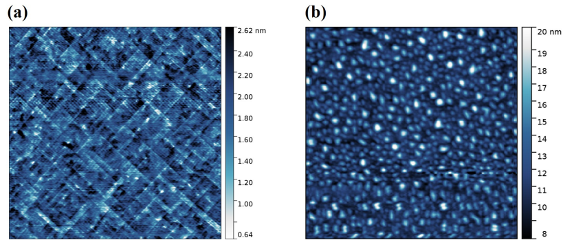
Figure 5.13: 3 \times 3 \mu\text{m} AFM measurements of sample F_{\text{high}}(4) in the as-grown state with a flat surface (a) and after three weeks of sample aging with islands of \sim 20 nm height (b).
