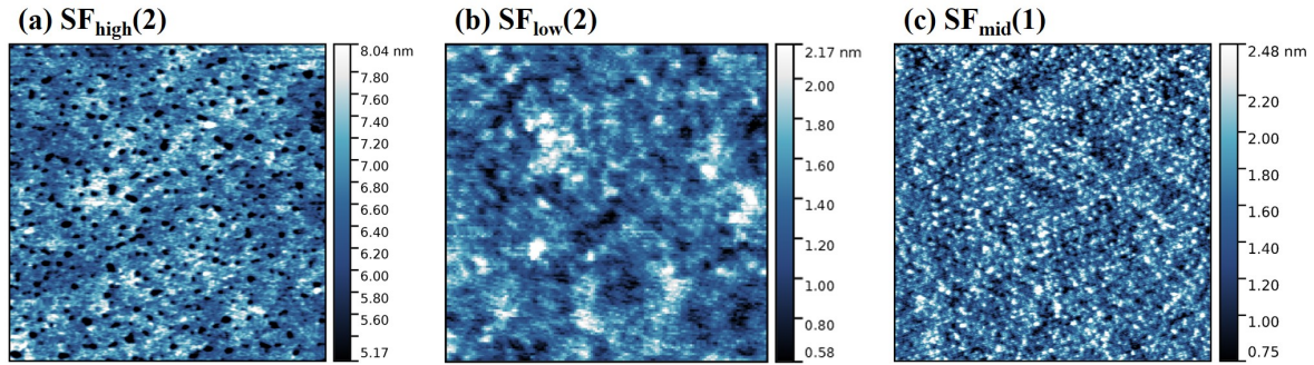
Figure 9.9: 3x3 \mu\text{m} AFM images of samples \text{SF}_{\text{high}} - \text{SF}_{\text{low}} at room temperature.
