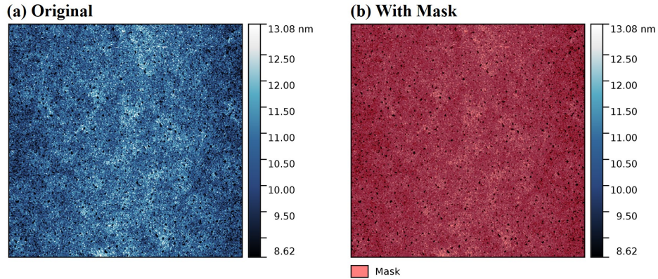
Figure 9.10: (a) 8x8 \mu\text{m} AFM image of \text{SIF}_{\text{high}} (1) displaying deep voids inside the FePd layer. (b) The red area denotes a mask added to the AFM image where the surface height is >60% above the minimum height level, the voids (black area) obtain a relation to the FePd surface of \sim 1\% .
