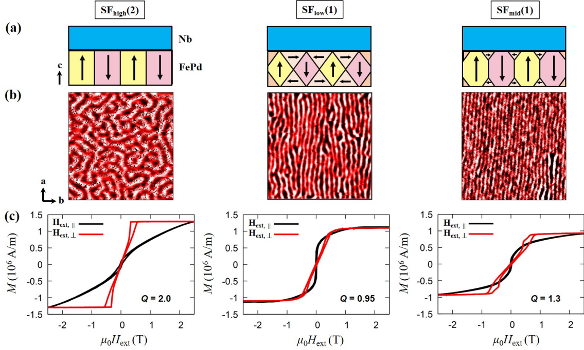
Figure 5.15: From left to right: SF_{high}(2) , SF_{low}(1) , and SF_{mid}(1) , respectively. (a) Schematic view of the magnetic domain formation inside the FePd layer and the toplayer of Nb in direction of the c-axis of L1_0 -ordered FePd. (b) ( 3 \times 3 \mu\text{m} ) zero-field MFM measurements in the as-grown state of SF_{high}(2) and SF_{mid}(1) and after demagnetization of SF_{low}(1) . (c) Hysteresis loops measured at 300 K with H_{ext, \parallel} in the surface plane and H_{ext, \perp} perpendicular to the surface plane, adapted from [182]. All measurements are obtained at 300 K.
