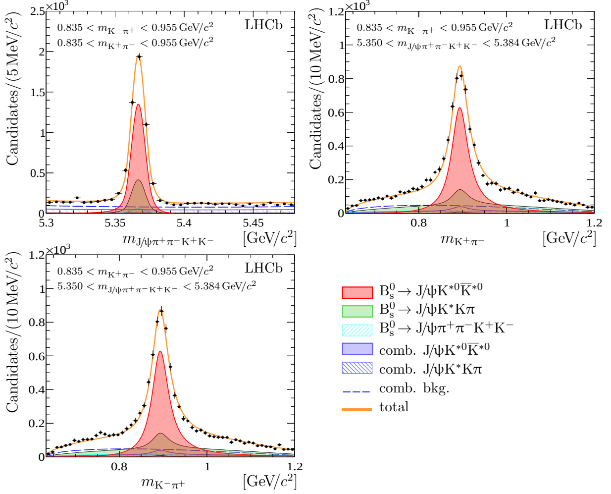
Figure 6: Distributions of the (top left) J/\psi \pi^+ \pi^- K^+ K^- , (top right) K^+ \pi^- and (bottom left) K^- \pi^+ mass of selected B_s^0 \rightarrow J/\psi K^{*0} \bar{K}^{*0} candidates shown as points with error bars. A fit, described in the text, is overlaid.
