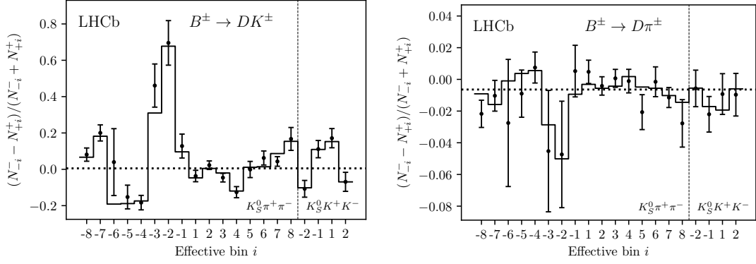
Figure 6: The bin-by-bin asymmetries (N_{-i}^- - N_{+i}^+)/ (N_{-i}^- + N_{+i}^+) for each Dalitz-plot bin number for (left) B^\pm \rightarrow DK^\pm decays and (right) B^\pm \rightarrow D\pi^\pm decays. The prediction from the central values of the CP -violation observables is shown with a solid line and the asymmetries obtained in fits with independent bin yields are shown with the error bars. The predicted asymmetries in a fit that does not allow for CP violation are shown with a dotted line. The vertical dashed line separates the K_S^0\pi^+\pi^- and K_S^0K^+K^- bins on the horizontal axis.
