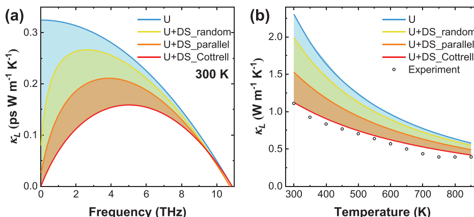
Figure 4. Thermal conductivity impacted by dislocations. a) The calculated spectral lattice thermal conductivity ( \kappa_L ) at 300 K and b) temperature dependence of \kappa_L using the modelled scattering terms from the Umklapp process (U) and dislocation strain field (DS) comparing random versus parallel dislocation arrangements and the effect of the Cottrell atmosphere. The experimental \kappa_L values [25] are plotted as a reference.
