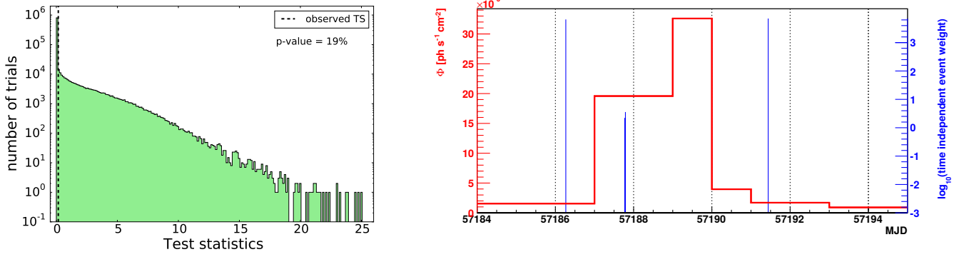
Figure 14. Result of the 11-day (MJD 57184 - 57195) analysis. Left: test statistics for 10^6 background trial scrambled data in green. The black dashed line shows the TS value resulting from the analysis. Right: The red line is the denoised light curve of 3C 279. The blue vertical lines represent IceCube events selected by the analysis and their size is given by the product of the signal over the background spatial and energy PDFs. The threshold is not represented since it was fitted to zero. No correlation is found between the flare of 3C 279 and neutrinos detected by IceCube.
