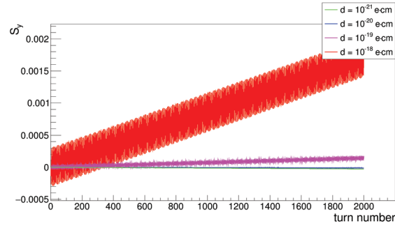
Figure 5.13: Vertical spin component for different EDM values. For the tracking calculation, a field amplification factor of 1000 was used to decrease the computing time and to enhance the spin behavior. The amplitude as well as the slope of the slow spin buildup clearly increase with larger EDM values which is in agreement with the theoretical prediction.
