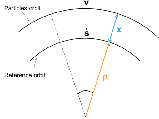
Figure 3.2: The velocity of an arbitrary particle in the beam is not equal to the velocity of the reference particle. It is larger (smaller) for particles that move on an outer (inner) path relative to the reference particle. Adapted from [36].
