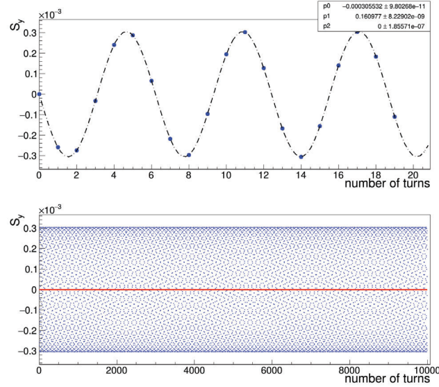
Figure 5.6: Tracking results for an initial spin along the momentum axes and an EDM of 10 \cdot 10^{-18} e cm ( \eta_{\text{EDM}} = 1.902052 \cdot 10^{-4} ). The invariant spin axis is tilted according to Equation (4.53) and the vertical spin component therefore performs fast oscillations. Over time, the EDM signal vanishes and the net spin buildup is zero.
