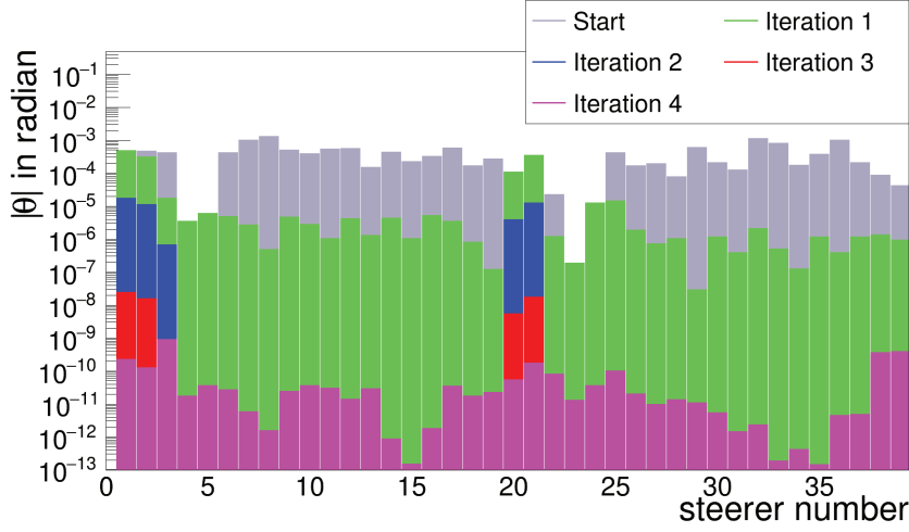
Figure 7.3: Steerer kick values in radian after each iteration of the orbit matching algorithm. The initial kicks are distributed according to a Gaussian distribution with a width of 0.5 mrad.
