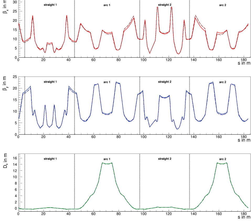
Figure 6.7: Optical functions \beta_x , \beta_y and D_x for the quadrupole strengths given in Table 6.1. The optical functions for the old effective quadrupole lengths is given by the solid lines, the optics according to the new effective lengths is shown by the dashed lines. The betatron tunes for the old lattice are Q_x = 3.68915 in horizontal direction and Q_y = 3.72521 in vertical direction., the ones for the new lattice are Q_x = 3.66564 and Q_y = 3.70662 .
