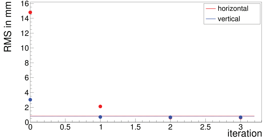
Figure 7.4: Closed orbit RMS values of the simulated orbits after each iteration of the orbit matching algorithm. Initially, all steerer kicks are set to zero. The target orbits are the measured orbits from the October 2019 beam time. The dashed lines (red: horizontal, blue: vertical) indicate the RMS values of the measured orbits.
