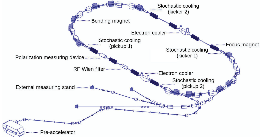
Figure 5.1: Sketch of the synchrotron COSY and the pre-accelerator JULIC including the main magnets, cooling sections, the RF Wien filter device and the polarimeter. Adapted from [62].
