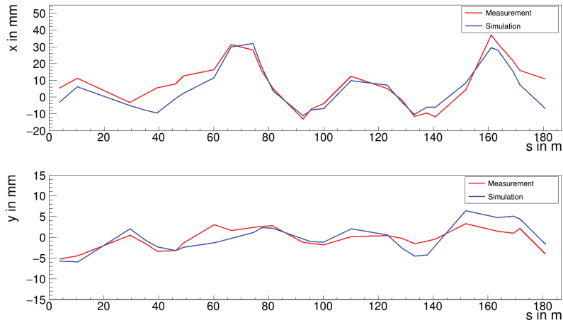
Figure 6.9: Simulated and measured orbit in horizontal and vertical direction. The simulation includes the additional kicks due to the shortening of the effective lengths of the dipoles and the magnet misalignments from Section 6.1. For the measurement, the orbit correction was turned off in order to see the uncorrected orbit that is present when only the dipoles and quadrupoles are turned on.
