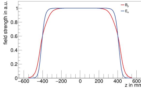
Figure 5.8: Normalized field distribution of the radial electric and vertical magnetic field along the longitudinal axis ( x = 0 and y = 0 ) inside the RF Wien filter device. The fringe field behavior of both fields differ. Therefore, the Lorentz force is locally different from zero and the particle motion is perturbed.
