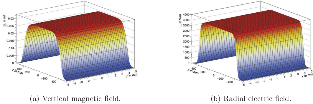
Figure 5.7: Grid field calculations of vertical magnetic and radial electric field at maximum amplitude for a vanishing vertical field component ( y = 0 ). The grid consists of one million grid points, i.e. 100 points in each direction. The transverse plane ( x and y ) covers a range of \pm 5 mm. The longitudinal range covers the complete length of the RF Wien filter device ( l_{WF} = 1100 mm).
