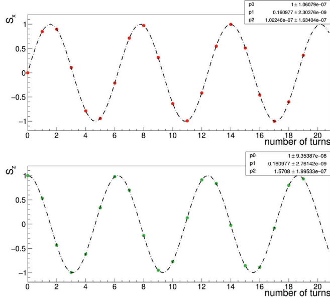
Figure 5.4: In-plane spin precession due to the MDM. The initial spin orientation is along the momentum vector and the spin precesses in the guiding fields of the dipoles. A sinusoidal fit was performed to determine the spin tune. The resulting value agrees with the theoretical prediction of |\nu_S| = -0.160977 .
