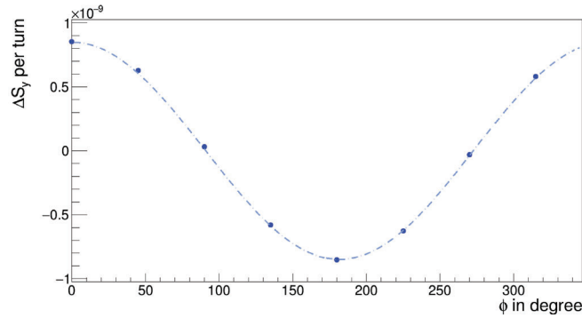
Figure 5.12: Average vertical spin buildup per turn as a function of the initial RF Wien filter phase \phi . The dashed line represents the theoretical predictions based on Equation (5.4). For a phase of \phi = 0^\circ the vertical spin buildup per turn is maximum and there is no buildup at all for an initial phase of \phi = 90^\circ .
