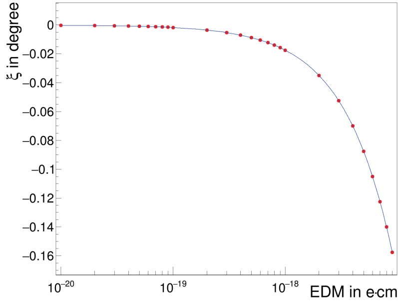
Figure 5.17: Determination of the invariant spin axis using spin tracking calculations. The plot shows the tilt angle \xi for different EDM values. The red dots represent the simulation results, the blue line indicates the theoretical predictions according to Equation (4.53).
