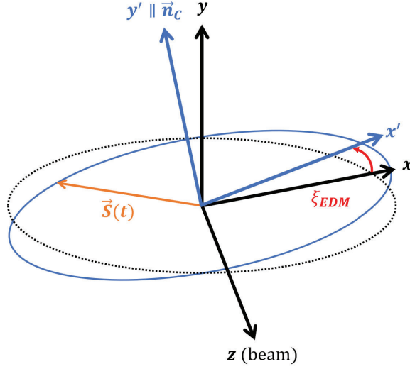
Figure 4.1: Sketch of the tilt \xi_{\text{EDM}} of the spin closed orbit due to the interaction of the EDM with the magnetic bending fields in a storage ring. The MDM and EDM contributions are perpendicular to each other. As a result, the vertical spin component oscillates.
