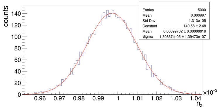
(b) Distribution of the longitudinal component of the invariant spin axis.
