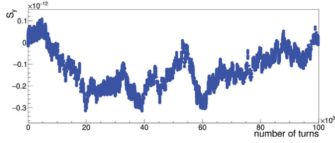
Figure 5.5: Vertical spin component of the reference particle with an initial spin pointing along the momentum vector and assuming a vanishing EDM. The vertical spin component is expected to stay zero. Due to the numerical limitations of the simulation, fluctuations of the order of 10^{-13} can be observed.
