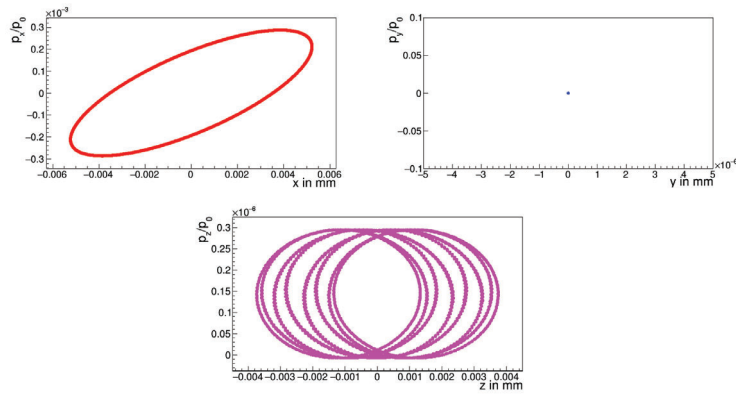
Figure A.1: Three-dimensional phase space of a particle with an initial horizontal offset at injection. Due to non-vanishing dispersion, different ellipses varying in their horizontal center position can be seen in the longitudinal phase space.
