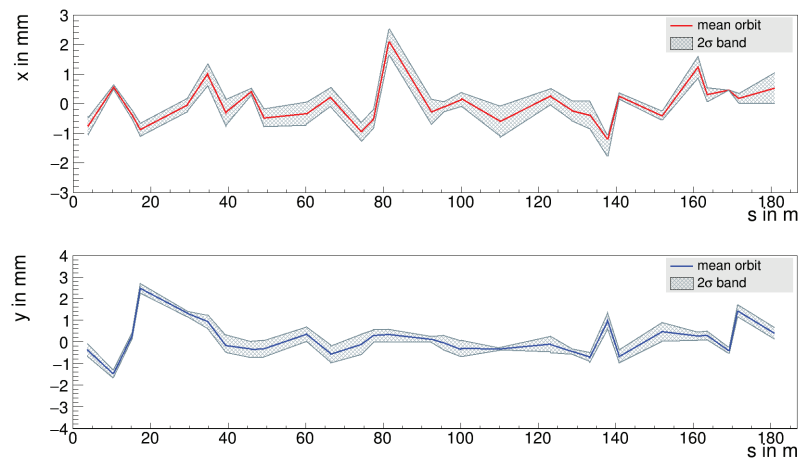
Figure 7.18: Closed orbits in horizontal (red) and vertical (blue) direction after fitting the model using the LOCO algorithm and matching the orbits by adjusting the steerer kicks. A 2\sigma range is shown based on randomly changed steerer kicks assuming an error of 1 % for each steerer setting.
