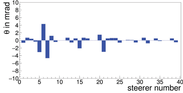
Figure 7.14: Final steerer settings after fitting the simulated closed orbits to the measured orbits using the method presented in Section 7.2.
