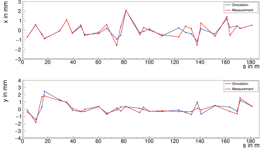
Figure 7.13: Closed orbits in horizontal and vertical direction after fitting the simulated orbits by changing the steerer kicks using the orbit matching method presented in Section 7.2 over five iterations.
