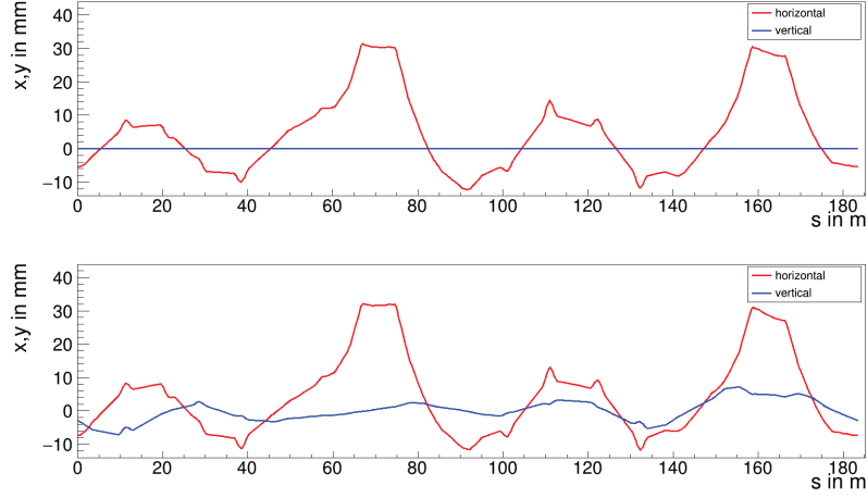
Figure 6.8: Horizontal (red) and vertical (blue) closed orbit resulting from shortened effective dipole length with an underlying ideal lattice (top) and including magnet misalignments (bottom). The horizontal closed orbit is clearly dominated by the shorter effective lengths of the dipoles which leads to orbit distortions up to 32 mm.
