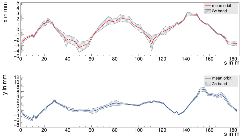
Figure 6.3: Closed orbits in horizontal and vertical direction including dipole and quadrupole misalignments. Both orbits (red and blue) show distortions of several millimeters compared to the default model with ideally positioned magnets. Additionally, a 2\sigma range is shown based on 10000 random settings according to Equation (6.2).
