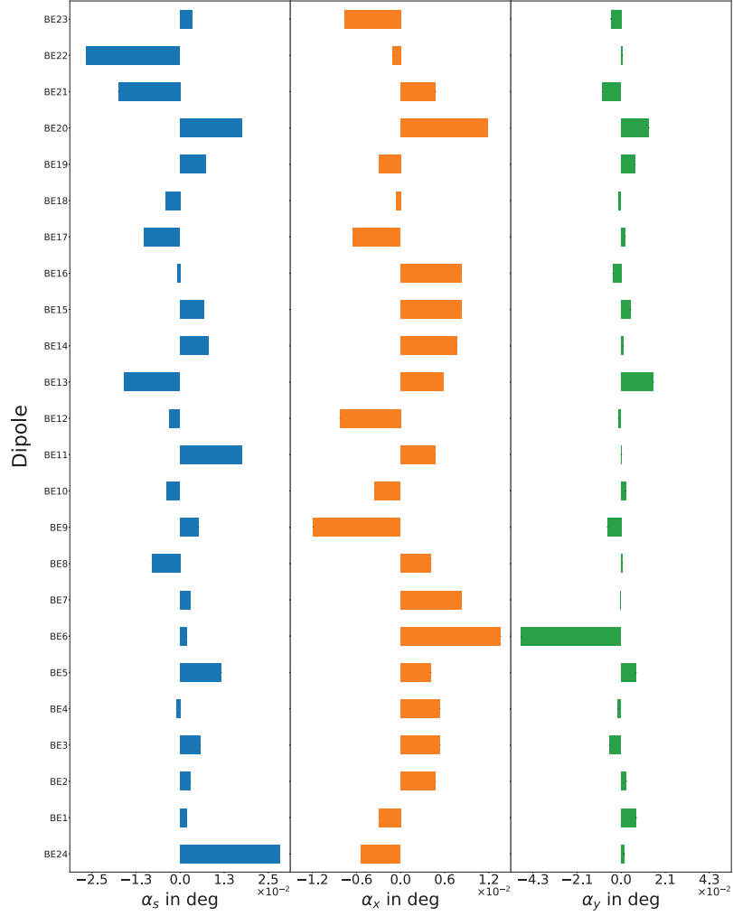
Figure A.4: Measured rotations of all dipoles including the measurement uncertainties. The individual 24 dipole magnets of COSY are denoted with B1, ..., B24. The measurements were performed in January 2020.
