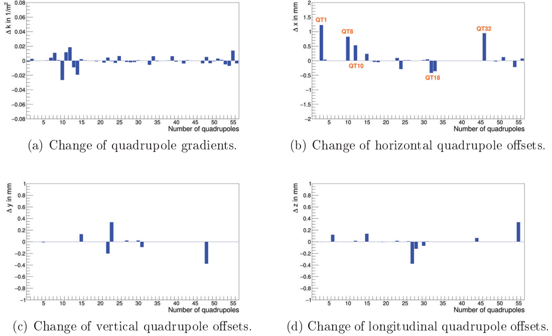
Figure 7.12: Changes of quadrupole gradients and positions after the final LOCO iteration.
