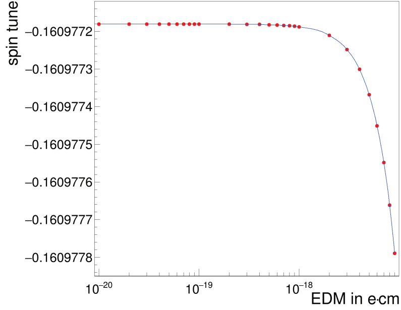
Figure 5.16: Spin tune determination using spin tracking calculations. The red dots represent the simulation results, the blue line indicates the theoretical predictions according to Equation (5.10).
