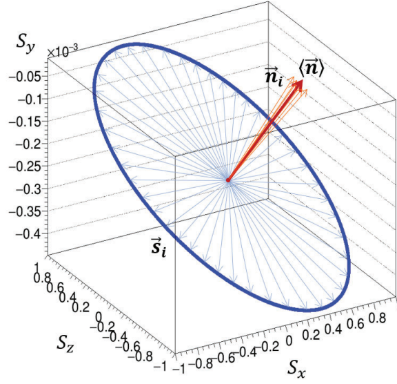
Figure 5.15: Spin tracking simulations using the reference particle moving on the closed orbit result in a well defined spin wheel. The invariant spin axis is the vector perpendicular to the plane that is defined by the spin wheel. The tilt of the invariant spin axis depends on the EDM value and other systematic effects such as magnet misalignments. For each turn, the normal vector \vec{n}_i is calculated. The average normal vector \langle \vec{n} \rangle is then considered as the invariant spin axis.
