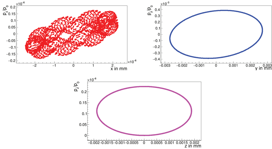
Figure 5.3: Three-dimensional phase space of a particle with an initial vertical offset at injection. The offset is chosen such that the vertical emittance \epsilon_y turns out to be 1 mm mrad. A well defined phase space ellipse can be seen in the vertical and the longitudinal phase space. Small distortions in the horizontal phase space are the result of dispersive areas in the arcs.
