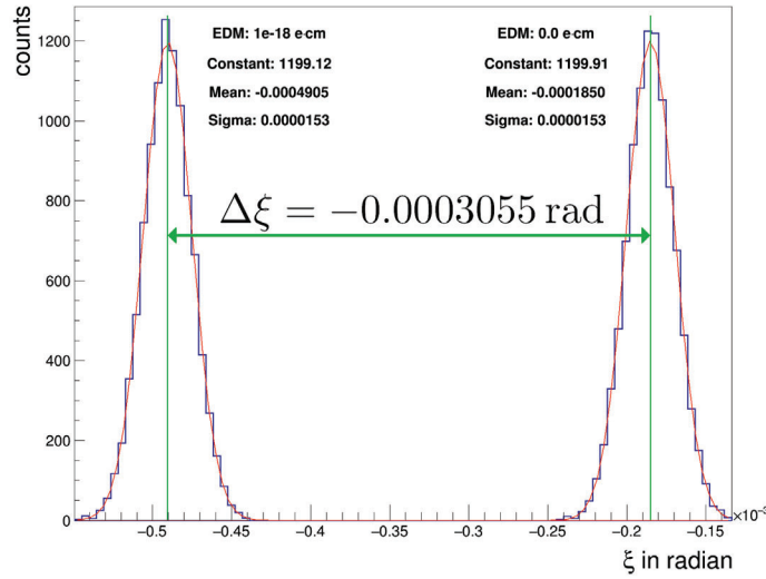
Figure 6.6: Distribution of tilt angles of the invariant spin axis in the y-x-plane for 10000 random Gaussian magnet misalignments. For the tracking calculations on the left, an EDM of 10^{-18} ecm was assumed. The distribution has the same shape and width as the one with a vanishing EDM (right). Only the mean value is shifted by the additional tilt angle described by Equation (4.53).
