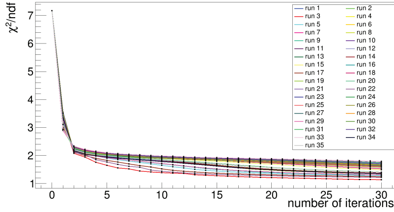
Figure 7.11: Different paths towards the global minimum of the minimization problem. Each path is the result of a different set of penalty weights.
