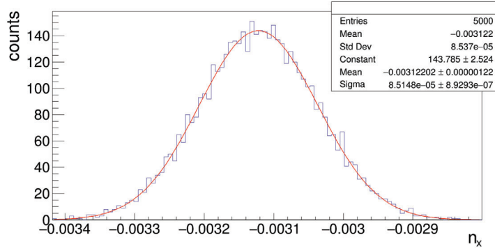
(a) Distribution of the horizontal component of the invariant spin axis.
