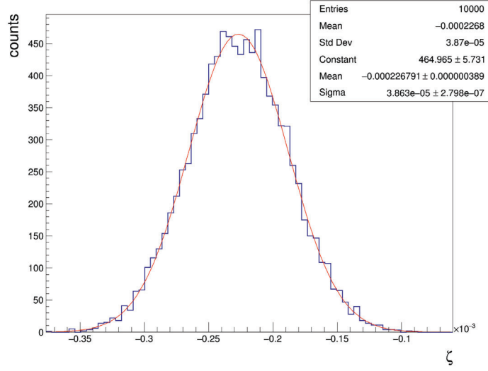
Figure 6.5: Distribution of tilt angles of the invariant spin axis in the y-s-plane for 10000 random Gaussian magnet misalignments. A Gaussian fit was performed to the data set.
