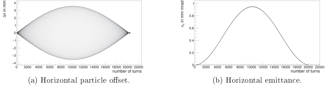
Figure 5.9: Tracking results of a deuteron with a momentum of 970 MeV/c and initial phase space coordinates on the closed orbit. The magnetic field of the Wien filter is reduced by 1 % compared to the default grid calculations. The horizontal betatron tune is changed to Q_x = 4 + \nu_S \approx 3.839 such that the Wien filter fields oscillate with a betatron sideband frequency. Therefore, the amplitude of the betatron oscillations adds up over time until the particle slips out of resonance.
