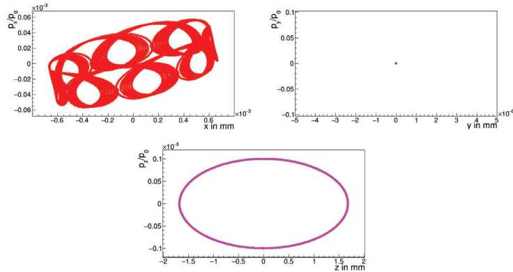
Figure A.2: Three-dimensional phase space of a particle with an initial longitudinal momentum offset of \frac{\Delta p_z}{p_0} = 10^{-4} at injection. While the vertical phase space is not affected, the horizontal motion is a superposition of betatron oscillations and dispersive effects.
