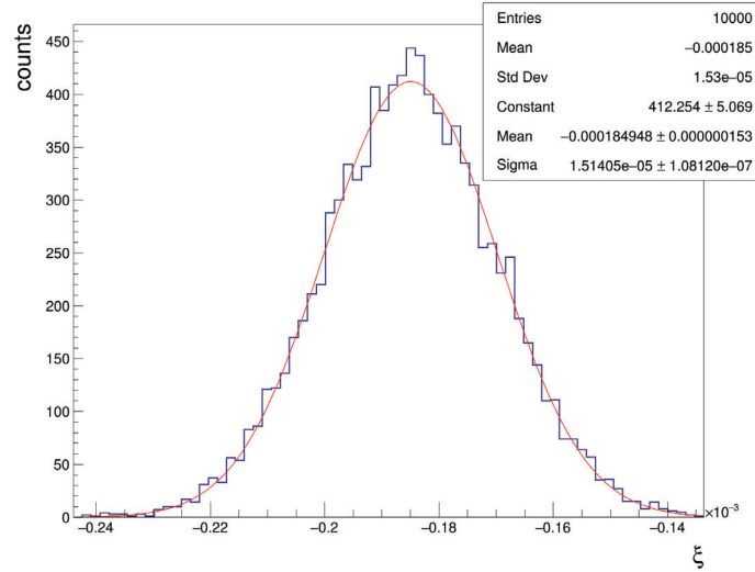
Figure 6.4: Distribution of tilt angles of the invariant spin axis in the y-x-plane for 10000 random Gaussian magnet misalignments. A Gaussian fit was performed to the data set. The mean value is equal to the tilt angle of the invariant spin axis when no random changes are applied and only the measured misalignments are taken into account. Note that the simulations are assuming a vanishing EDM ( \xi_{\text{EDM}} = 0 ).
