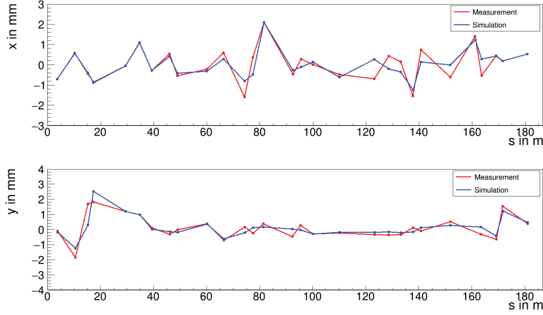
Figure 7.5: Simulated and measured orbits in horizontal and vertical direction. The simulation used the orbit matching algorithms over three iterations.
