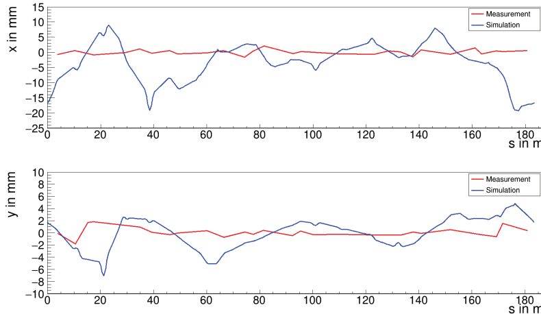
Figure 7.1: Simulated and measured orbit in horizontal and vertical direction. The simulation includes the changed effective length of dipoles and quadrupoles and the magnet misalignments from Section 6.1. The magnet settings (dipoles, quadrupoles, sextupoles and steerers) from the measurements in October 2019 were used for the simulation.
