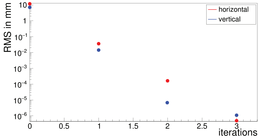
Figure 7.2: Closed orbit RMS values of the simulated orbits after each iteration of the orbit matching algorithm. The default simulation was initially distorted using randomly distributed steerer kicks. Afterwards, the algorithm step by step adjusts the steerer kicks so that the closed orbit becomes less and less distorted.
