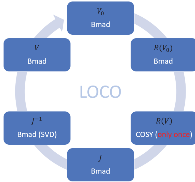
Figure 7.6: Working principle of the ORM analysis algorithm based on the LOCO method. All parts that are purely related to the simulation are marked with Bmad . The ORM has to be measured only once independently of the number of fitting iterations that are performed. After one cycle, the result of the current iteration is used to set the new machine parameter guess for the next iteration. Performing several iterations can lead to a better fit result since a single iteration cannot account for non-linear effects (adapted from [105]).
