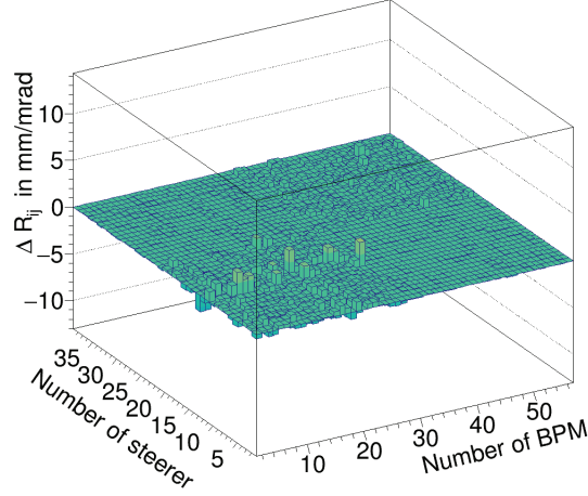
Figure 7.15: Final difference ORM after fitting the model using the LOCO algorithm as well as the orbit matching method.
