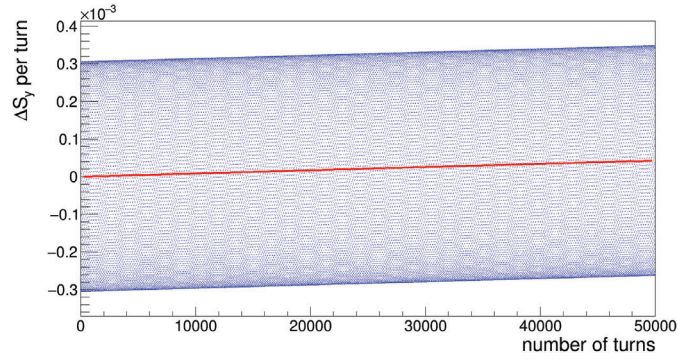
Figure 5.11: Tracking results for an initial spin along the momentum axes and an EDM of 10 \cdot 10^{-18} \text{ e cm} ( \eta_{\text{EDM}} = 1.902052 \cdot 10^{-4} ). The invariant spin axis is tilted according to Equation (4.53) and the vertical spin component therefore performs fast oscillations. Due to the electromagnetic fields of the RF Wien filter, a slow buildup of the average vertical spin component can be observed.
