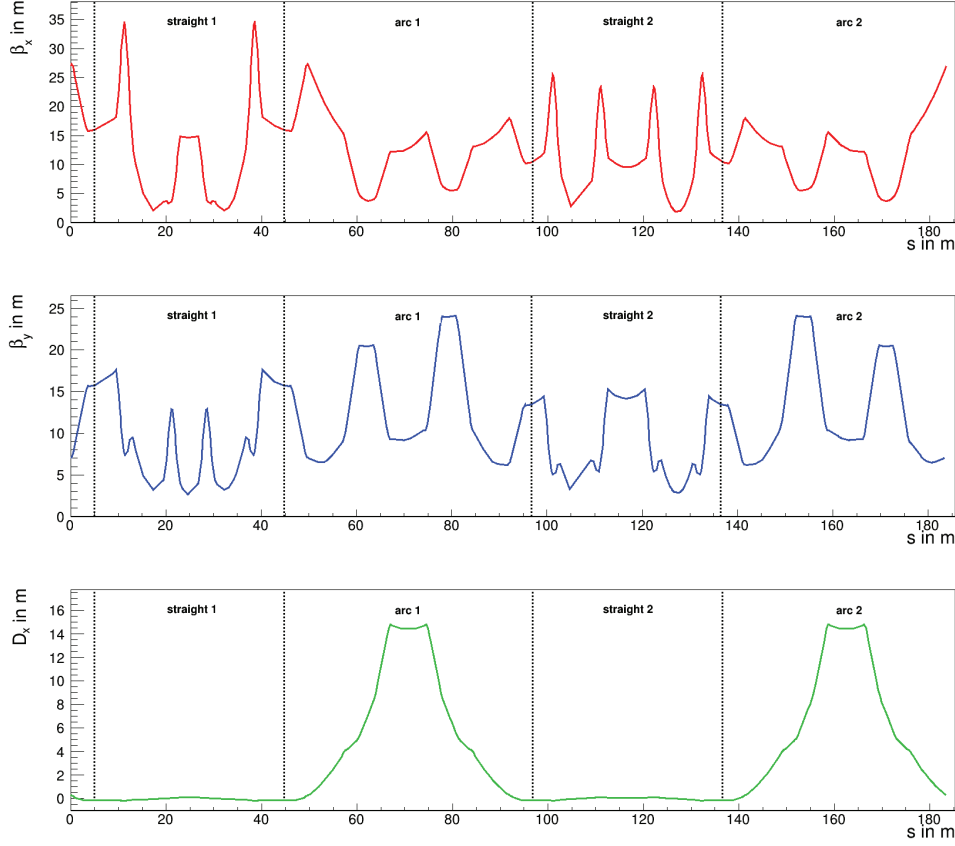
Figure 5.2: Optical functions \beta_x , \beta_y and D_x of the default lattice. The resulting dispersion in the straight sections is close to zero. Therefore, dispersive effects mainly appear in the arcs. The betatron tunes for the default lattice are Q_x = 3.62512 in horizontal direction and Q_y = 3.63061 in vertical direction.
