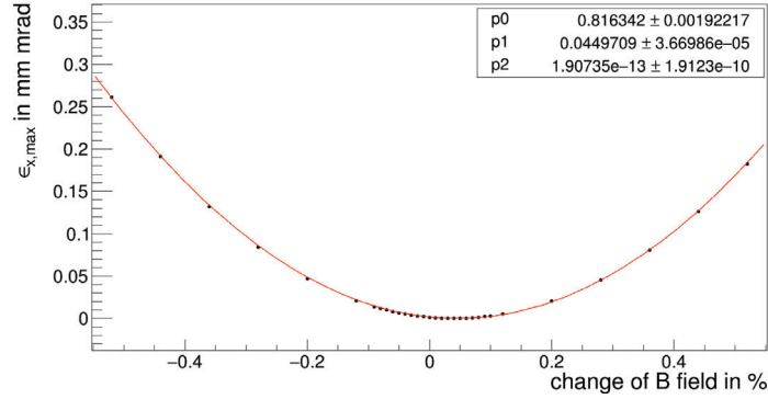
Figure 5.10: The maximum value of the horizontal emittance is shown as a function of the enhancement of the magnetic field inside the RF Wien filter. The electric field stays unchanged. A parabolic fit is performed in order to find the minimum emittance value and the corresponding scaling factor for the magnetic field. The minimum is reached for an increase of 0.045 %.
