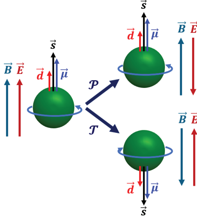
Figure 2.1: Schematic illustration of a particle in an external magnetic \vec{B} and electric \vec{E} field including a permanent EDM. Under a parity transformation ( \mathcal{P} ) the electric field changes its sign while the magnetic field and the spin stay unchanged. The time reversal transformation \mathcal{T} in contrast flips the MDM as well as the EDM and the magnetic field changes its sign. As a result, a system with a permanent EDM violates both symmetries and is according to the \mathcal{CPT} theorem also \mathcal{CP} violating (adopted from [21], Figure 2.1).
