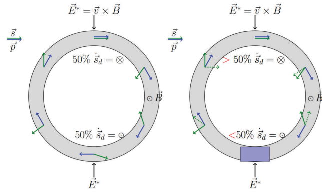
Figure 4.2: Schematic drawing of the RF Wien filter method. The RF Wien filter is represented by the blue box in the right sketch. Without an RF Wien filter (left), the spin points as often in direction of motion as it points in opposite direction. Therefore, the EDM signal fully averages to zero over time. The Wien filter (right) leads to an additional rotation of the spin around the vertical axis. As a result, the vertical polarization still oscillates but the signal does not completely vanish and a vertical polarization builds up over time [50].
