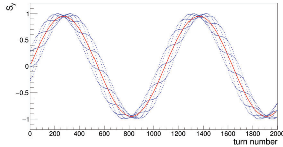
Figure 5.14: Tracking results using a field amplification factor of 10000 and an EDM value of 10 \cdot 10^{-15} ecm. The blue points correspond to the simulation results and the red line represents a sinusoidal fit to the data. A full slow oscillation is usually not detected within the experiment since the oscillation period is too long. The EDM measurement takes place in the very beginning of the vertical spin buildup where the behavior is almost linear.
