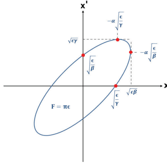
Figure 3.4: The phase space of a linear transverse particle motion is described by an ellipse with constant area, dependent on the Courant-Snyder invariant of the particle. Along the magnetic structure of the ring, the ellipse rotates in the coordinate system but its size and form stays unchanged. Adapted from [[37], [39]].
