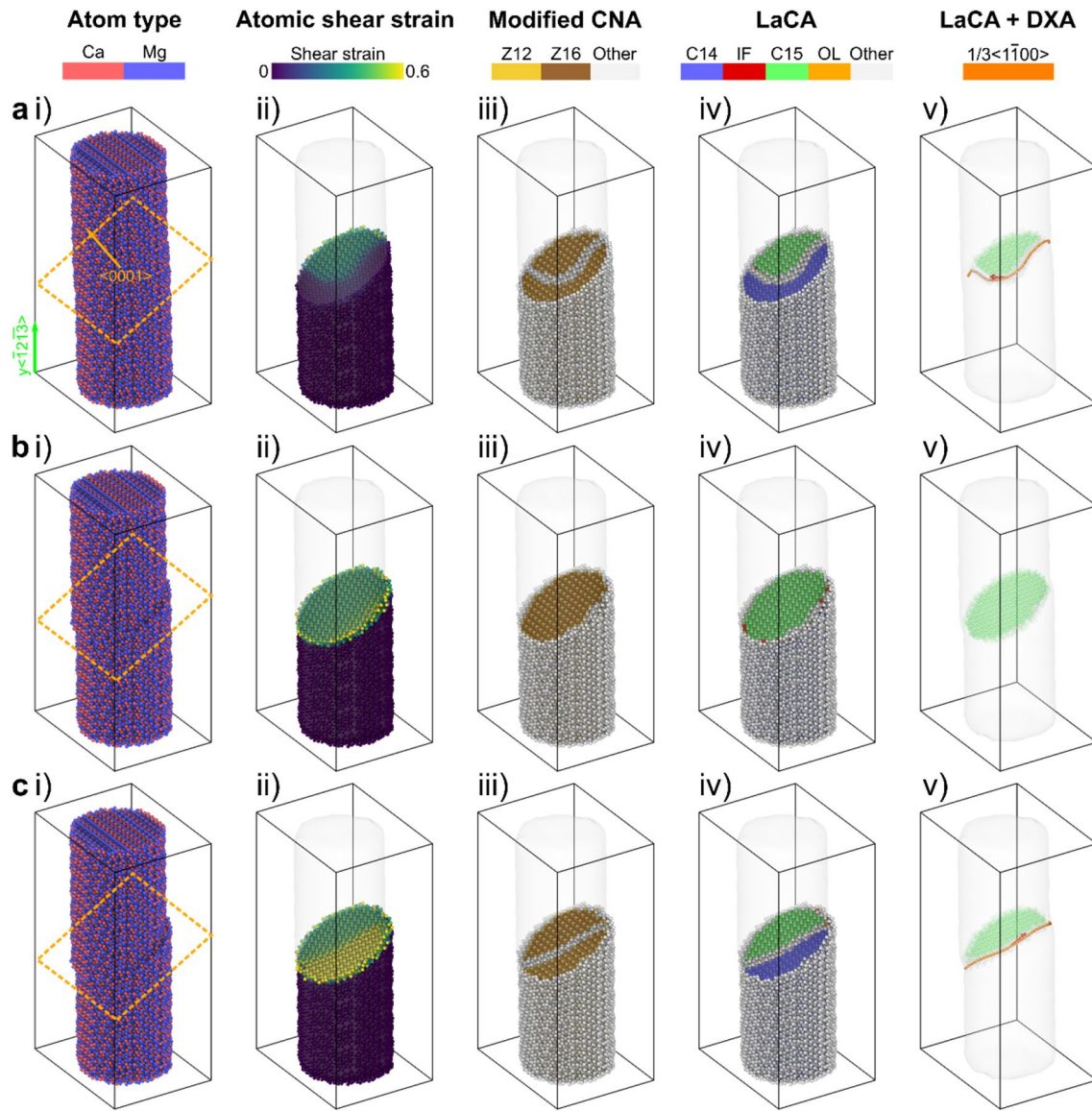
Figure 4: Synchroshear mechanism for basal slip in C14 \text{Mg}_2\text{Ca} Laves phase as computed by nudged-elastic band (NEB) method. (a) Glide of the leading synchro-Shockley dislocation. (b) Formation of a stacking fault (C15 Laves crystal structure) in the C14 Laves phase after the glide of the leading synchro-Shockley dislocation. (c) Glide of the trailing synchro-Shockley dislocation. (i) Colored by particle type, the dashed box indicates the slice along the basal plane in (ii)–(v). (ii) Colored by shear strain. (iii) Colored by the modified CNA. (iv) Colored by LaCA. (v) DXA was performed on the Laves phase crystal structures as identified by the modified CNA, by considering only the central atoms of the Z16 atomic clusters. Only atoms in stacking faults (C15 Laves crystal structure and Other) are shown in half-transparent. Burgers vector is colored red. The surface mesh of the pillar is shown in half-transparent.
