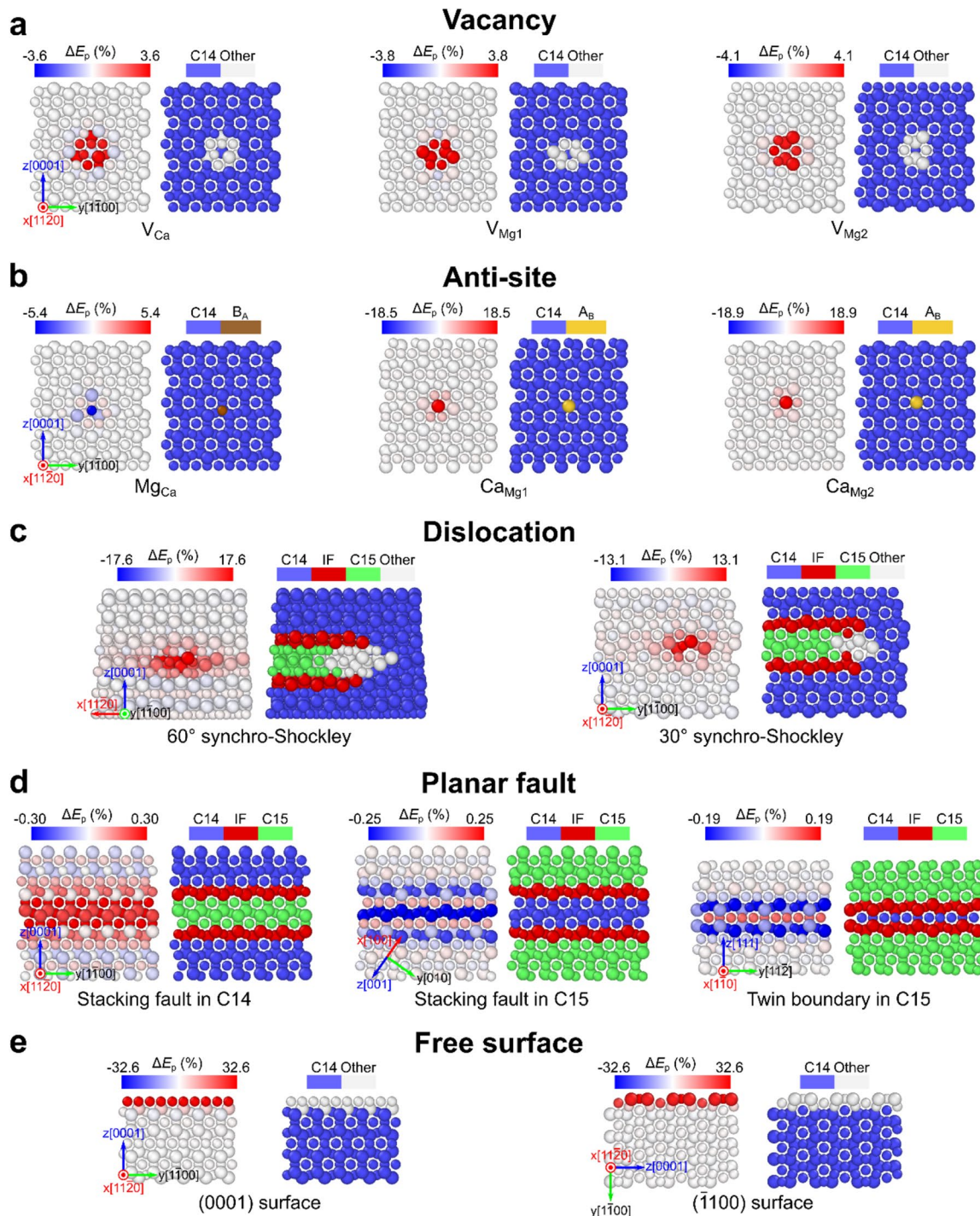
Figure 3: Overview of typical crystallographic defects in Laves phases. Left: colored by percentage deviation of potential energy to bulk ( \Delta E_p ). Right: colored by LaCA. Large and small atoms are A- and B-type atoms, respectively. The atomic size ratio is 1.231 for Mg–Ca systems. (a) Vacancy defects (denoted, e.g., as V_A for vacancy on an A site) in C14 Mg_2Ca . (b) Anti-site defects (denoted, e.g., as A_B for an A atom on a B site) in C14 Mg_2Ca . (c) Synchro-Shockley dislocations in C14 Mg_2Ca . (d) Stacking faults and twin boundary in C14 and C15 Mg_2Ca . (e) Free surfaces in C14 Mg_2Ca .
