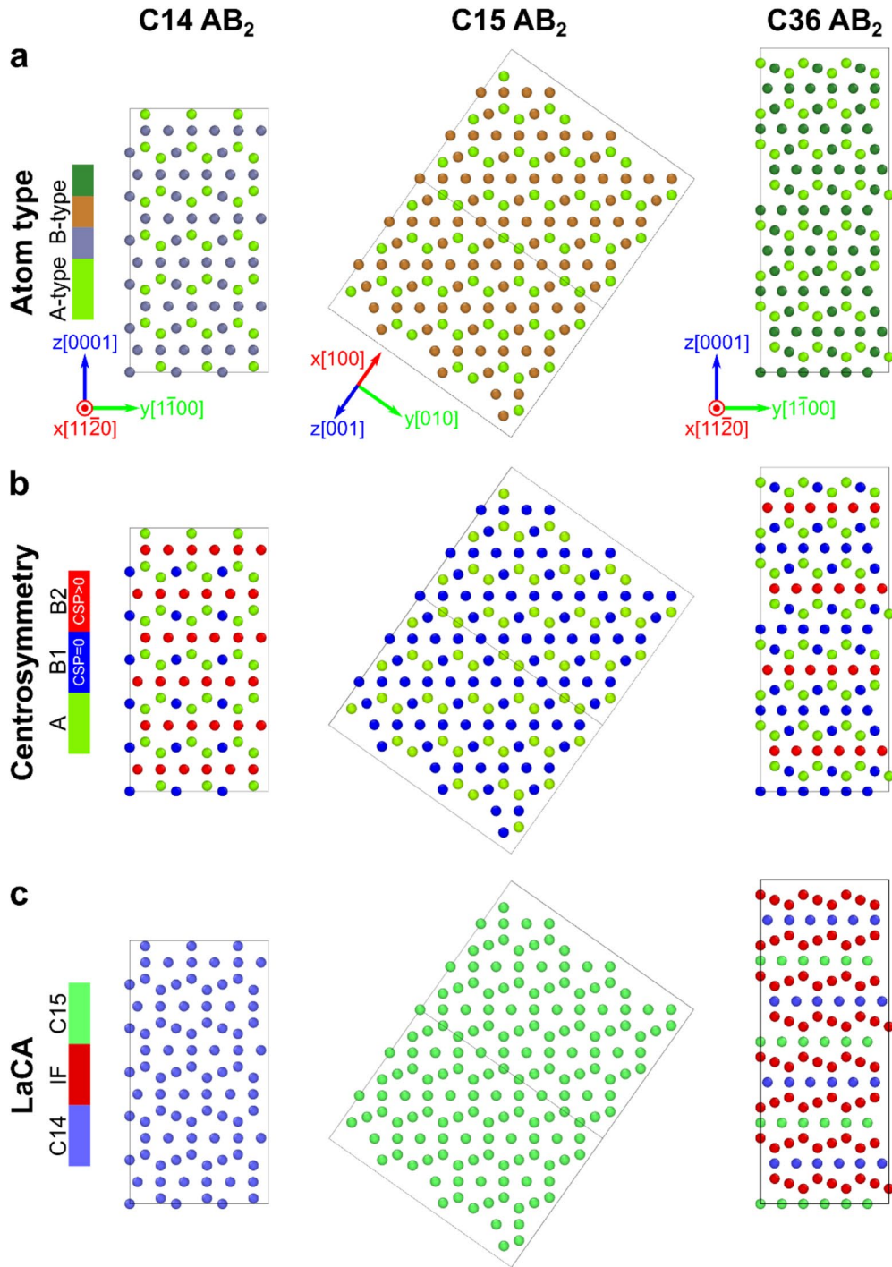
Figure 1: Laves phase crystal structures C14 ( 3 \times 3 \times 3 unit cells), C15 ( 3 \times 3 \times 3 unit cells) and C36 ( 3 \times 3 \times 2 unit cells). (a) Colored by particle type. A-type and B-type atoms are colored bright green and different subdued shades, respectively. (b) Colored by centrosymmetry parameter (CSP) which is calculated on the central atoms of Z12 Frank–Kasper (FK) clusters. B1-type and B2-type atoms are colored blue and red, respectively. (c) Colored by Laves phase crystal analysis (LaCA) method. Atoms in C14, interface (IF) between C14 and C15, and C15 Laves crystal structures are colored blue, red, and green, respectively.
