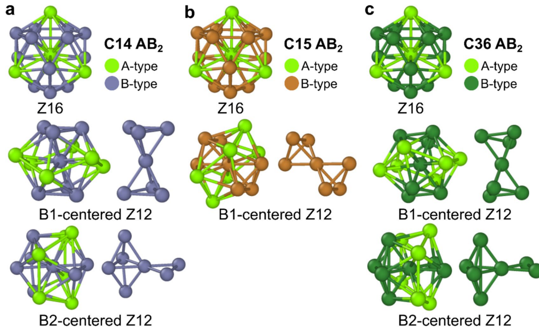
Figure 2: Characteristic atomic clusters in Laves phase crystal structures (a) C14, (b) C15 and (c) C36. B-type atoms in the Z12 icosahedral clusters are shown on the right side of the individual Z12 icosahedral clusters.
