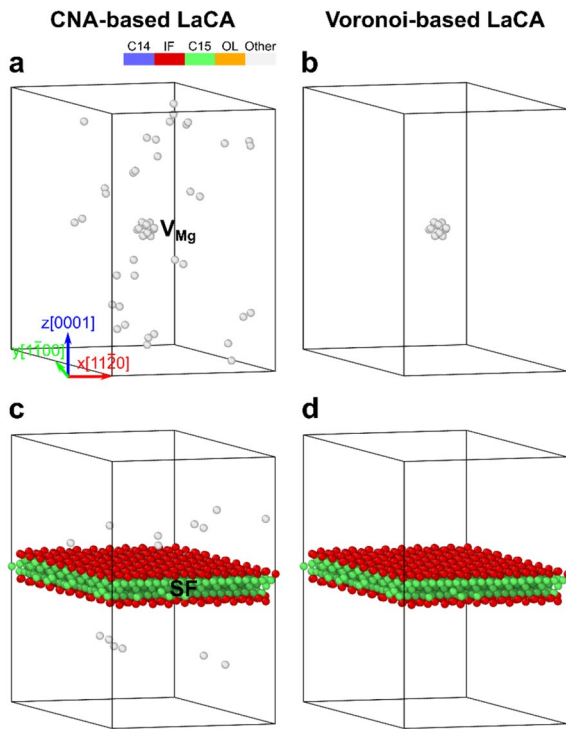
Figure 7: Defect structures of C14 Mg 2 Ca atomistic configurations with (a, b) a Mg vacancy and (c, d) a stacking fault at 500 K. Characteristic atomic clusters were identified using (a, c) the modified CNA and (b, d) the Voronoi index. Colored by LaCA.
