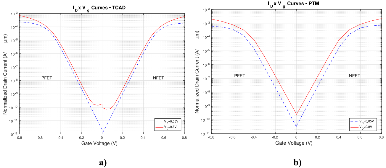
Fig. 4 Drain Current vs Gate Voltage for the transistors modeled in: a) TCAD, with physical parameter \times b) SPICE, with PTM
