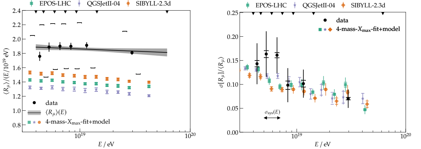
FIG. 7. Left panel: Average number of muons measured as a function of the energy together with the predictions from three interaction models given the composition measured with X_{\max} . The line is the best fit of the form \langle R_\mu \rangle(E) = a(E/10^{19} \text{ eV})^b . Right panel: Relative fluctuations in the number of muons measured as a function of the energy together with the predictions from three interaction models given the composition measured with X_{\max} .
