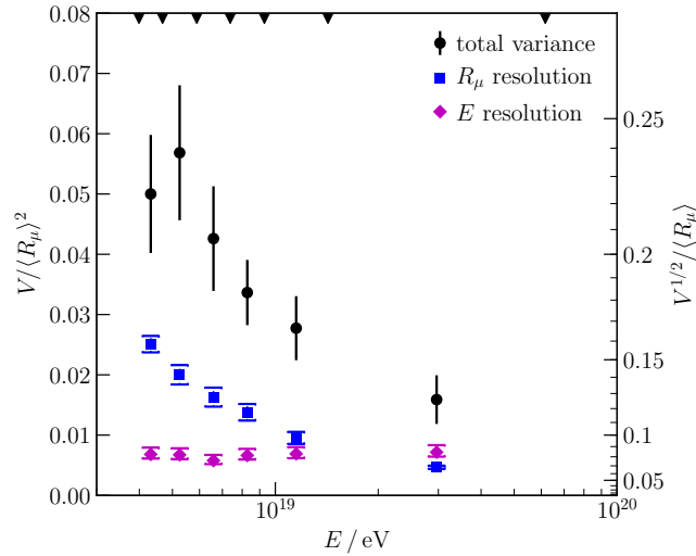
FIG. 5. Black points show the total relative fluctuations in R_\mu as a function of the shower energy (left axis for the variance and right axis for the standard deviation). Blue and pink points show the average relative resolution in R_\mu ( \langle s_\mu / R_\mu \rangle ) and E ( \langle s_E / E \rangle ) respectively. The error bars show the statistical uncertainty.
