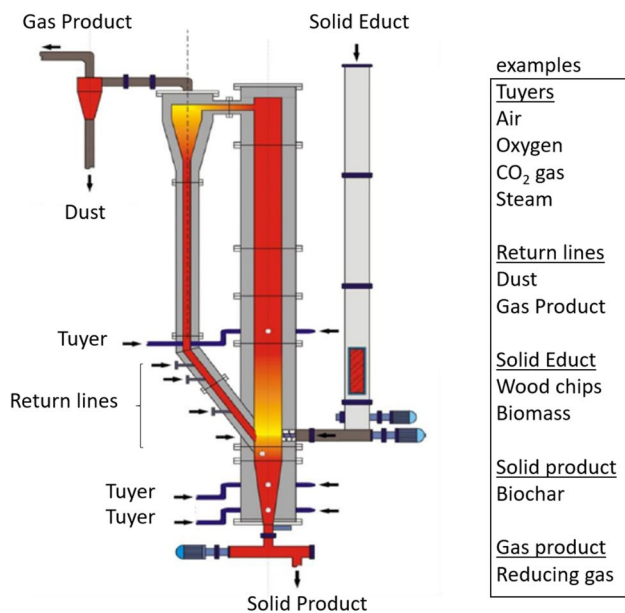
Fig. 15 Schematic of a high-temperature winkler process
