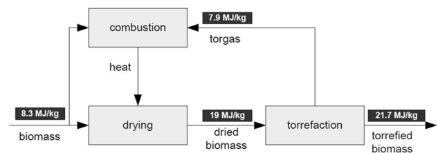
Fig. 14 Exemplary biomass drying and torrefaction process without the usage of recovered slag heat [21]
