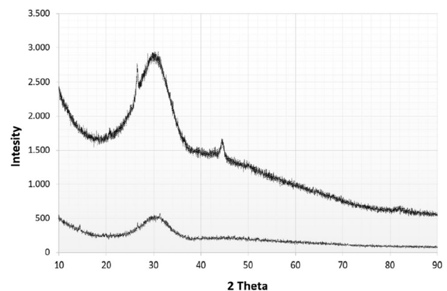
Fig. 8 X-ray diffraction pattern of two exemplary slag plates being > 0.950 g/g vitreous
