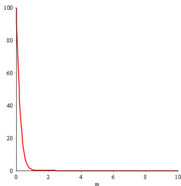
Figure 10. Function y^*(m, t) at t = 0.1 . The curve conditionally connects the values at discrete points.
