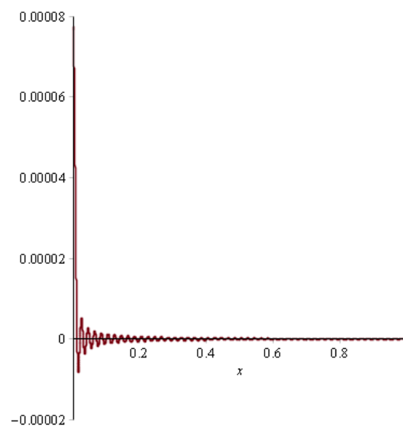
Figure 9. Function u^*(x) at h = 0.01 .
