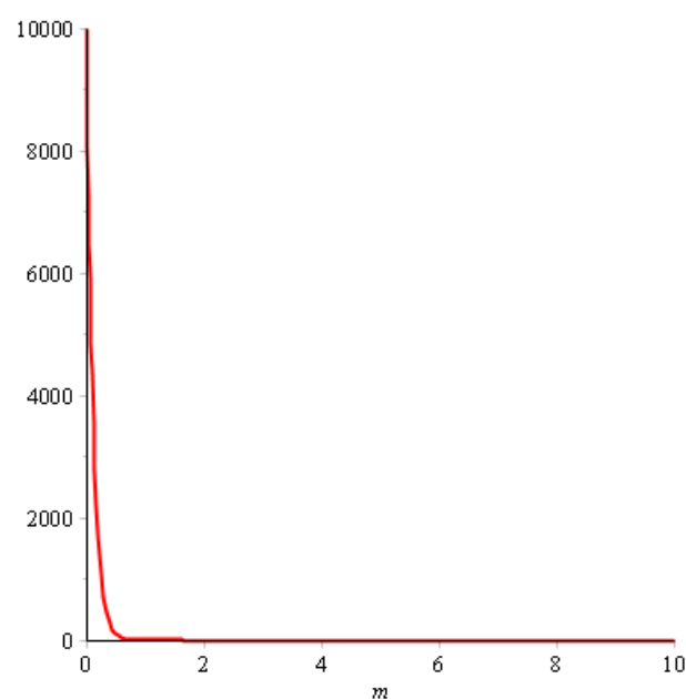
Figure 11. Function y^*(m, t) at t = 0.01 . The curve conditionally connects the values at discrete points.
