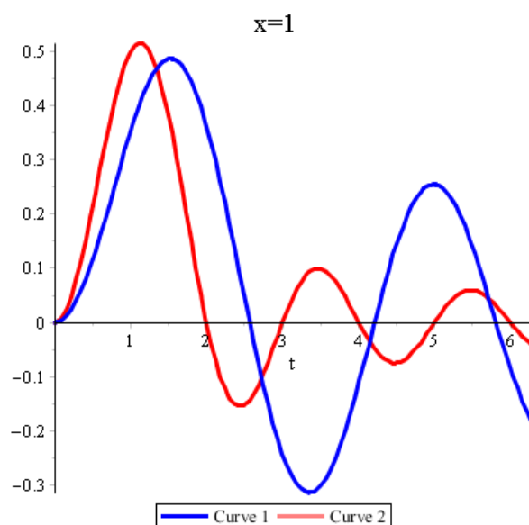
Figure 4. Comparison of continuous (12) (blue curve) and discrete (6) (red curve) solutions for x = mh , m = [1/h] ; [] denotes the integer part of the number. The red curve conditionally connects the values at discrete points.
