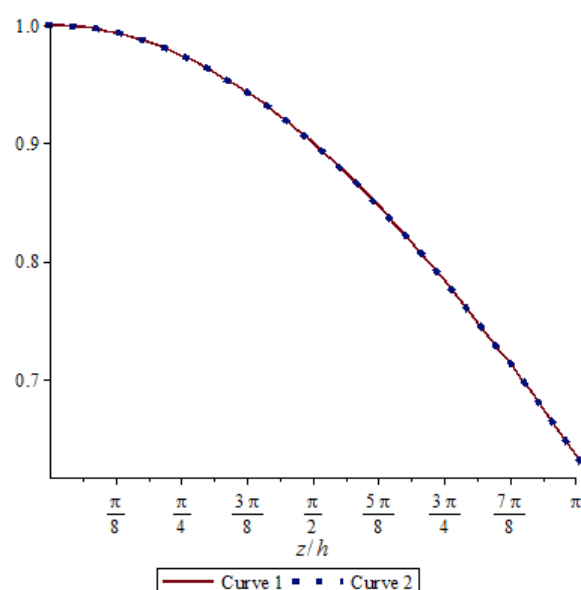
Figure 6. Comparison of phase velocities for continuous (13), (27) (curve 1) and discrete (2) (curve 2) models. The abscissa shows the values z/h ; the ordinates show the values V_{ph}/h . Curve 2 conditionally connects the values at discrete points.
