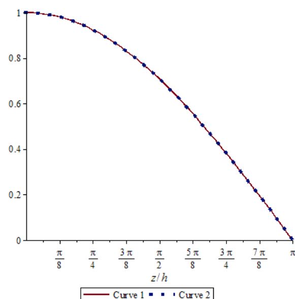
Figure 7. Comparison of group velocities for continuous (13), (27) (curve 1) and discrete (2) (curve 2) models. The abscissa shows the values z/h ; the ordinates show the values V_{gr}/h . Curve 2 conditionally connects the values at discrete points.
