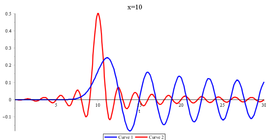
Figure 5. Comparison of continuous (12) (blue curve) and discrete (6) (red curve) solutions for x = m , m = [10/h] ; [] denotes the integer part of the number. The red curve conditionally connects the values at discrete points.
