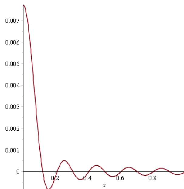
Figure 8. Function u^*(x) at h = 0.1 .
