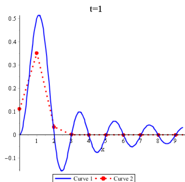
Figure 2. Comparison of continuous (12) (blue curve) and discrete (6) (red points) solutions for t = 1 .
