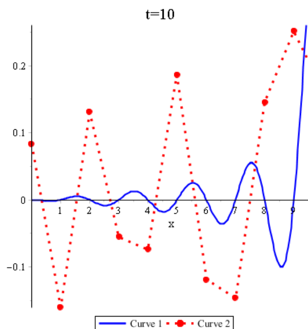
Figure 3. Comparison of continuous (12) (blue curve) and discrete (6) (red points) solutions f or t = 10 .
