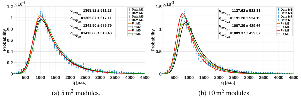
Figure 20: HG channel muon charge histograms for different modules. The data set corresponds to the period from May 2017 to December 2018.
