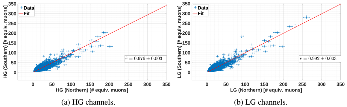
Figure 22: Comparison of the muons measured in the southern modules versus northern modules for the HG (a) and LG (b) channels. The red line represents a strait line fit of the ratio.
