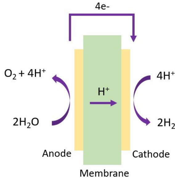
Figure 2.1 Schematic diagram of the working principle of PEM water electrolyzer.
