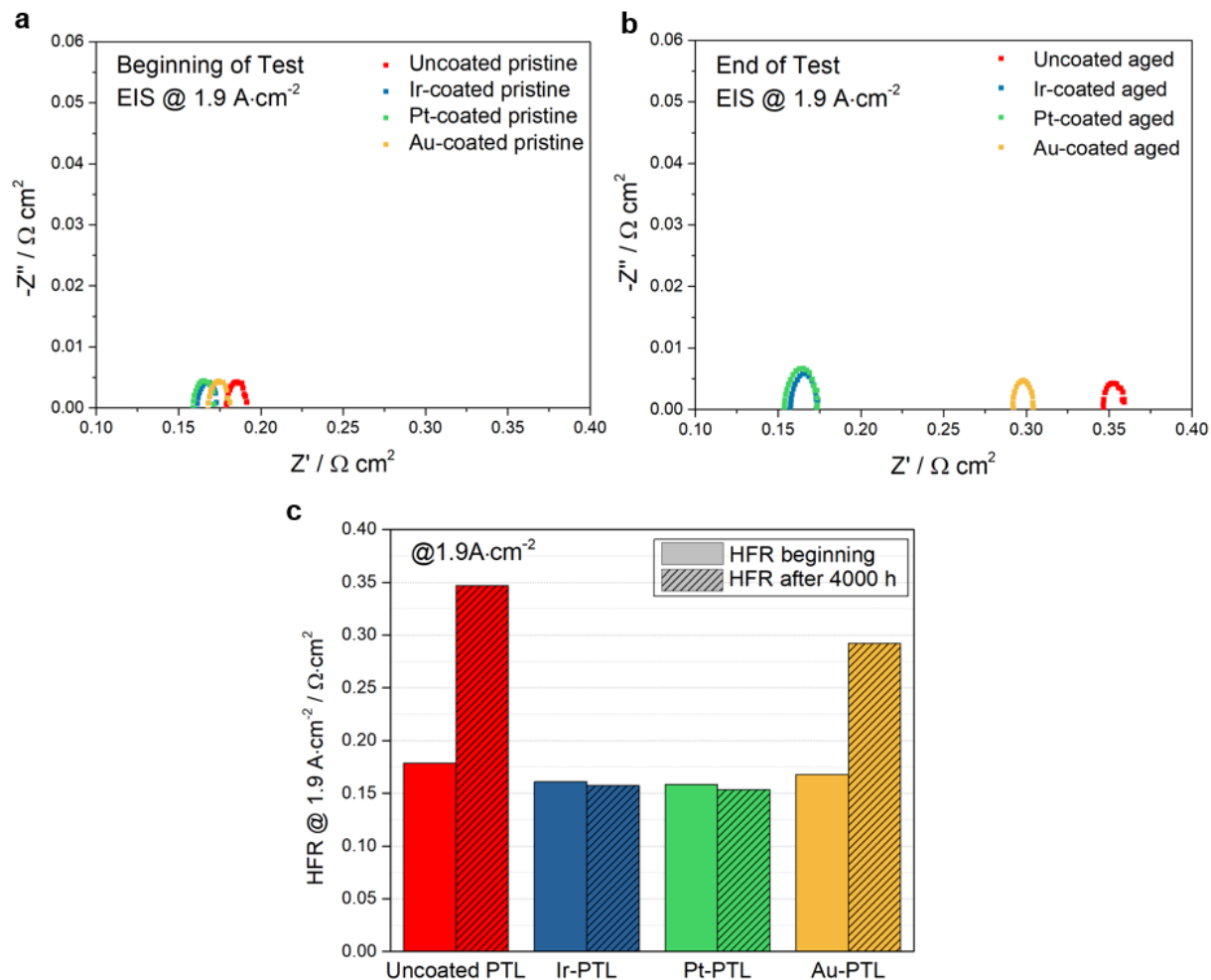
Figure 7.4 (a, b) EIS results at 1.9 \text{ A}\cdot\text{cm}^{-2} of Ir-coated, Pt-coated, Au-coated and uncoated PTLs; (c) HFR at 1.9 \text{ A}\cdot\text{cm}^{-2} of Ir-coated, Pt-coated, Au-coated and uncoated PTLs before and after 4000 hours of operation [28].
