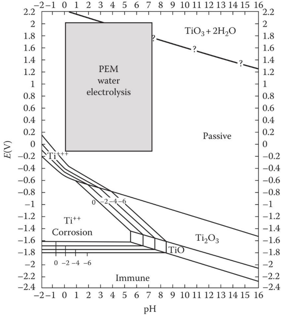
Figure 2.5 Pourbaix diagram of the titanium–water system [78].
