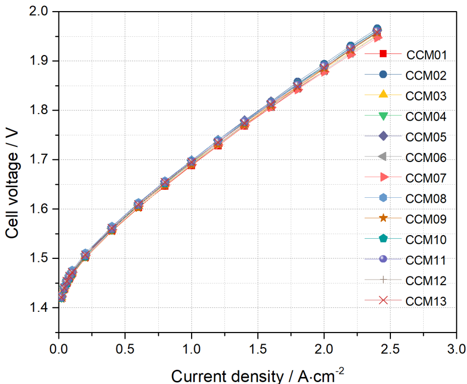
Figure 4.2 Polarization curves of PEM water electrolyzer single cells assembled with carbon papers and CCMs from the same batch. The cell temperature was 80^{\circ}\text{C} and under ambient pressure.
