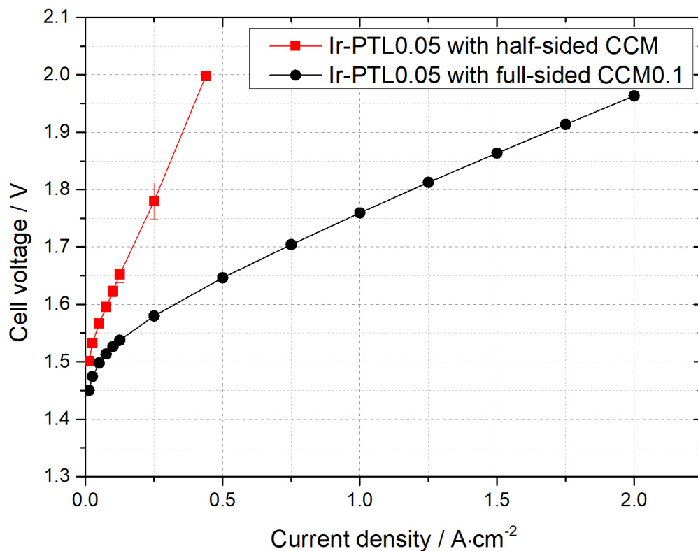
Figure 5.7 Polarization curves of PEM water electrolyzer single cells assembled with Ir-PTL0.05; one is with normal(full-sided) CCM containing 0.1 \text{ mg}\cdot\text{cm}^{-2} \text{IrO}_2 at anode and 0.8 \text{ mg}\cdot\text{cm}^{-2} Pt/C at cathode (black), the other one (referred to as half-sided CCM) is without \text{IrO}_2 at anode but just 0.8 \text{ mg}\cdot\text{cm}^{-2} Pt/C at the cathode (red).
