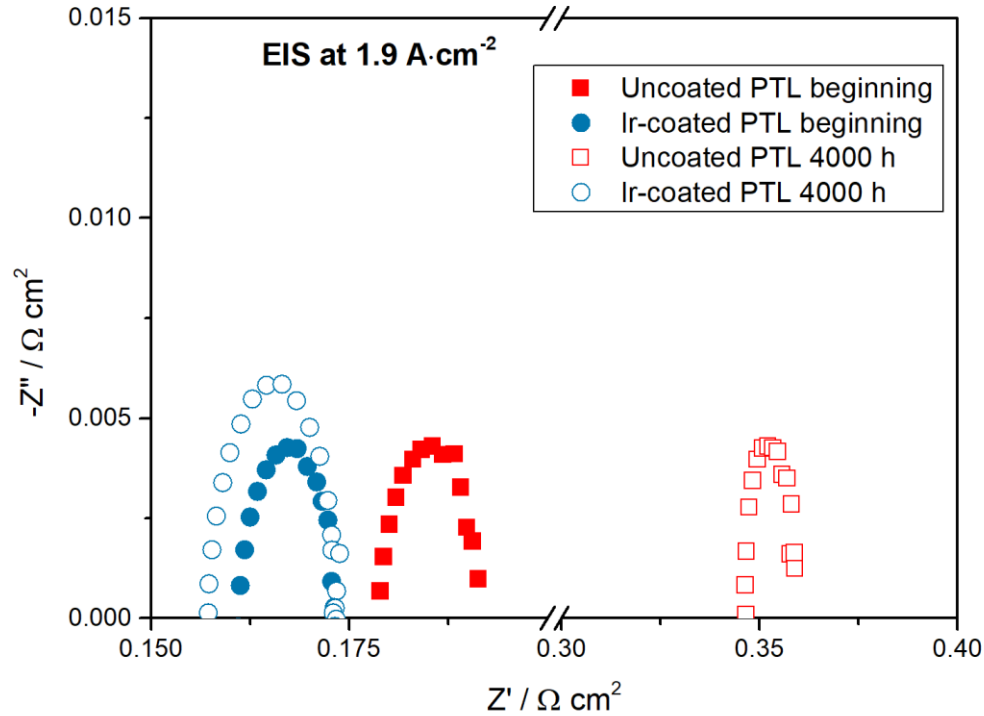
Figure 6.4 EIS results at 1.9 \text{ A} \cdot \text{cm}^{-2} .
