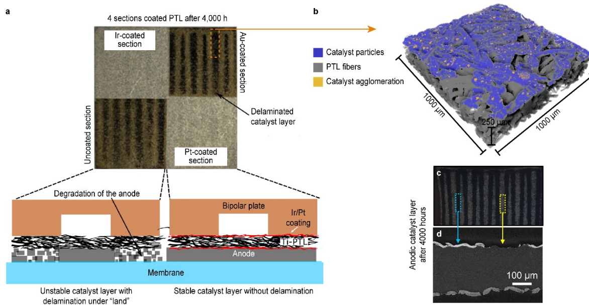
Figure 8.1 (a), Optical image of four sections of coated PTL after 4000 hours; (b), X-ray CT image of Au-coated section after 4000 hours (catalyst residuals are shown in blue, larger particles/ catalyst agglomeration in yellow); (c), optical image of aged CCM assembled with uncoated PTL; (d), cross-section SEM images of aged CCM assembled with uncoated PTL [28].
