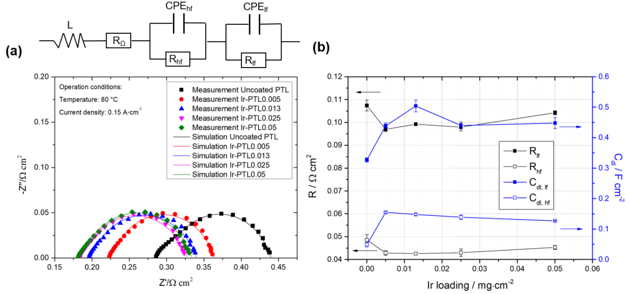
Figure 5.5 (a) EIS results at 0.15 A·cm -2 and equivalent circuit fitting; (b) Kinetic resistances, R_{hf}/R_{lf} , and double layer capacitances, C_{dl,hf}/C_{dl,lf} , obtained from the fits of the impedance spectra shown in Fig. 5.5a. The error bars show the individual fitting errors of each value [108].
