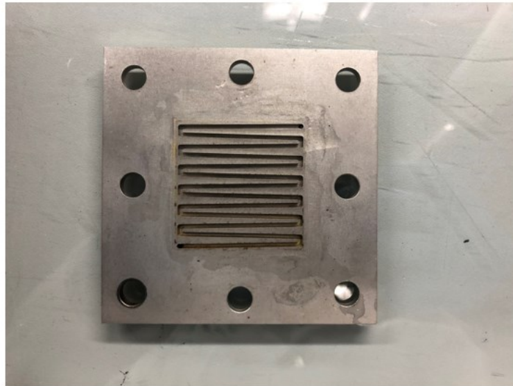
Figure 12.1 (a) Image of pin-type flow field used in chapter 4 and 5 (active area: 25 \text{ cm}^2 ); (b) Image of single serpentine type flow field used in chapter 6, 7 and 8 (active area: 17.64 \text{ cm}^2 ).
