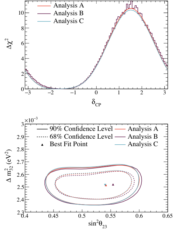
FIG. 47. Comparison between analyses A, B and C. The normal mass ordering is assumed and the reactor constraint is applied. Top: the predicted \Delta\chi^2 functions for \delta_{\text{CP}} . Bottom: the 1\sigma (dashed lines) and 90% (solid lines) C.L. regions for \Delta m^2 vs \sin^2 \theta_{23} .
