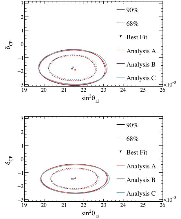
FIG. 57. Comparison between the observed 1\sigma (dashed lines) and 90% (solid lines) C.L. regions for \delta_{CP} vs \sin^2\theta_{13} produced using analyses A, B and C, assuming normal mass ordering (top) or inverted mass ordering (bottom). The reactor constraint is applied.
