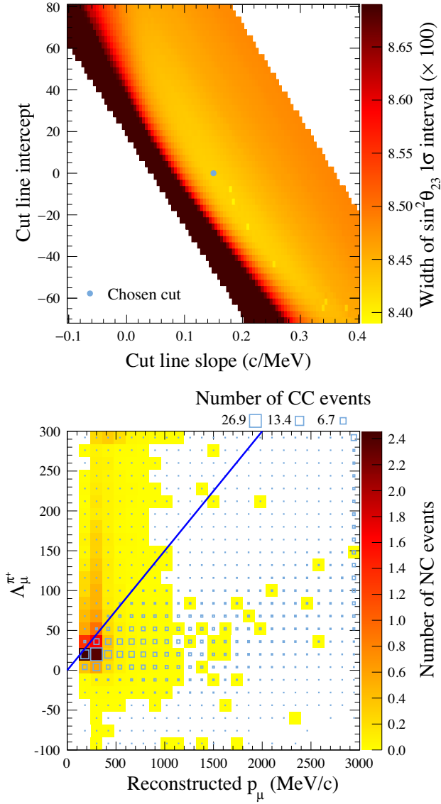
FIG. 28. The width of \sin^2 \theta_{23} 1\sigma confidence interval as a function of the slope and intercept of the \text{NC}\pi^+ rejection cut line is shown on the top and the distribution of signal (box histogram, axis on top of plot) and background events (colored histogram) is shown on the bottom, along with the line below which \mu -like events are selected.
