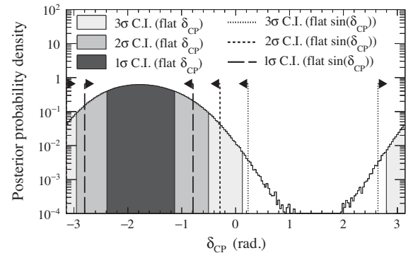
FIG. 61. Posterior probability density for \delta_{\text{CP}} and credible intervals obtained using a prior uniform in \delta_{\text{CP}} compared against credible intervals obtained with a prior uniform in \sin(\delta_{\text{CP}}) . The CP-conserving values are outside of the 2\sigma credible intervals in both cases.
