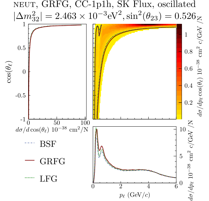
FIG. 7. The predicted flux-averaged cross section for three different nuclear response models. The different models result in different predictions of the observed final-state lepton kinematics for the same oscillated neutrino flux. If such variations are not accounted for in the uncertainty model, extracted oscillation parameters may be biased. The contours contain the region of phase space with a differential cross section d\sigma/dp_\ell \cos(\theta_\ell) > 0.05 \times 10^{-38} \text{ cm}^2 \text{ c / GeV / N} .
