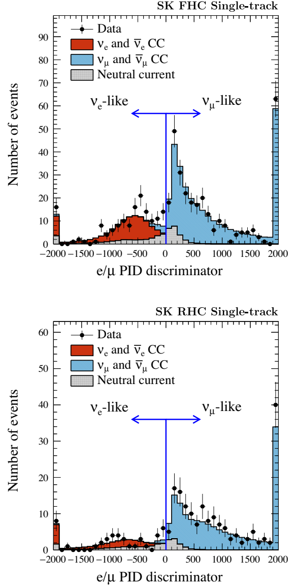
FIG. 17. Distribution of the e/\mu PID discriminator for single-track events passing the wall > 80 cm and towall > 170 cm FV criteria in FHC (top) and RHC (bottom) data.
