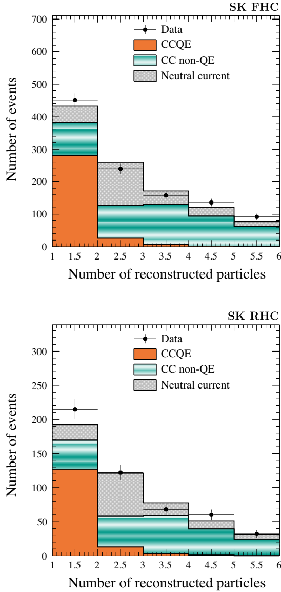
FIG. 16. Distribution of number of reconstructed particle tracks for events passing the wall > 80 cm and towall > 170 cm FV criteria in FHC (top) and RHC (bottom) data.
