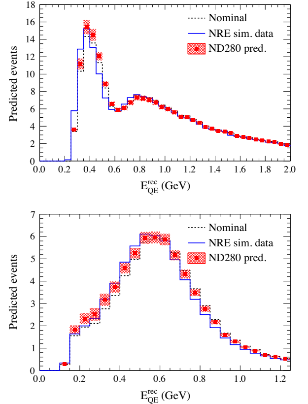
FIG. 51. Comparison of the nominal MC prediction (dashed black line), simulated data (solid blue line) and prediction from the near detector fit to the simulated data (shaded red). This is shown for the far detector muonlike (top) and electronlike (bottom) neutrino beam event samples.
