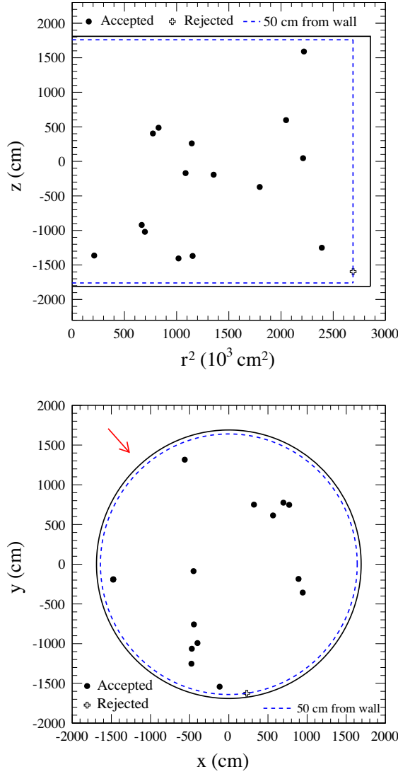
FIG. 24. Reconstructed vertices of selected FHC data 1R_e + 1 \text{ d.e.} events projected in z vs r^2 (top) and y vs x (bottom). The neutrino beam direction is shown as a red arrow and events which do not pass the fiducial volume criteria are shown as hollow crosses.
