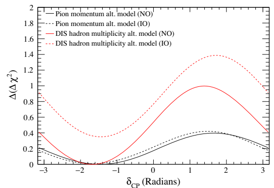
FIG. 68. Change in the \Delta\chi^2 function for \delta_{CP} when fitting data using an alternative model for DIS hadron multiplicity (red curves) and pion momentum spectra (black curves). The \Delta\chi^2 was reduced by the value shown on the plot in each case. The difference is shown for the model change that gave the largest difference in each case.
