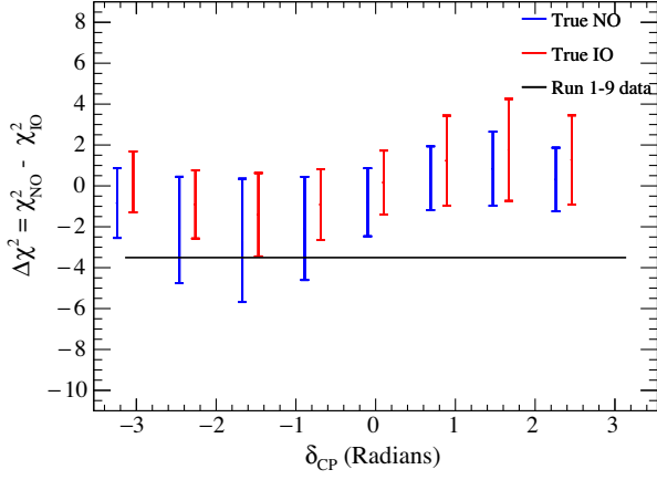
FIG. 70. Ability to distinguish between the two mass orderings as a function of the true value of \delta_{CP} . The bar indicates the range of values of \Delta\chi^2 = \chi^2_{NO} - \chi^2_{IO} which contains 95% of the values obtained for the pseudoexperiments generated in each case. The black line corresponds to the value obtained in the data fit by analysis A.
