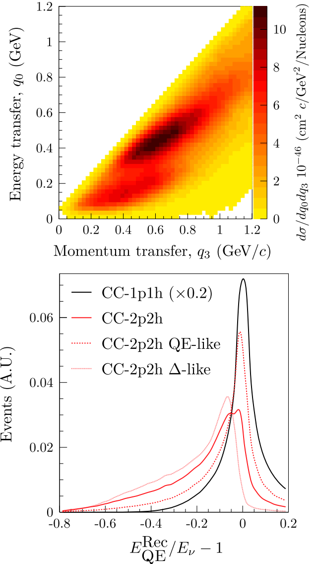
FIG. 4. Top: the energy and momentum transfer distribution for the Nieves et al. 2p2h model in NEUT. The two-peak structure is clear, with QE-like kinematics corresponding to the lower left peak and Delta-like kinematics to the stronger central peak. Bottom: the reconstructed energy bias at SK is shown for 1p1h and 2p2h events for an oscillated muon neutrino flux. The different reconstructed energy smearing for 2p2h events with QE-like and Delta-like interaction kinematics can be seen.
