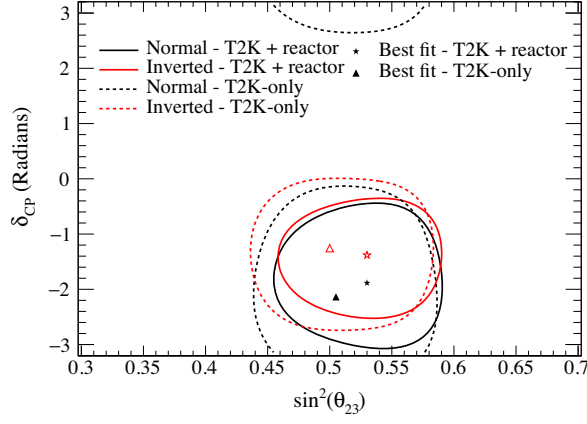
FIG. 55. The observed constant \Delta\chi^2 90% confidence regions of \sin^2\theta_{23} and \delta_{CP} with normal and inverted mass orderings and with and without the reactor constraint. Normal and inverted mass ordering contours are independent. \Delta\chi^2 values are calculated independently for the functions with and without the reactor constraint.
