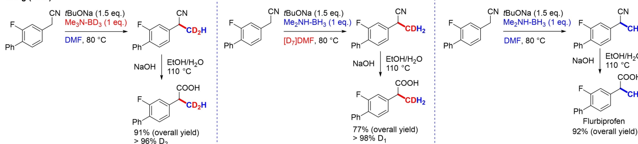
Scheme 31. Preparation of CD 2 H/CDH 2 /CH 3 flurbiprofen precursors by \alpha -trideuteromethylation of arylacetonitriles.
