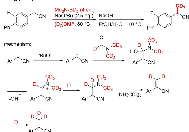
Scheme 30. Preparation of the CD 3 -flurbiprofen precursor by \alpha -trideuteromethylation of aryl acetonitriles.
