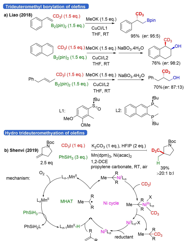
Scheme 13. Trideuteromethyl functionalization of alkenes with CD 3 I.
