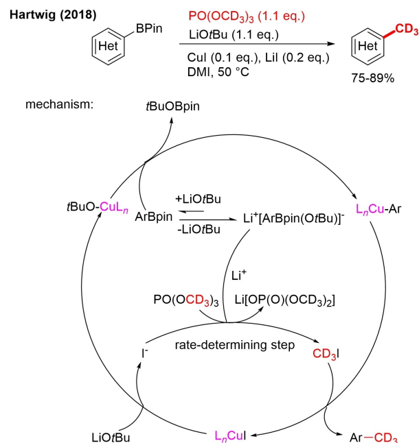
Scheme 25. Trideuteromethylation (hetero)arylboronic ester with \text{PO}(\text{OCD}_3)_3 .
