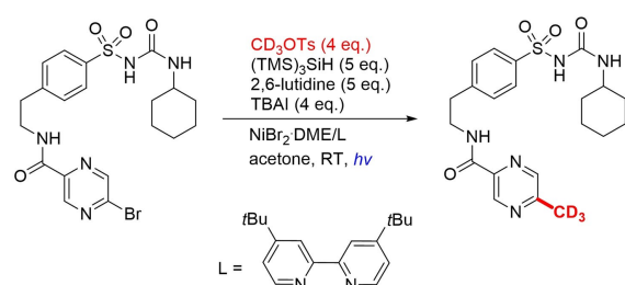
Scheme 22. Trideuteromethylation of \text{ArX} with \text{CD}_3\text{OTs} by reductive cross-coupling a) using \text{Co/Ni} dual catalysis and b) under photoredox conditions.
