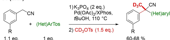
Scheme 24. Trideuteromethylation with \text{CD}_3\text{OTs} in multicomponent reactions.
