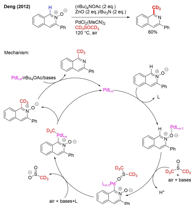
Scheme 15. Pd-catalyzed conversion of isoquinoline N-oxides to 1- \text{CD}_3 -isoquinolines in [\text{D}_6]\text{DMSO} .
