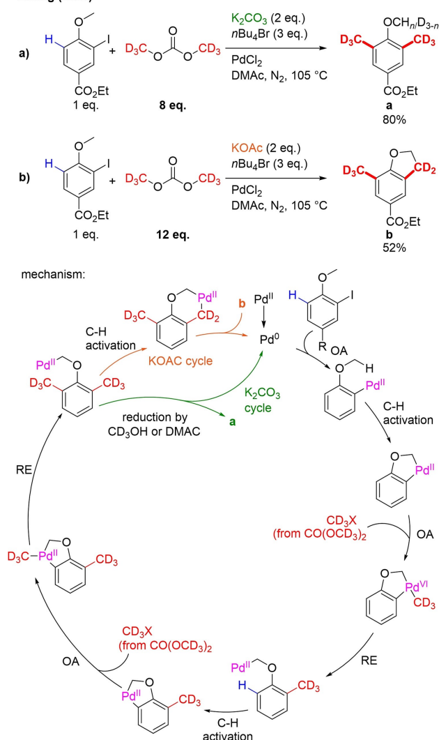
Scheme 36. - Site-selective di-trideuteromethylation of ortho -substituted iodoarenes.
