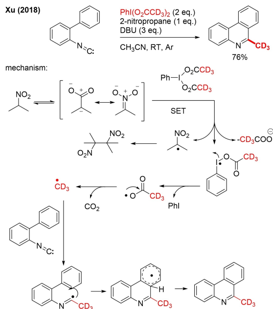
Scheme 37. 6-CD 3 -phenanthridine preparation by radical trideuteromethylation of biphenylisocyanide with PhI(O 2 CCD 3 ) 2 as trideuteromethyl radical source.
