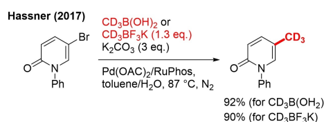
Scheme 27. Noncryogenic route towards 5- \text{CD}_3 pirfenidone.
