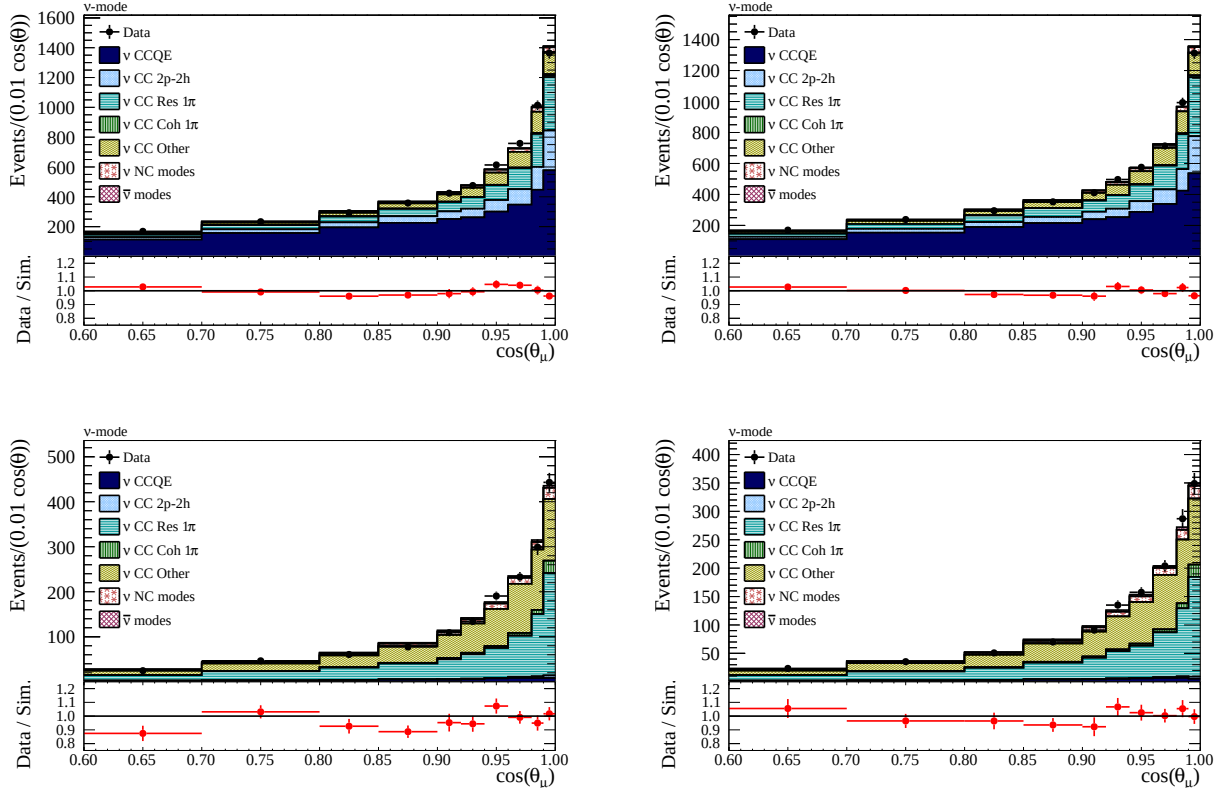
FIG. 38: Post ND280 fit distributions of the final state muon angle of the FHC \nu_\mu CC 0\pi (top), and FHC \nu_\mu CC 1\pi (bottom) samples in FGD1 (left) and FGD2 (right).
