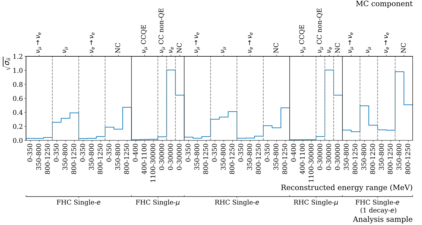
FIG. 33: Square root of the diagonal elements of the covariance matrix describing the systematic uncertainty associated to the modeling of the SK detector.
