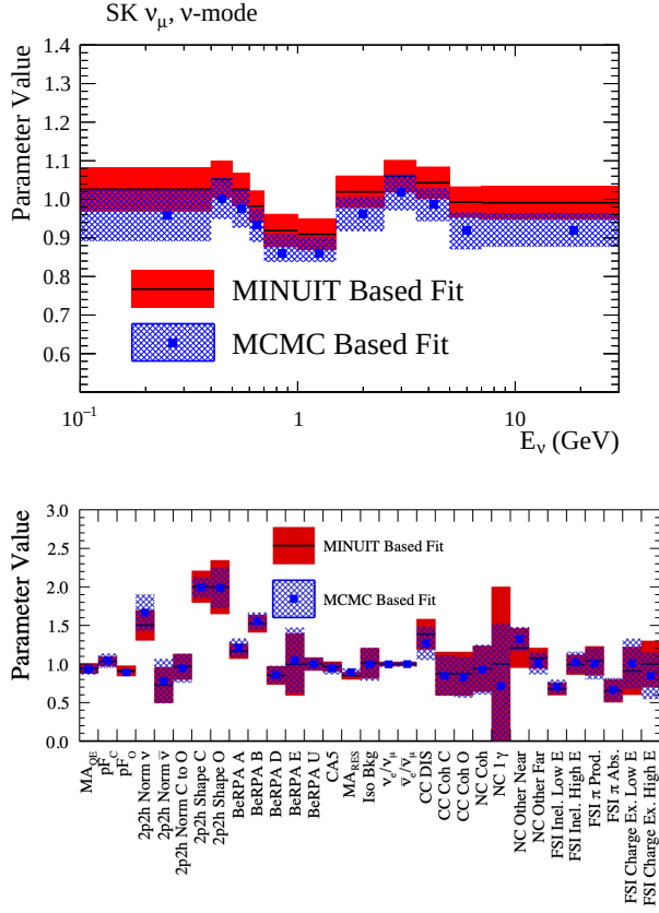
FIG. 43: Comparisons of the fitted SK FHC flux parameters (top) and cross-section parameters (bottom) between the ND280 fit (red, solid) and the MCMC analysis (blue, hashed).
