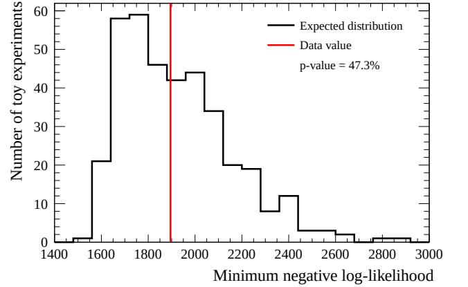
FIG. 36: Distribution of the minimum negative log-likelihood values from fits to the mock data sets (black), with the value from the fit to the data superimposed in red. The p -value is 47.3%.
