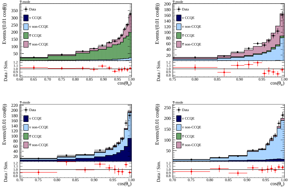
FIG. 40: Post ND280 fit distributions of the final state muon angle for the RHC \bar{\nu}_\mu (top) and \nu_\mu (bottom) CC 1-track (left) and CC N -track (right) FGD1 samples.
