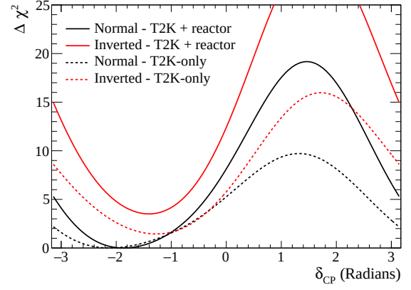
FIG. 54: The observed \Delta\chi^2 function of \delta_{CP} , with and without the reactor constraint. The \Delta\chi^2 is computed with respect to the best fit over the two mass orderings, and separate best fit points are used for the T2K-only and the T2K+reactor cases.
