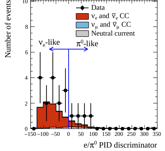
FIG. 20: Distribution of the e/\pi^0 PID discriminator for 1R_e + 1 d.e. in FHC data.
