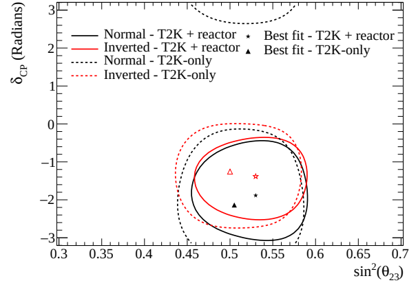
FIG. 55: The observed constant \Delta\chi^2 90% confidence regions of \sin^2 \theta_{23} and \delta_{CP} with normal and inverted mass orderings and with and without the reactor constraint. Normal and inverted mass ordering contours are independent. \Delta\chi^2 values are calculated independently for the functions with and without the reactor constraint.
