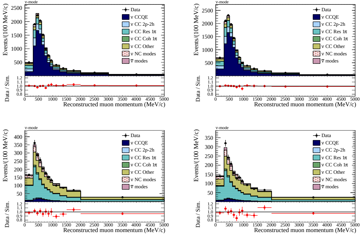
FIG. 37: Post ND280 fit muon momentum distributions of the FHC \nu_\mu CC 0\pi (top), and FHC \nu_\mu CC 1\pi (bottom) samples in FGD1 (left) and FGD2 (right).
