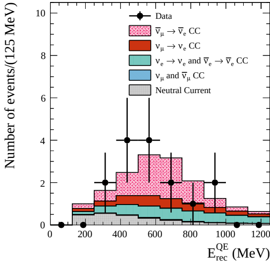
FIG. 25: Reconstructed energy distribution for 1R_e events in FHC (top) and RHC (bottom) data.
