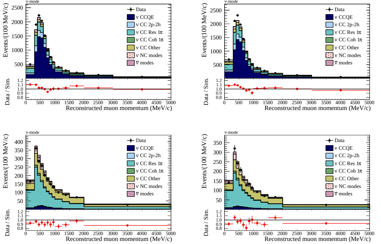
FIG. 11: Final state muon momentum distributions of the FHC \nu_\mu CC 0\pi (top) and \nu_\mu CC 1\pi^+ (bottom) data and simulation samples in FGD1 (left) and FGD2 (right).
