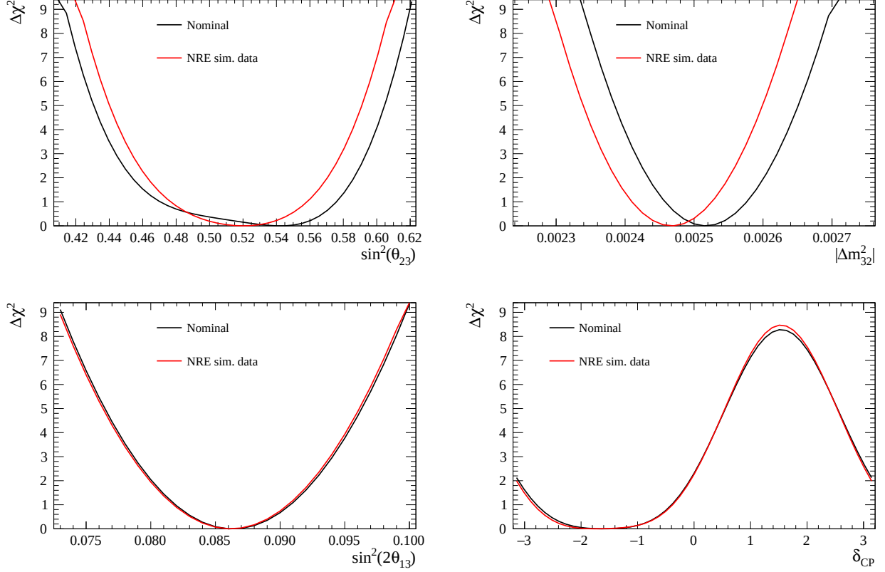
FIG. 52: Comparison of the nominal MC oscillation parameter \Delta\chi^2 function (black) to those from the simulated data fits (red).
