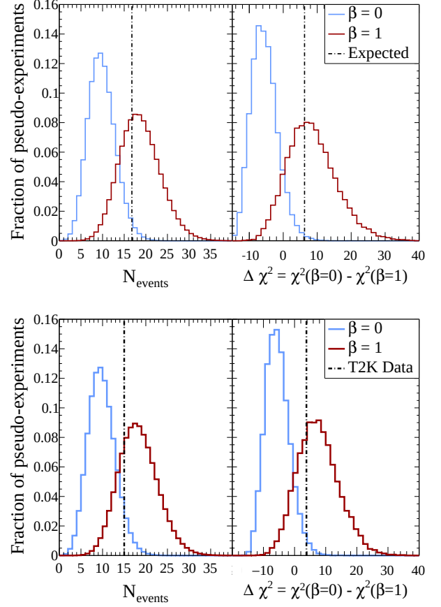
FIG. 73: Distributions of the expected (top) and observed (bottom) rate-only (left) and rate+shape (right) test statistics compared to the expected/observed test statistics. Here N_{\text{events}} denotes the number of observed events in the RHC single-ring e -like sample.
