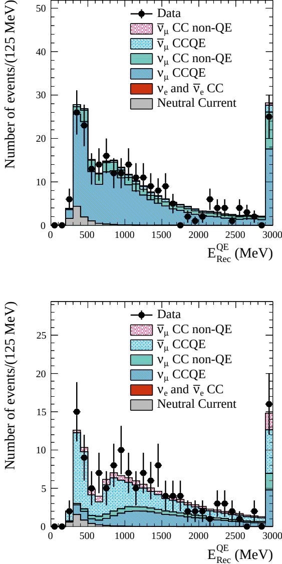
FIG. 27: Reconstructed energy distribution for 1R_\mu events in FHC (top) and RHC (bottom) data.
