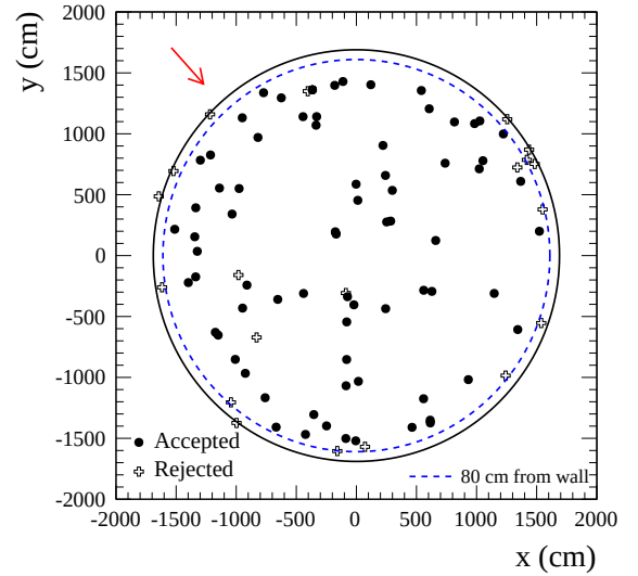
FIG. 22: Reconstructed vertices of selected FHC data 1R_e events projected in z vs r^2 (top) and y vs x (bottom). The neutrino beam direction is shown as a red arrow and events which do not pass the fiducial volume criteria are shown as hollow crosses.
