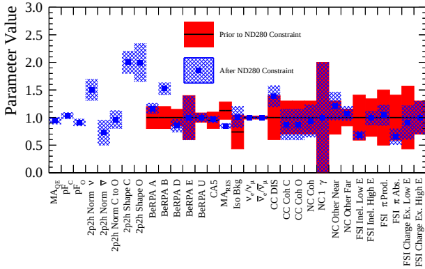
FIG. 35: The cross-section parameters as a fraction of the nominal value. The bands indicate the 1\sigma uncertainty on the parameters before (solid, red) and after (hatched, blue) the near detector fit.
