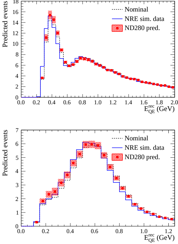
FIG. 51: Comparison of the nominal MC prediction (dashed black), simulated data (solid blue) and prediction from the near detector fit (shaded red), for the far detector muon-like (top) and electron-like (bottom) neutrino beam event samples.
