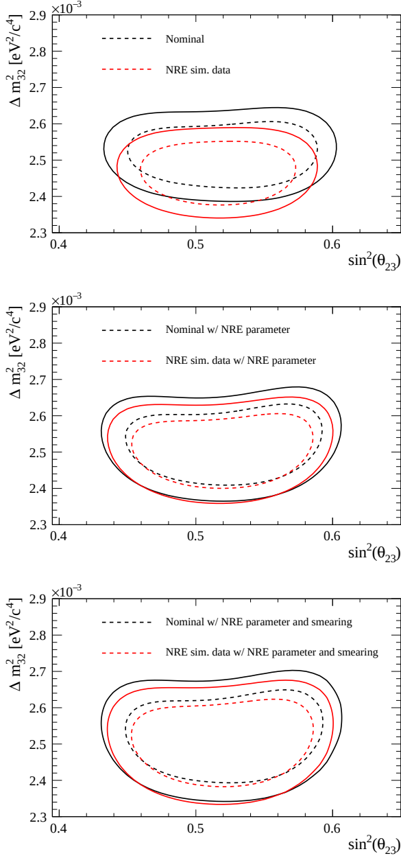
FIG. 53: Comparison of the \sin^2 \theta_{23} - \Delta m_{32}^2 parameter contours using the nominal cross-section model (top), after the addition of the ‘effective NRE’ parameter (middle) and after the additional smearing is applied to \Delta m_{32}^2 (bottom). In all cases the expected result, as described in the text, is shown in black and the simulated data result is in red. The solid lines represent the 90% confidence region and the dashed lines represent the 1\sigma confidence region.
