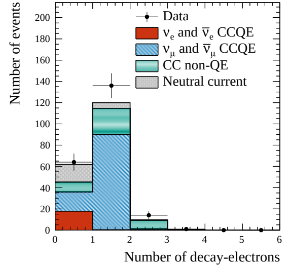
FIG. 18: Distribution of the number of identified decay-electrons for single-particle events passing the wall > 80 cm and towall > 170 cm FV criteria in FHC (top) and RHC (bottom) data.
