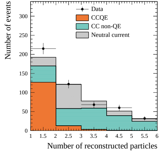
FIG. 16: Distribution of number of reconstructed particles for events passing the wall > 80 cm and towall > 170 cm FV criteria in FHC (top) and RHC (bottom) data.
