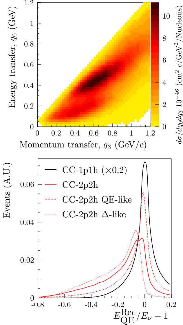
FIG. 4: Top: The energy and momentum transfer distribution for the Nieves et al. 2p2h model in NEUT.
