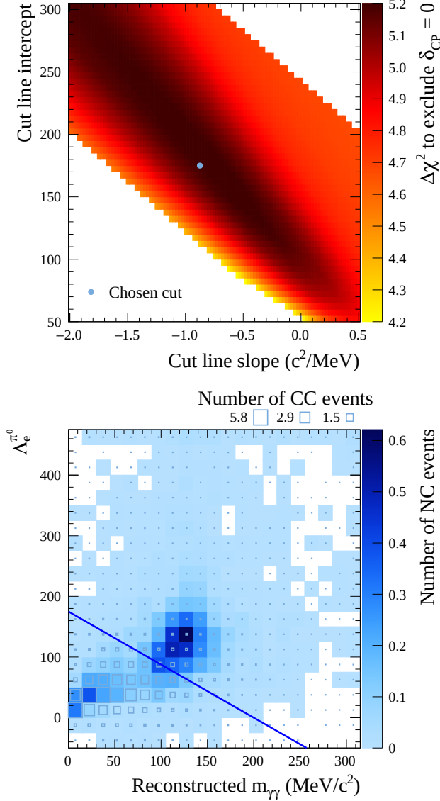
FIG. 29: The sensitivity to exclude \delta_{\text{CP}} = 0 as a function of the slope and intercept of the NC \pi^0 rejection cut line is shown on the top and the distribution of signal and background events is shown on the bottom, along with the line below which e -like events are selected.
