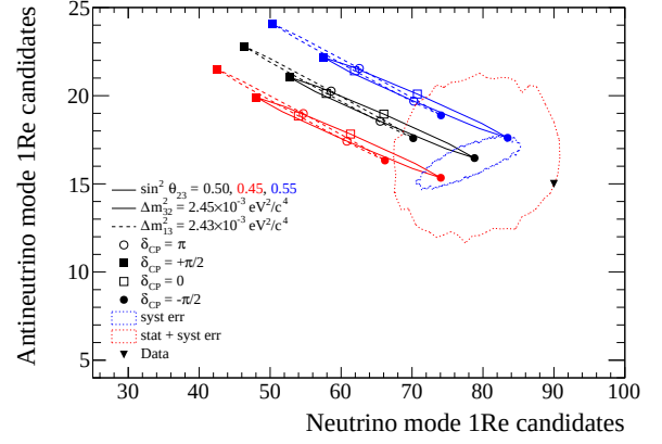
FIG. 72: Candidate RHC one-ring e -like event rate vs the candidate FHC one-ring e -like event rate (including CC 1\pi events) for a variety of different oscillation parameter values. Predictions are generated for the given values of \delta_{\text{CP}} , \sin^2\theta_{23} and mass ordering with remaining oscillation parameters fixed at the central values of the prior probability density functions defined in Sec. XIII A 1. The uncertainty regions are created assuming that \delta_{\text{CP}} = -\pi/2 , \sin^2\theta_{23} = 0.5 , \Delta m_{32}^2 = 2.45 \times 10^{-3} \text{eV}^2/c^4 and normal mass ordering.
