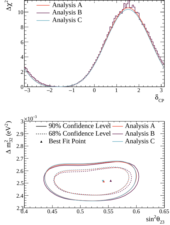
FIG. 47: Comparison between analyses A, B and C. The normal mass ordering is assumed and the reactor constraint is applied. Top: the predicted \Delta\chi^2 functions for \delta_{CP} . Bottom: the 1\sigma (dashed) and 90% (solid) CL regions for \Delta m^2 vs. \sin^2\theta_{23} .
