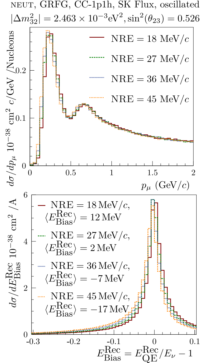
FIG. 8: Top: The predicted muon momentum spectrum for a number of different values of NRE in an oscillated SK flux. The shift towards lower momentum may be confused for a shift in |\Delta m_{32}^2| . Bottom: The effect of varying NRE on the reconstructed energy bias; higher values result in more energy ‘feed down’.
