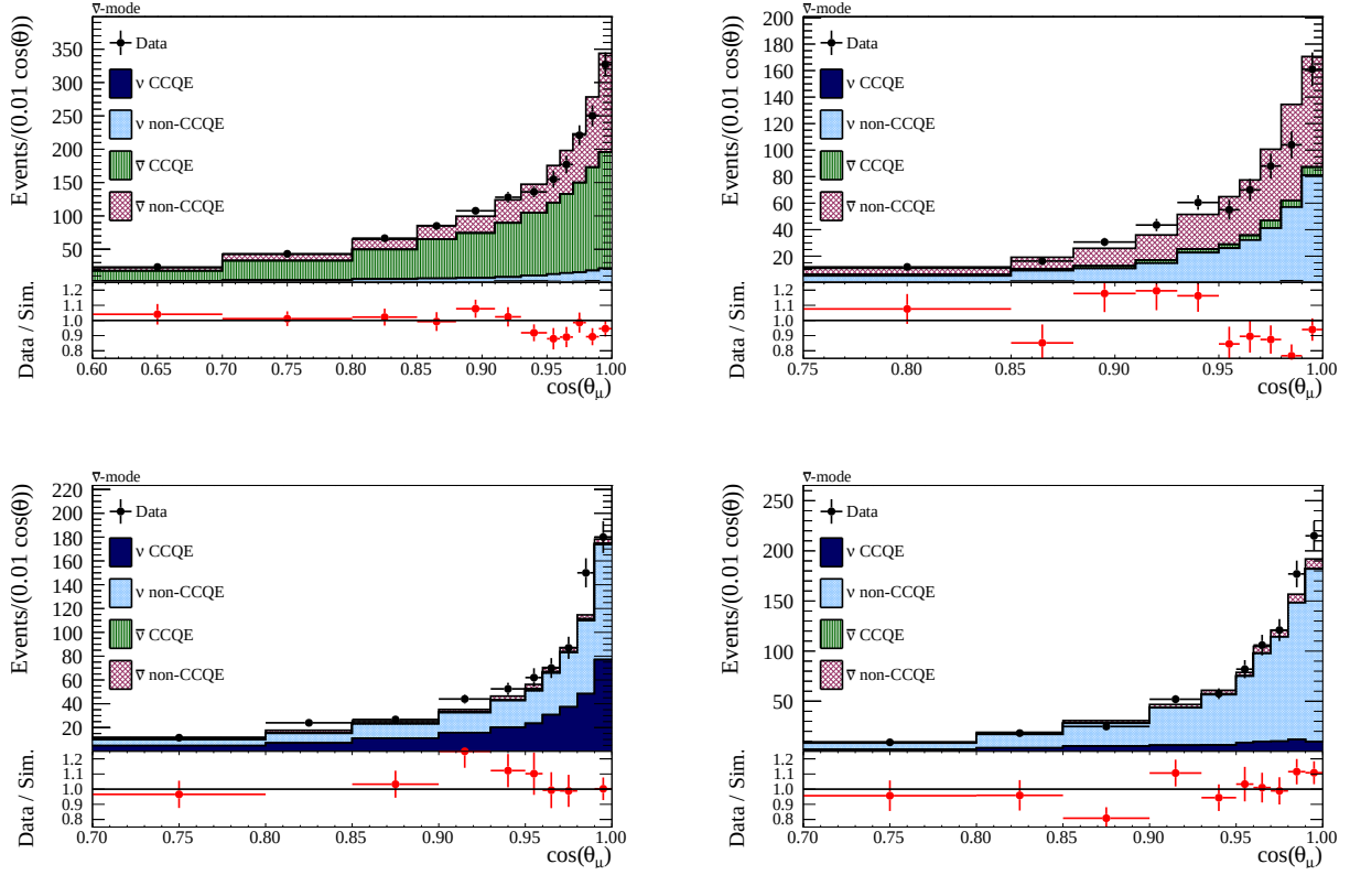
FIG. 14: Distributions of the final state muon angle for the RHC \bar{\nu}_\mu (top) and \nu_\mu (bottom) CC 1-track (left) and CC N-track (right) FGD1 simulation samples. These distributions are before the ND280 fit.
