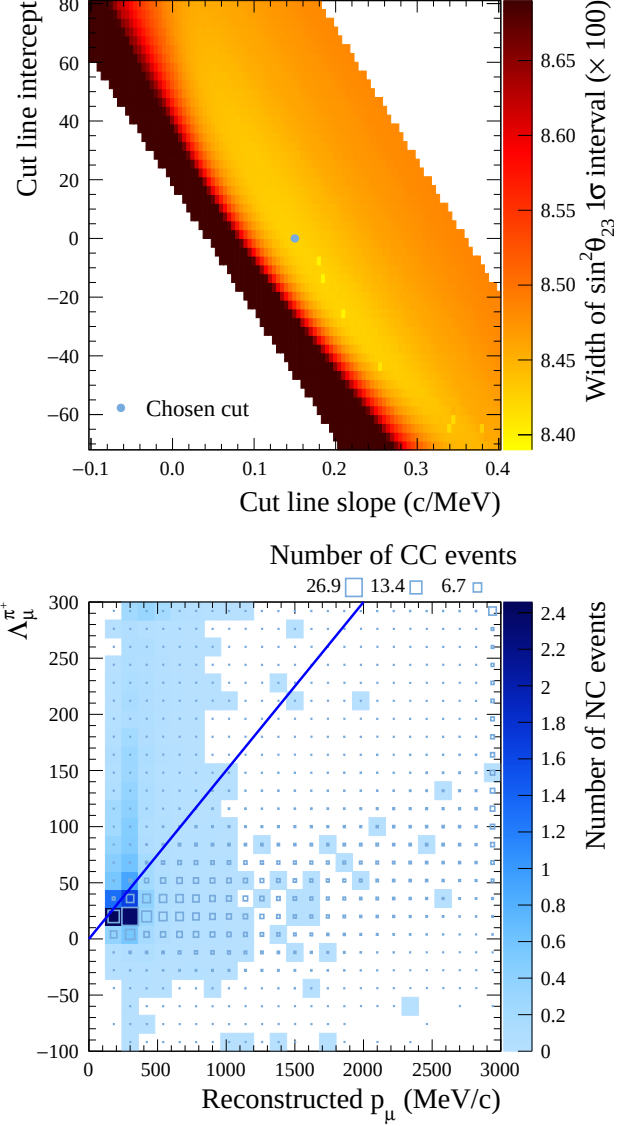
FIG. 28: The width of \sin^2 \theta_{23} 1\sigma confidence interval as a function of the slope and intercept of the \text{NC}\pi^+ rejection cut line is shown on the top and the distribution of signal and background events is shown on the bottom, along with the line below which \mu -like events are selected.
