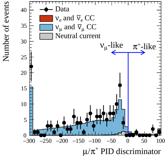
FIG. 21: Distribution of the \mu/\pi^+ PID discriminator for 1R_\mu events in FHC (top) and RHC (bottom) data.
