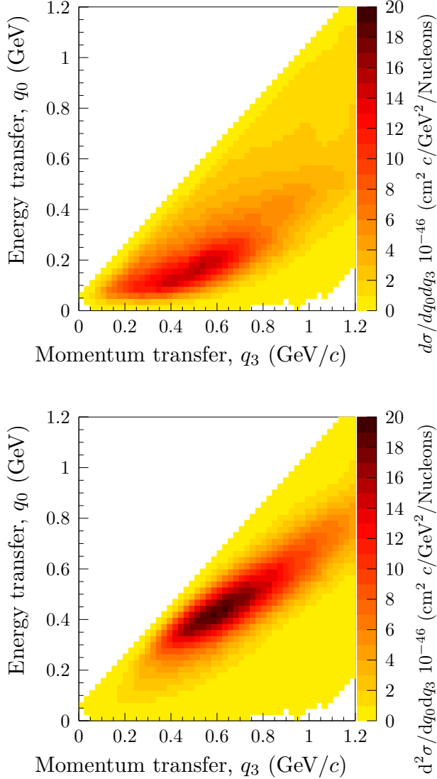
FIG. 6: The differential cross section for the two extreme variations of the 2p2h ‘shape’ parameter—QE-like (top) and Delta-like (bottom)— c.f. Fig. 4 (top) for the central-value-predicted cross section.
