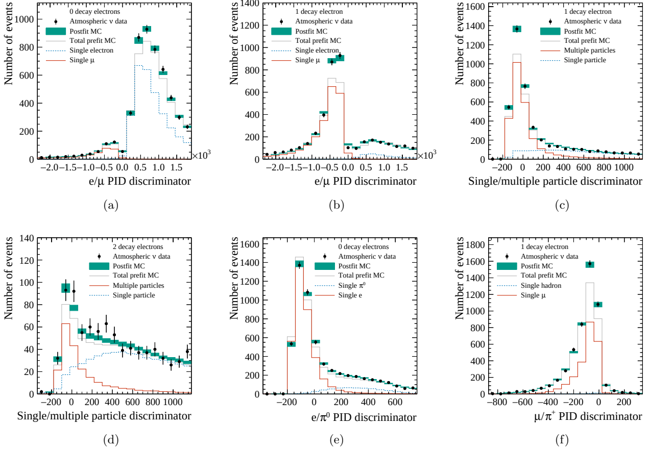
FIG. 31: Posterior predictive distributions of SK atmospheric MCMC fit to determine detector systematic uncertainties. The total nominal MC is shown in gray, with components targeted by each of the distributions shown in red and blue. The 68.27% intervals of the posterior predictive distribution is shown in green. Observed data are shown as black circles. All distributions shown are for the largest detector region, 5. Distributions of the e/\mu PID discriminator for 0 and 1 decay- e events are shown in (a) and (b). In (c) and (d), the particle-counting parameter is shown for events with 1 and 2 decay-electrons, respectively. The e/\pi^0 discriminator distribution is shown in (e) for e -like events and the \mu/\pi^+ distribution is shown in (f) for \mu -like events.
