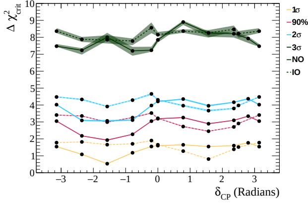
FIG. 59: Feldman–Cousins critical values for \delta_{\text{CP}} . The shaded bands represent the \pm 1\sigma Monte Carlo statistical uncertainty on the calculated critical values.
