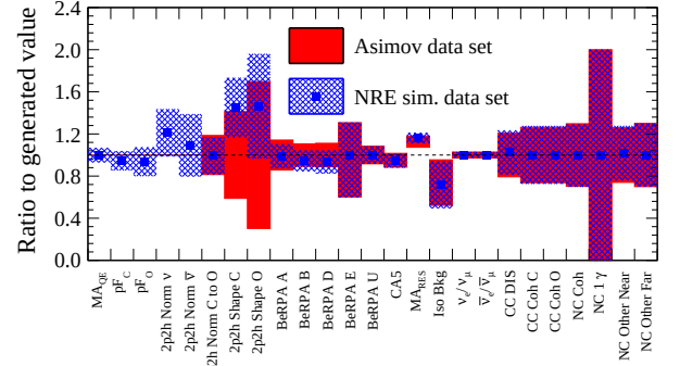
FIG. 50: Results of the fit to the near detector simulated data with an increased nucleon removal energy. The best fit values for the \nu_\mu flux parameters at SK (top) and cross-section parameters (bottom) are shown for the NRE fit (blue) compared to the Asimov data set fit (red).
