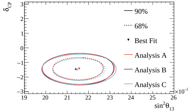
FIG. 57: Comparison between the observed 1\sigma (dashed) and 90% (solid) CL regions for \delta_{CP} vs \sin^2\theta_{13} produced using analyses A, B and C, assuming normal mass ordering (top) or inverted mass ordering (bottom). The reactor constraint is applied.
