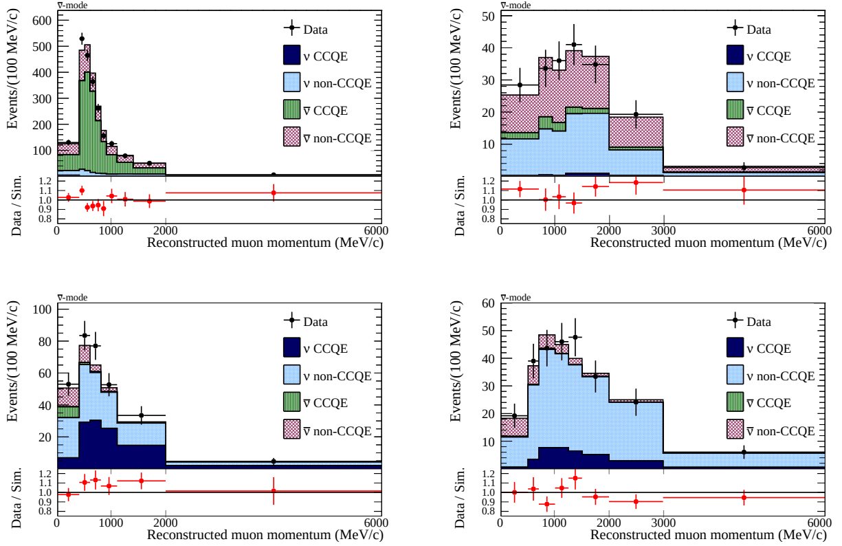
FIG. 13: Final state muon momentum distributions for the RHC \bar{\nu}_\mu (top) and \nu_\mu (bottom) CC 1-track (left) and CC N -track (right) FGD1 simulation samples. These distributions are before the ND280 fit.
