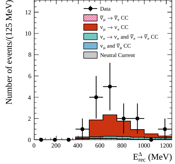
FIG. 26: Reconstructed energy distribution for 1R_e + 1 d.e. events in FHC data. The \Delta(1232) mass is used for the final-state nucleon in the reconstructed neutrino energy calculation.
