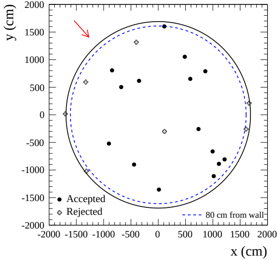
FIG. 23: Reconstructed vertices of selected RHC data 1R_e events projected in z vs r^2 (top) and y vs x (bottom). The neutrino beam direction is shown as a red arrow and events which do not pass the fiducial volume criteria are shown as hollow crosses.
