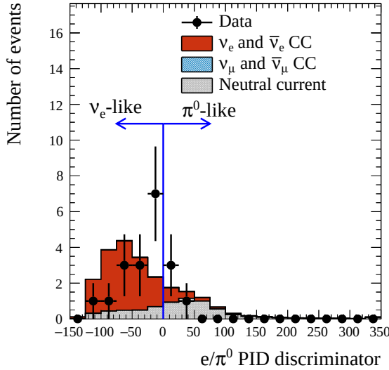
FIG. 19: Distribution of the e/\pi^0 PID discriminator for 1R_e events in FHC (top) and RHC (bottom) data.
