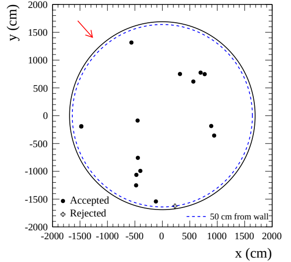
FIG. 24: Reconstructed vertices of selected FHC data 1R_e + 1 d.e. events projected in z vs r^2 (top) and y vs x (bottom). The neutrino beam direction is shown as a red arrow and events which do not pass the fiducial volume criteria are shown as hollow crosses.
