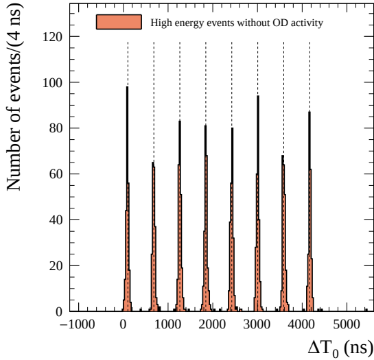
FIG. 15: Reconstructed event time distributions in the 1 ms (top) and [-1.2, 5.6] \mu\text{s} (bottom) windows around the beam spill leading edge.
