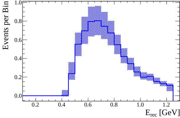
FIG. 41: Post-ND280-fit predicted event spectrum for the FHC beam SK samples as a function of E_{QE}^{Rec} . The samples are: single-ring muon-like (top), single-ring electron-like without decay electrons (middle) and single-ring electron-like with a single decay electron (bottom).
