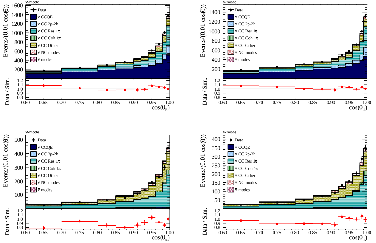
FIG. 12: Distributions of the final state muon angle of the FHC \nu_\mu CC 0\pi (top) and \nu_\mu CC 1\pi^+ (bottom) data and simulation samples in FGD1 (left) and FGD2 (right).
