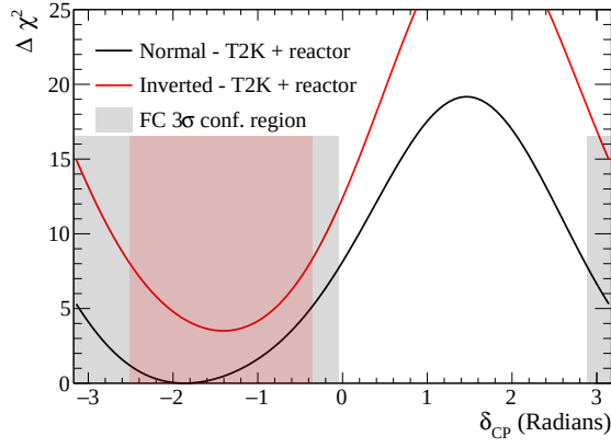
FIG. 60: The observed 3\sigma Feldman–Cousins (FC) confidence intervals for \delta_{\text{CP}} . The \Delta\chi^2 is computed with respect to the best fit over the 2 mass orderings.
