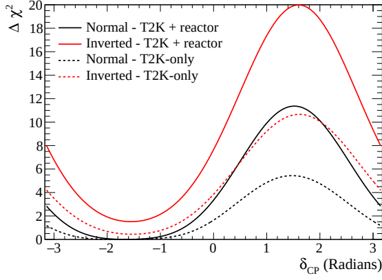
FIG. 45: The predicted \Delta\chi^2 = -2\ln[L/L_{max}] function as a function of \delta_{CP} with and without reactor constraint, for both mass orderings.
