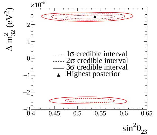
FIG. 63: Bayesian credible regions for \Delta m_{32}^2 against \sin^2\theta_{23} covering both mass orderings.
