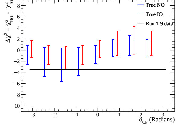
FIG. 70: Ability to distinguish between the two mass orderings as a function of the true value of \delta_{\text{CP}} . The bar indicates the range of values of \Delta\chi^2 = \chi^2_{\text{NO}} - \chi^2_{\text{IO}} which contains 95% of the values obtained for the pseudo-experiments generated in each case. The black line corresponds to the value obtained in the data fit by Analysis A.
