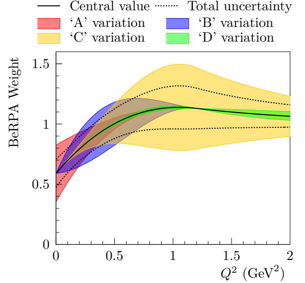
FIG. 5: The central value BeRPA suppression factor (solid) and the total prior uncertainty (dashed) determined from 10^5 uncorrelated throws of the free parameters, overlaid on the corresponding envelopes generated by varying each parameter. The continuity conditions result in a perhaps unintuitive total uncertainty envelope given the individual parameter variations.
