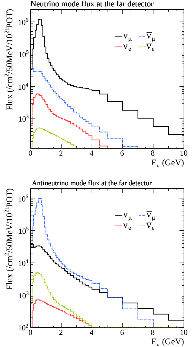
FIG. 1: The SK flux prediction for Runs 1–9a with horns operating in FHC (250 kA) mode (upper) and RHC (–250 kA) mode (lower).
