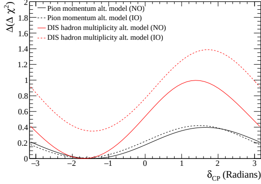
FIG. 68: Change in the \Delta\chi^2 function for \delta_{\text{CP}} when fitting data using an alternative model for DIS hadron multiplicity (red) and pion momentum spectra (black). The \Delta\chi^2 was reduced by the value shown on the plot in each case. The difference is shown for the model change that gave the largest difference in each case.
