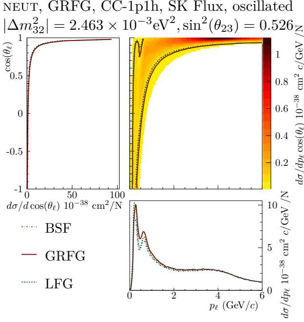
FIG. 7: The predicted flux-averaged cross section for three different nuclear response models. The different models result in different predictions of the observed final-state lepton kinematics for the same oscillated neutrino flux. If such variations are not accounted for in the uncertainty model, extracted oscillation parameters may be biased. The contours contain the region of phase space with a differential cross section d\sigma/dp_\ell \cos(\theta_\ell) > 0.05 \times 10^{-38} \text{ cm}^2 \text{ c}/\text{GeV} / \text{N} .
