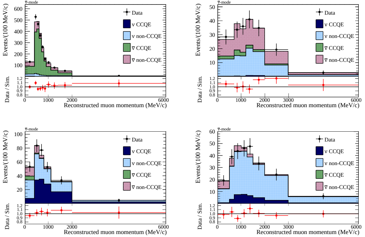
FIG. 39: Post ND280 fit muon momentum distributions for the RHC \bar{\nu}_\mu (top) and \nu_\mu (bottom) CC 1-track (left) and CC N -track (right) FGD1 samples.
