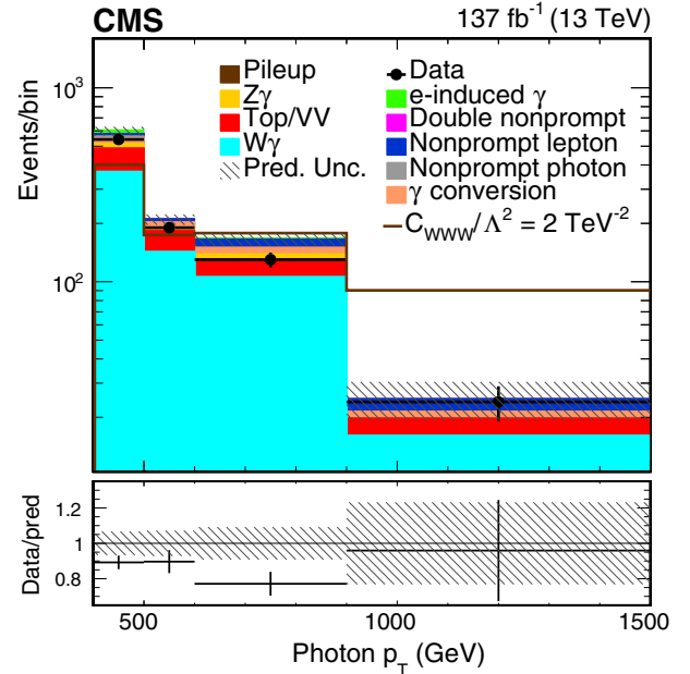
FIG. 3. The photon p_T distribution used for the extraction of limits on dimension-six EFT operators. The expected yields correspond to the estimates made before the fit. The uncertainty in the prediction (the hatched band) is the quadratic sum of the systematic uncertainties. The uncertainty in the data is statistical. The last bin includes the overflow.
