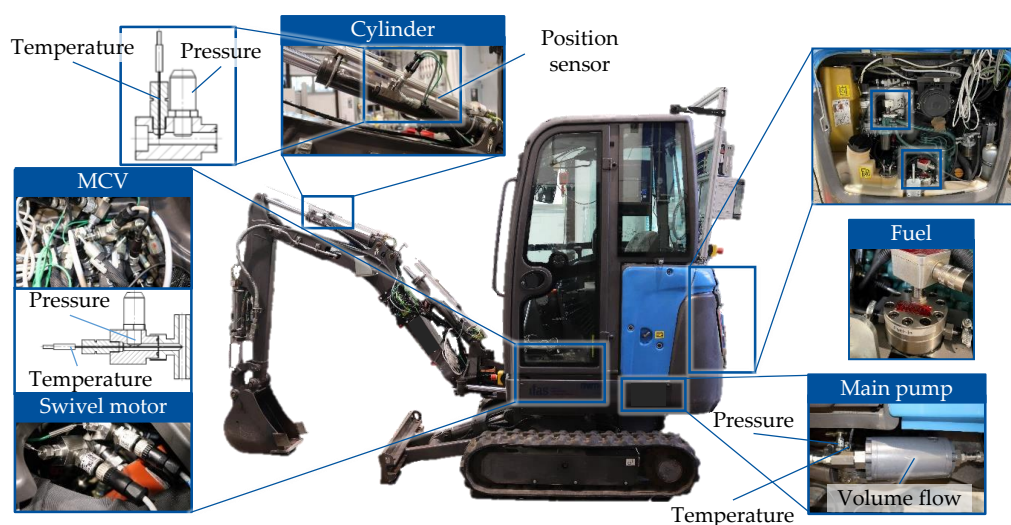
Figure 8. Integration measurement equipment test excavator.
