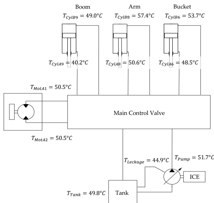
Figure 9. Maximum temperature during the reference cycle.
