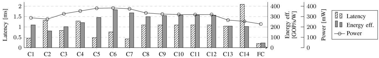
FIGURE 13. Results for convolutional layers of MobileNet. Stated values depict the combined depthwise and pointwise convolution.
