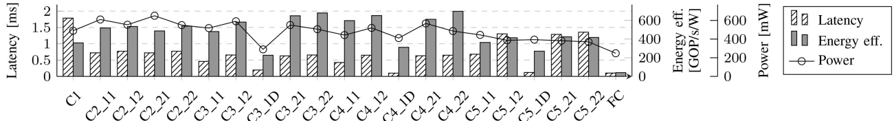
FIGURE 14. Results for convolutional layers of ResNet-18. Entries with a D suffix are downsample layers.
