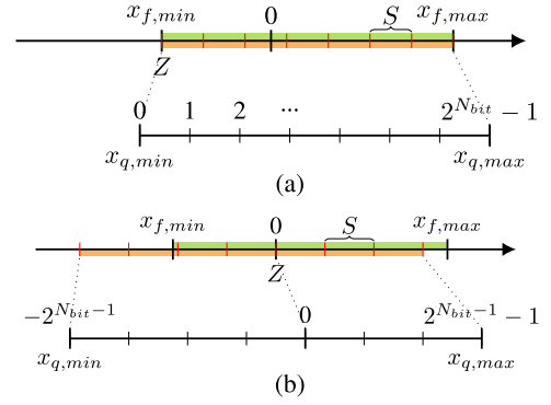
FIGURE 2. Asymmetric (a) and symmetric (b) integer-only quantization.
