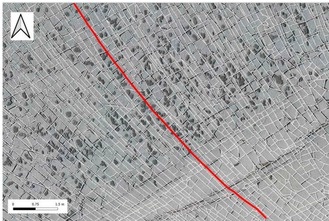
Fig. 12. Continuous and sinuous fracture from Area 4 automatically joined from graph segments with a strike threshold of 20^\circ . Note that the strike of the start and end segment of the fracture vary by more than 50^\circ .
