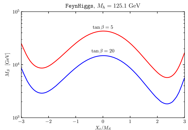
Fig. 2 Values of the SUSY mass parameter M_S and of the stop mixing parameter X_t (normalized to M_S ) that lead to the prediction M_h = 125.1 GeV, in a simplified MSSM scenario with degenerate SUSY masses, for \tan \beta = 20 (blue) or \tan \beta = 5 (red)
