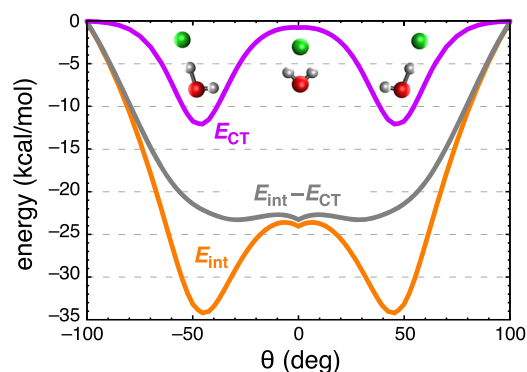
FIG. 30. Total interaction potential ( E_{\text{int}} ) for \text{F}^-(\text{H}_2\text{O}) along a relaxed radial scan of the \text{XOH} angle, \theta . Also shown is a SAPT/cDFT-EDA decomposition of E_{\text{int}} into a CT component ( E_{\text{CT}} ) and a CT-free interaction energy, E_{\text{int}} - E_{\text{CT}} . As the ion circumscribes the water molecule, E_{\text{CT}} turns on sharply in the vicinity of quasi-linear hydrogen bonds. Removal of CT stabilization results in a C_{2v} -symmetric structure, in disagreement with experiment, 662 although the “dipolar” C_{2v} structure can still be found in many undergraduate textbooks, e.g., Ref. 663. Adapted with permission from J. M. Herbert and K. Carter-Fenk, J. Phys. Chem. A 125 , 1243 (2021). Copyright 2021 American Chemical Society.
