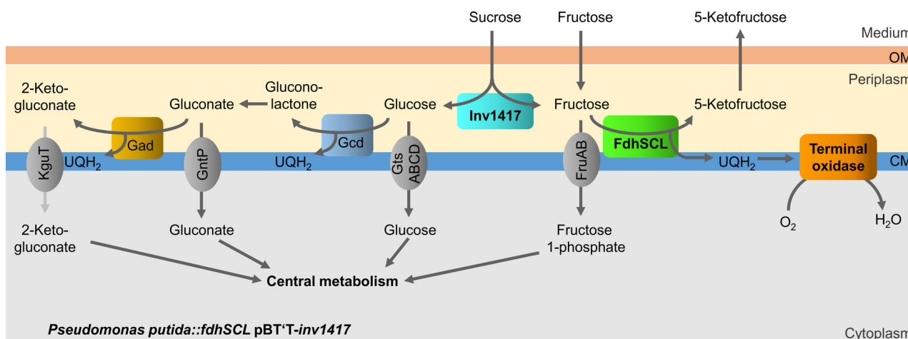
Fig. 6. Schematic overview of sugar metabolism and 5-KF production in P. putida::fdhSCL (pBT-T-inv1417). Sucrose and fructose enter the periplasm via porins (not shown) in the outer membrane (OM). Sucrose is cleaved by the periplasmic invertase Inv1417 of G. japonicus to glucose and fructose. Fructose is oxidized to 5-ketofructose by the membrane-bound fructose dehydrogenase FdhSCL from G. japonicus . Glucose can be taken up into the cytosol via the cytoplasmic membrane (CM) by the glucose transport system (GtsABCD) or is oxidized by the PQQ-dependent glucose dehydrogenase (Gcd) to gluconolactone, which is subsequently hydrolyzed to gluconate. Gluconate can be taken up via the gluconate permease (GntP) or is further oxidized by the gluconate dehydrogenase (Gad) to 2-ketogluconate, which can be taken up via the ketogluconate transporter (KgtT). Periplasmic oxidation by the membrane-bound dehydrogenases generates ubiquinol, which is oxidized in the respiratory chain either directly by ubiquinol oxidases or via the cytochrome bc 1 complex and cytochrome c oxidases.
