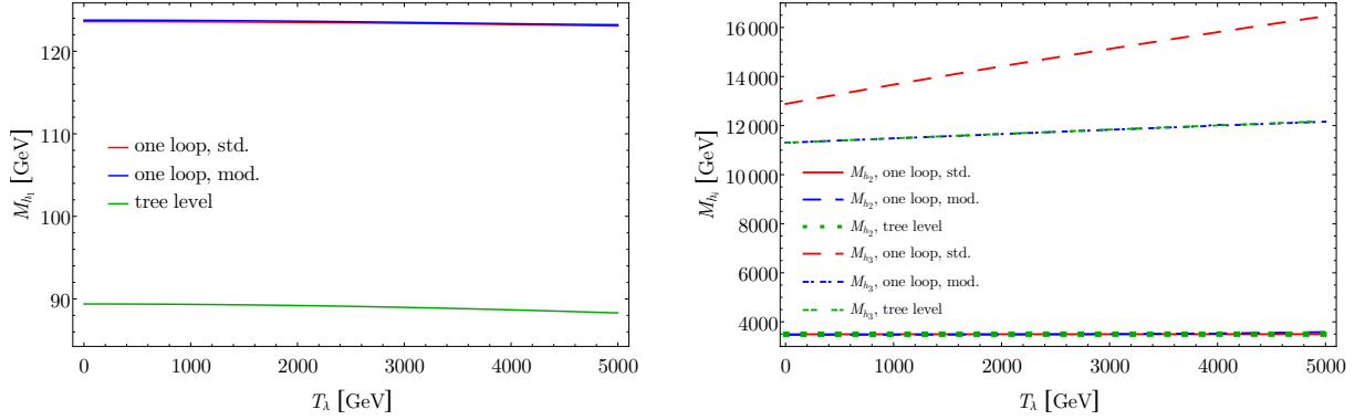
Figure 10: M_{h_1} (left) and M_{h_2} and M_{h_3} (right) as a function of the soft trilinear coupling T_\lambda , in scenario 2. The values of the other BSM parameters are taken as in table 1.
