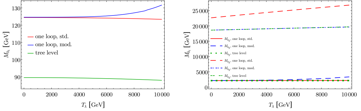
Figure 12: M_{h_1} (left) and M_{h_2} and M_{h_3} (right) as a function of T_\lambda , in scenario 3. The other BSM inputs are taken as in table 1.
