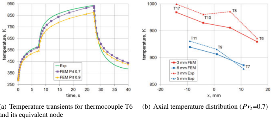
Fig. 4 Comparison of thermocouple measurements and its corresponding FEM node temperatures
