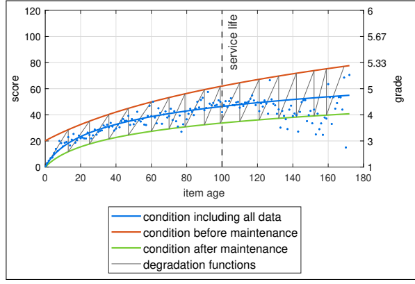
Fig. 6. Life cycle function. Plot of the intervention threshold (red) and of the condition after a maintenance measure (green). The blue line corresponds to the performed logarithmic regression including all available data. The degradation function of an average item is indicated by the gray lines.
