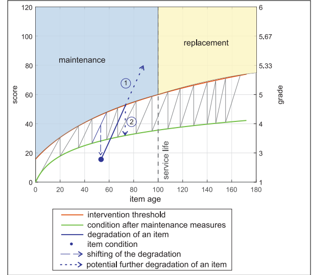
Fig. 7. Assignment of degradation functions and classification of measures. Plot of the intervention threshold (red) and of the condition after a maintenance measure (green). The purple dot indicates a sample item. The degradation of the item according to its age is shifted to the item (purple arrow). At the intersection with the intervention threshold, the item can either deteriorate further based on the shifted degradation function (dashed purple arrow ①) or receive a maintenance measure that improves the item's score to the lower boundary function (dashed purple arrow ②).
