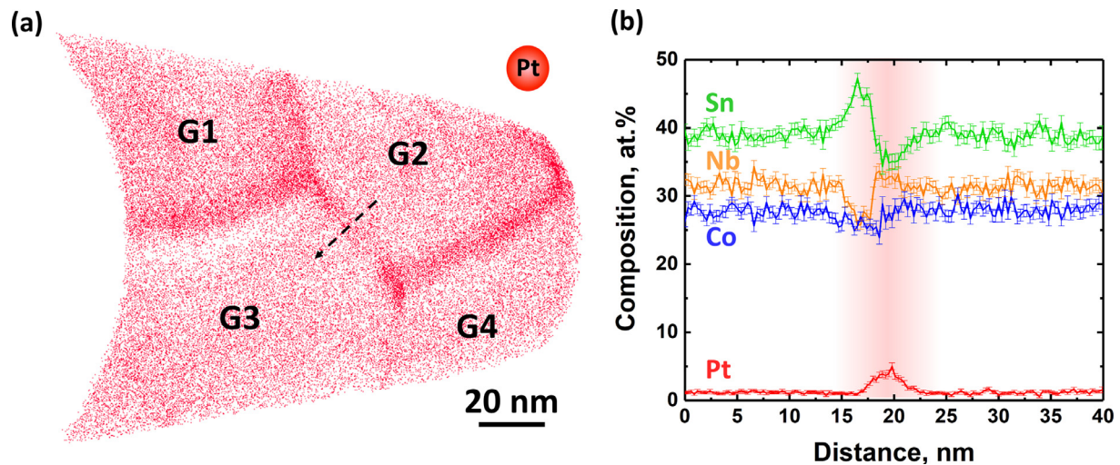
Fig. 3. APT analysis of NbCoSn-Pt: (a) distribution map of Pt atoms, indicating the presence of four grains (G1, G2, G3 and G4); (b) 1D-composition profile in a 20 nm-diameter cylinder perpendicular to the G2/G3 grain boundary.
