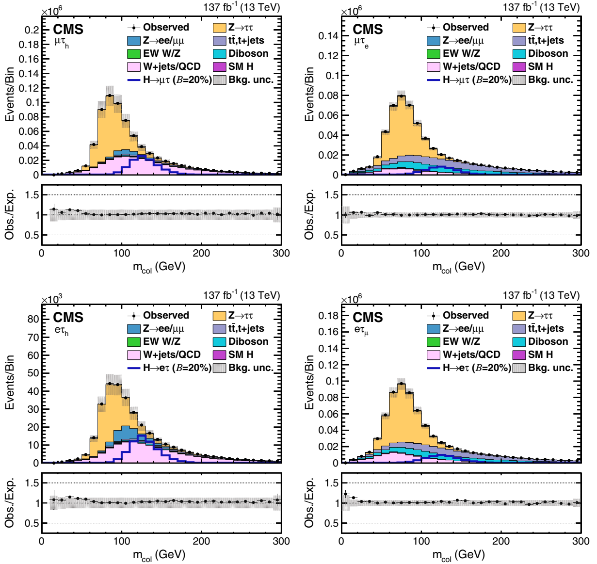
FIG. 1. Collinear mass distributions for the data and background processes. A B(H \rightarrow \mu\tau) = 20\% and B(H \rightarrow e\tau) = 20\% are assumed for the two signal processes. The channels are H \rightarrow \mu\tau_h (upper row left), H \rightarrow \mu\tau_e (upper row right), H \rightarrow e\tau_h (lower row left), and H \rightarrow e\tau_\mu (lower row right). The lower panel in each plot shows the ratio of data and estimated background. The uncertainty band corresponds to the background uncertainty in which the statistical and systematic uncertainties are added in quadrature.
