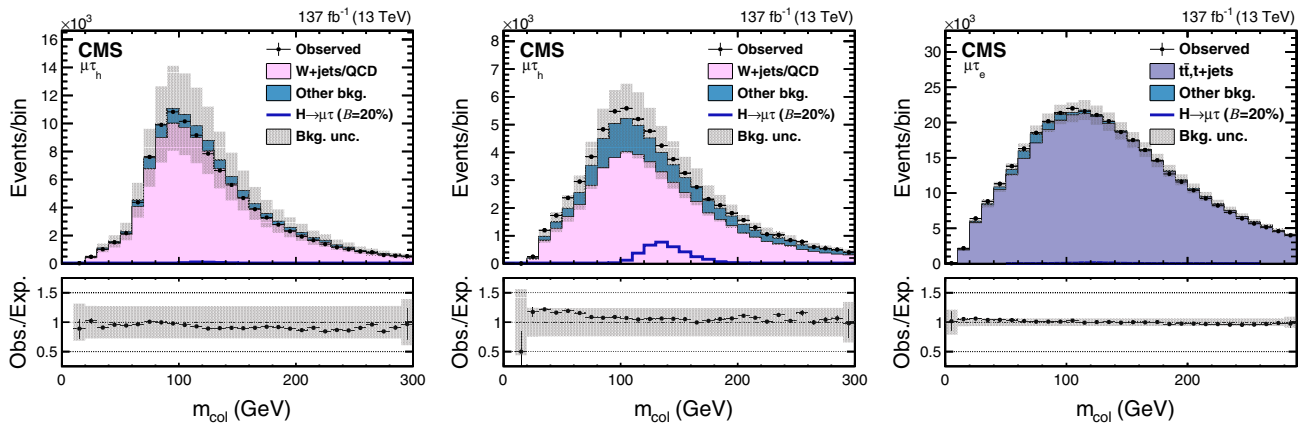
FIG. 6. The m_{\text{col}} distribution in VR with same electric charge for both leptons (left), W + \text{jets} VR (middle), and t\bar{t} VR (right). In each distribution, the VR’s dominant background is shown, and all the other backgrounds are grouped into “Other bkg.”. A \mathcal{B}(H \rightarrow \mu\tau) = 20\% is assumed for the signal. The lower panel in each plot shows the ratio of data and estimated background. The uncertainty band corresponds to the background uncertainty in which the post-fit statistical and systematic uncertainties are added in quadrature.
