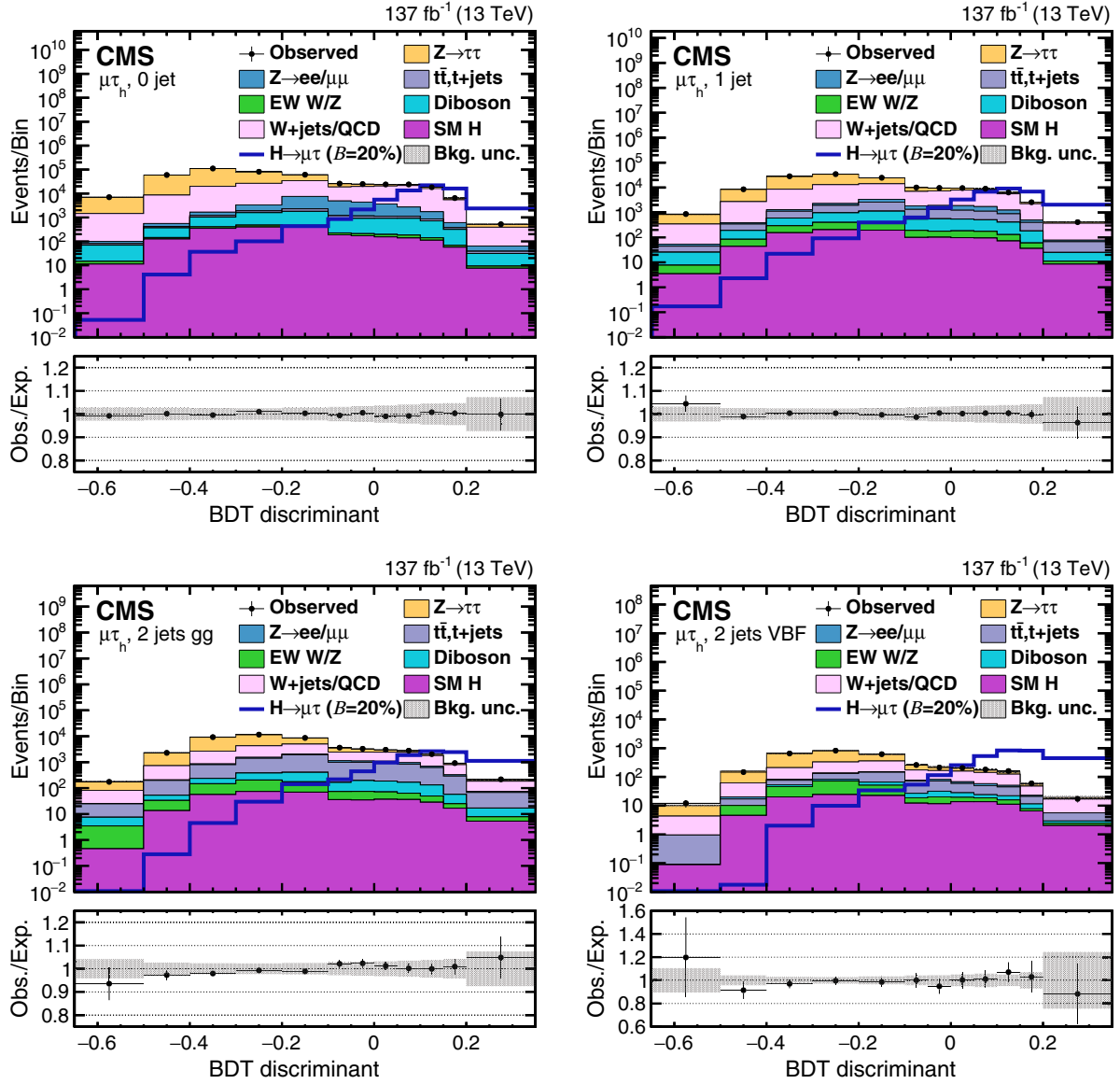
FIG. 2. BDT discriminant distributions for the data and background processes in the H \rightarrow \mu\tau_h channel. A B(H \rightarrow \mu\tau) = 20\% is assumed for the signal. The channel categories are zero jets (upper row left), one jet (upper row right), two jets ggH (lower row left), and two jets VBF (lower row right). The lower panel in each plot shows the ratio of data and estimated background. The uncertainty band corresponds to the background uncertainty in which the postfit statistical and systematic uncertainties are added in quadrature.
