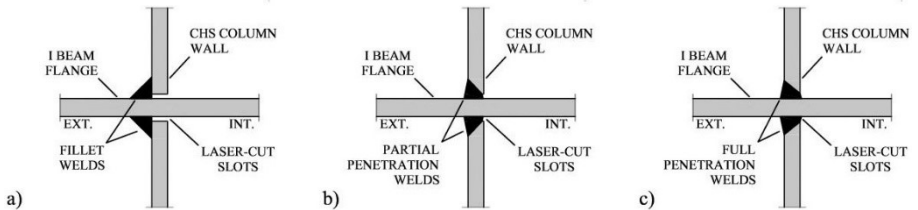
Figure 5.9 Welding possibilities for passing-through elements: a) fillet, b) partial penetration, and c) full penetration welding
