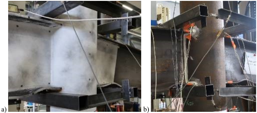
Figure 6.14 Failure mode exhibited in the C3 specimens under symmetric vertical loads: local buckling of the compressed beam flanges of specimen a) C3-1B-1, and b) C3-3A-1
