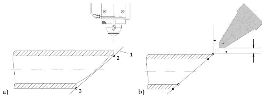
Figure 5.2 Laser cutting possible geometries: a) 2D cutting VS b) 3D cutting (Castiglioni et al. 2016)
