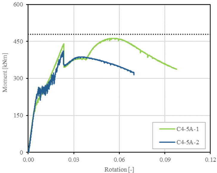
Figure 6.20 Results of monotonic test on C4 specimens, with 12.5 mm thick column, in the symmetric configuration (vertical loading configuration); the dot line represents the beam design resistance
