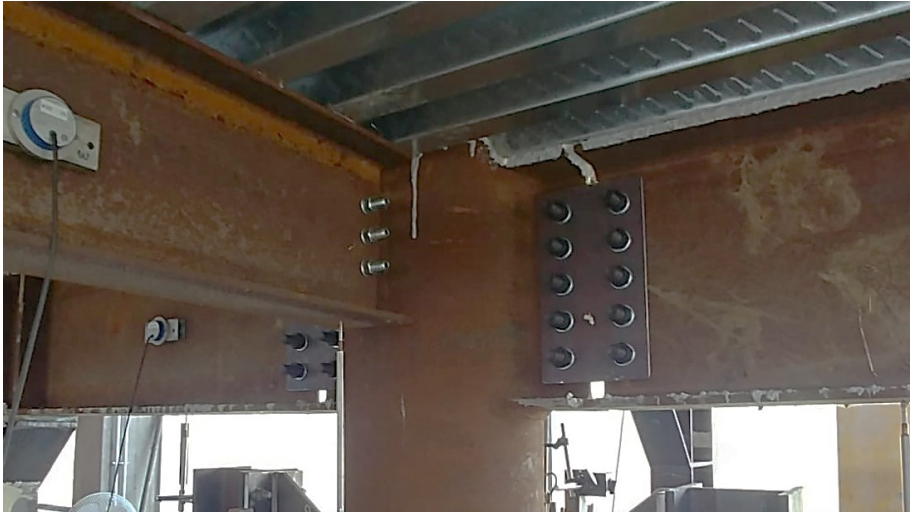
Figure 8.13 Four-way specimen C5 tested under vertical loads
