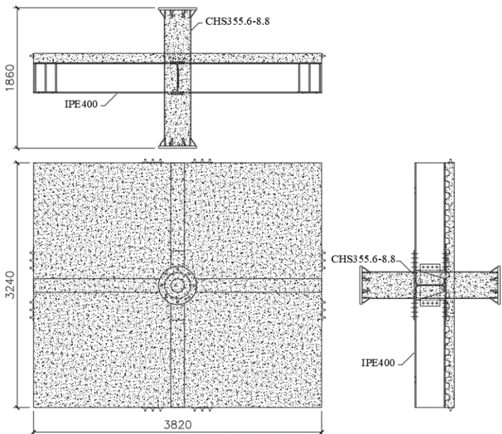
Figure 7.17 Details of specimen C7
