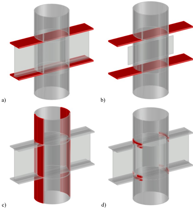
Figure 10.7 Axially loaded components: a) through beam flanges (type C3), b) through flange plates (type C4), c) tubular column wall, and d) flange welds
