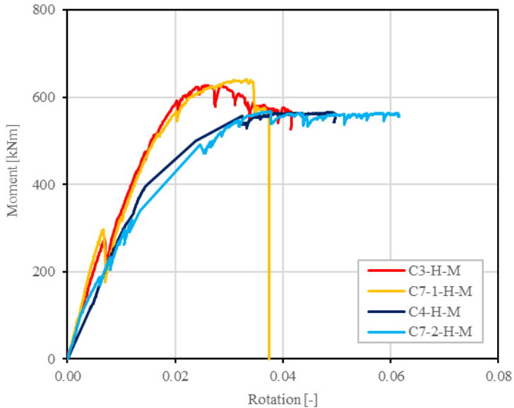
Figure 9.37 Comparison of the curves representing the behavior of the specimens with the passing-through beam in the tested direction (C3 and C7-1) and the specimens with the three passing-through plates in the tested direction (C4 and C7-2)
