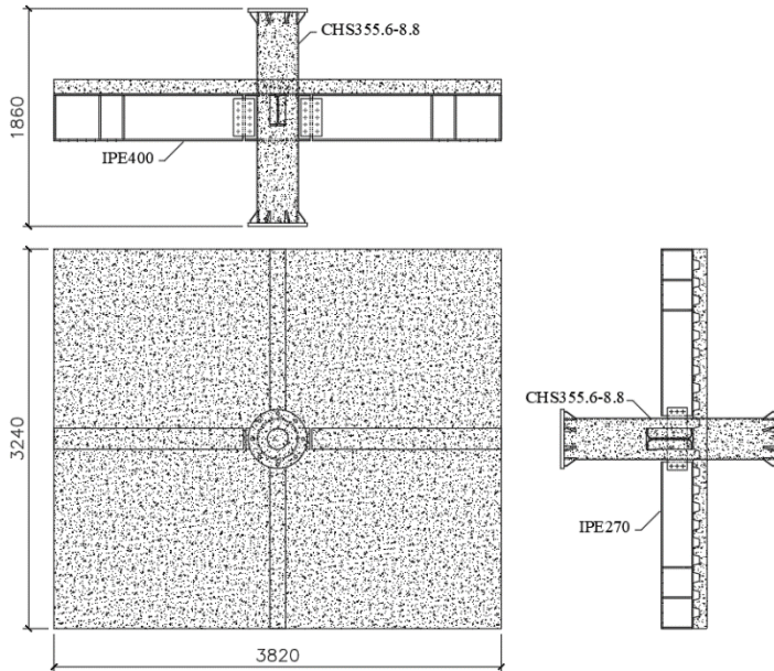
Figure 7.15 Details of specimen C5
