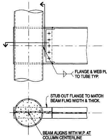
Figure 2.13 Connection made by passing-through plates (Alostaz and Schneider 1996a)
