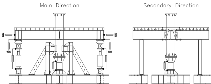
Figure 8.9 LVDTs displacement transducers disposed in the test setup and on the specimen in each testing setup
