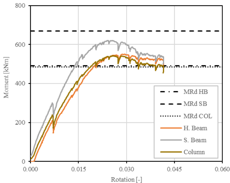
Figure 9.16 Moment-rotation curves for the C3 two-way specimen; the column bending moment is calculated in the sections on the top and on the bottom of the connection
