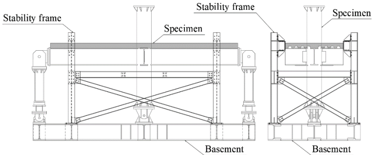
Figure 9.6 Stability frame designed in order to avoid lateral displacement
