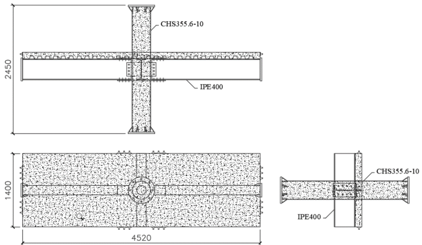
Figure 7.24 C7-2 to be tested under horizontal loads
