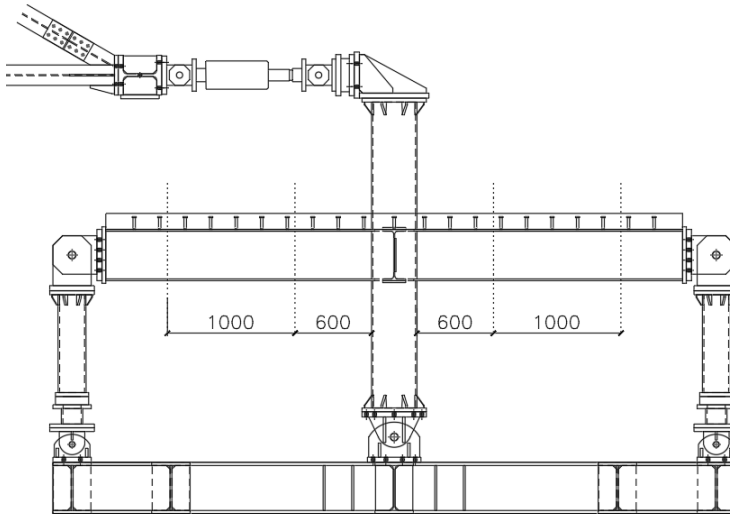
Figure 9.10 Beam sections controlled by strain gauges
