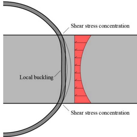
Figure 10.15 Force transmission in the compression region
