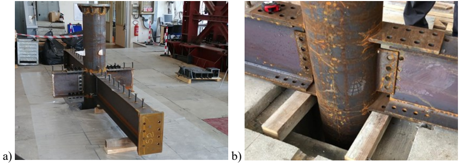
Figure 7.27 Assembly operations in the laboratory: a) specimen C7-1, and b) specimen C4
