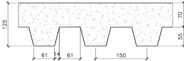
Figure 7.7 Dimensions of the composite slab
