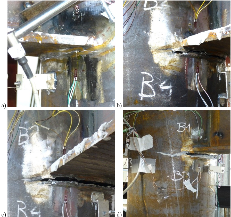
Figure 9.21 Failures of the penetration welds: a) first lesion exhibited in the first cycle at 40 mm, b) propagation of the lesion to the column wall in the first cycle at 60 mm, c) and d) bottom weld regions in the end of the test
