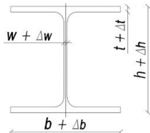
Figure 5.3 Nominal dimensions and tolerances
