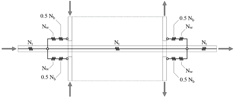
Figure 10.13 Assembly of the components in the flange region; each component can have different strength in compression and in tension
