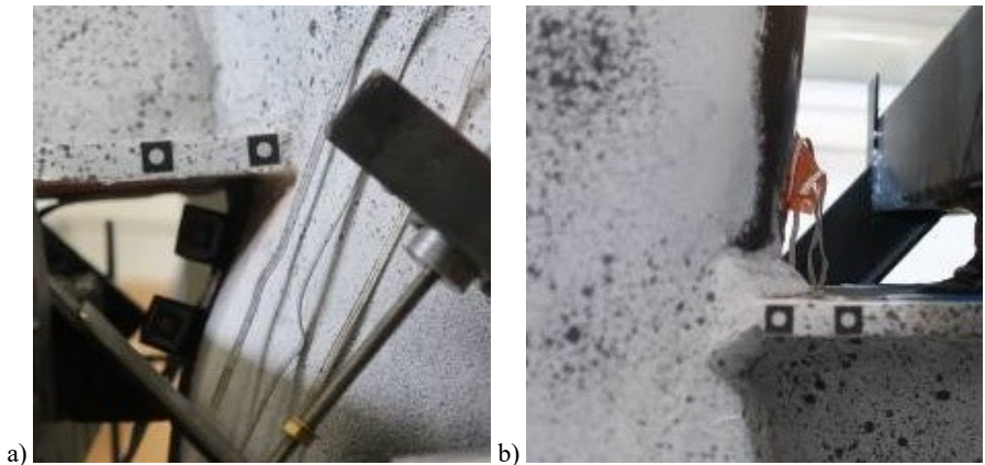
Figure 6.25 Local buckling of the column wall where compression forces are transmitted by the flanges: a) C3-1B-2 specimen with 8.8 mm thick column and full penetration welding, and b) C3-3A-2 specimen with 12.5 mm thick column and fillet welding
