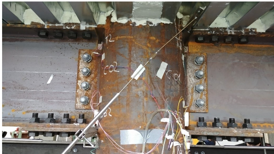
Figure 9.22 Two-way specimen C4 with the passing-through plates bolted to the girders
