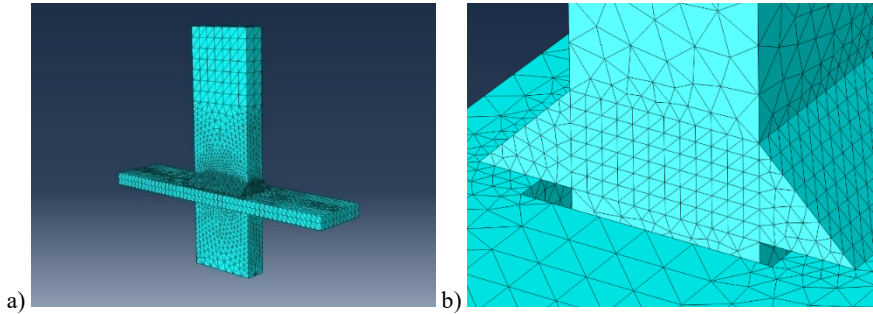
Figure 5.21 Preliminary numerical model of the welds for the “2C” model (Table 5.3): a) global 3D view and b) particular of the mesh adopted in the model
