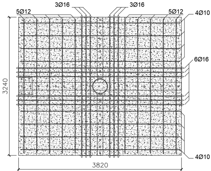
Figure 7.19 Concrete slab details for the specimen C6
