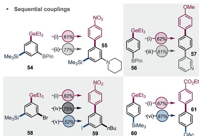
Figure 3. i) \text{ArGeEt}_3 (0.3 mmol), \text{ArN}_2\text{BF}_4 (0.36–0.45 mmol), [(\text{PPh}_3)\text{AuCl}] (0.03 mmol), MeCN; ii) \text{ArBpin} (0.2 mmol), \text{Cu}(\text{OAc})_2 (0.2 mmol), \text{NEt}_3 (0.4 mmol), piperidine (0.4 mmol), MeCN; iii) \text{ArBpin} (0.20 mmol), \text{ArBr} (0.22 mmol), \text{K}_2\text{CO}_3 (0.40 mmol), \text{Pd}(\text{dppf})\text{Cl}_2\cdot\text{CH}_2\text{Cl}_2 (0.01 mmol), 1,4-dioxane; iv) \text{ArBr} (0.20 mmol), \text{AlkZnCl/LiCl} (0.46 mmol), \text{Pd}^{\text{I}} -dimer (0.005 mmol); v) \text{ArSiMe}_3 (0.3 mmol), N-iodo succinimide (0.6 mmol), p\text{TsOH} (0.6 mmol), \text{CHCl}_3 ; vi) \text{ArSiMe}_3 (0.2 mmol), \text{PhI}(\text{O}_2\text{CCF}_3) (0.3 mmol), \text{Pd}(\text{OAc})_2 (0.01 mmol), AcOH.
