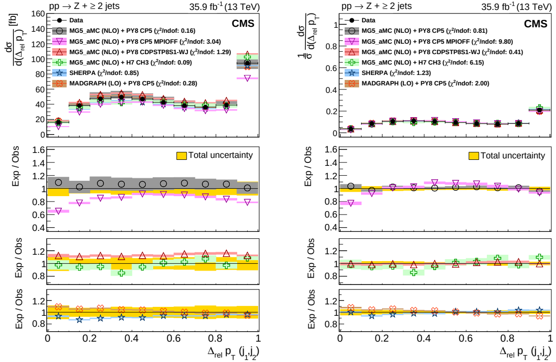
Figure 6: Differential cross sections (left) and area-normalized distributions (right) as functions of the p_T imbalance between leading and subleading jets for Z + \geq 2 jet events. The uncertainties in the predictions are shown as coloured bands around the theoretical predictions including statistical, PDF, scale, and tune uncertainties for the NLO MG5_aMC + PYTHIA8 (with CP5 tune) and the statistical uncertainty only for the LO MG5_aMC + PYTHIA8 (with CP5 tune), NLO MG5_aMC + PYTHIA8 (with CDPSTP8S1-WJ tune, CP5 tune with MPI-OFF), NLO MG5_aMC + HERWIG7 (with tune CH3), and SHERPA predictions. In the top panel, the vertical bars on the data points represent statistical uncertainties, whereas in the bottom panels, the total uncertainty in data is indicated by the solid yellow band centred at 1. In the legend, the \chi^2 per degree of freedom is given to quantify the goodness of fit of the model to the data.
