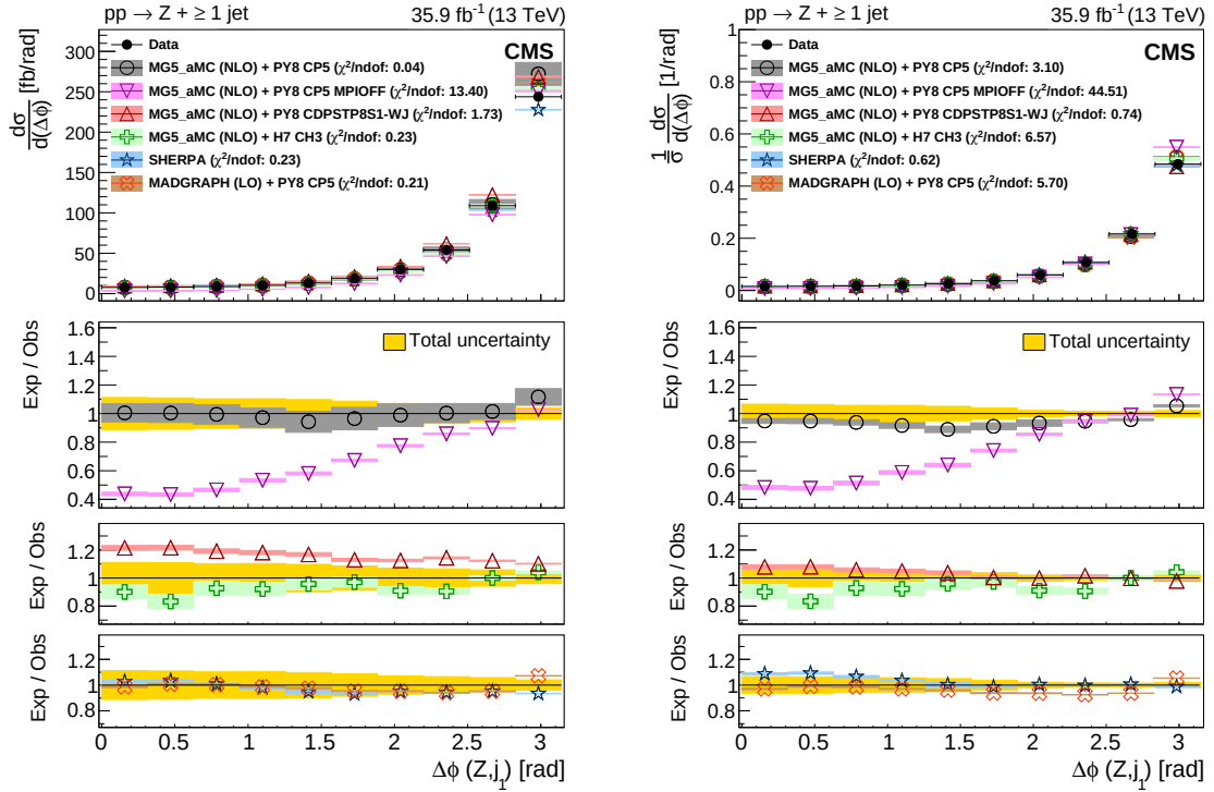
Figure 2: Differential cross sections (left) and area-normalized distributions (right) as functions of \Delta\phi between the Z boson and the leading jet for Z + \geq 1 \text{ jet} events. The uncertainties in the predictions are shown as coloured bands around the theoretical predictions including statistical, PDF, scale, and tune uncertainties for the NLO MG5_aMC + PYTHIA8 (with CP5 tune) and the statistical uncertainty only for the LO MG5_aMC + PYTHIA8 (with CP5 tune), NLO MG5_aMC + PYTHIA8 (with CDPSTP8S1-WJ tune, CP5 tune with MPI-OFF), NLO MG5_aMC + HERWIG7 (with tune CH3), and SHERPA predictions. In the top panel, the vertical bars on the data points represent statistical uncertainties, whereas in the bottom panels, the total uncertainty in data is indicated by the solid yellow band centred at 1. In the legend, the \chi^2 per degree of freedom is given to quantify the goodness of fit of the model to the data.
