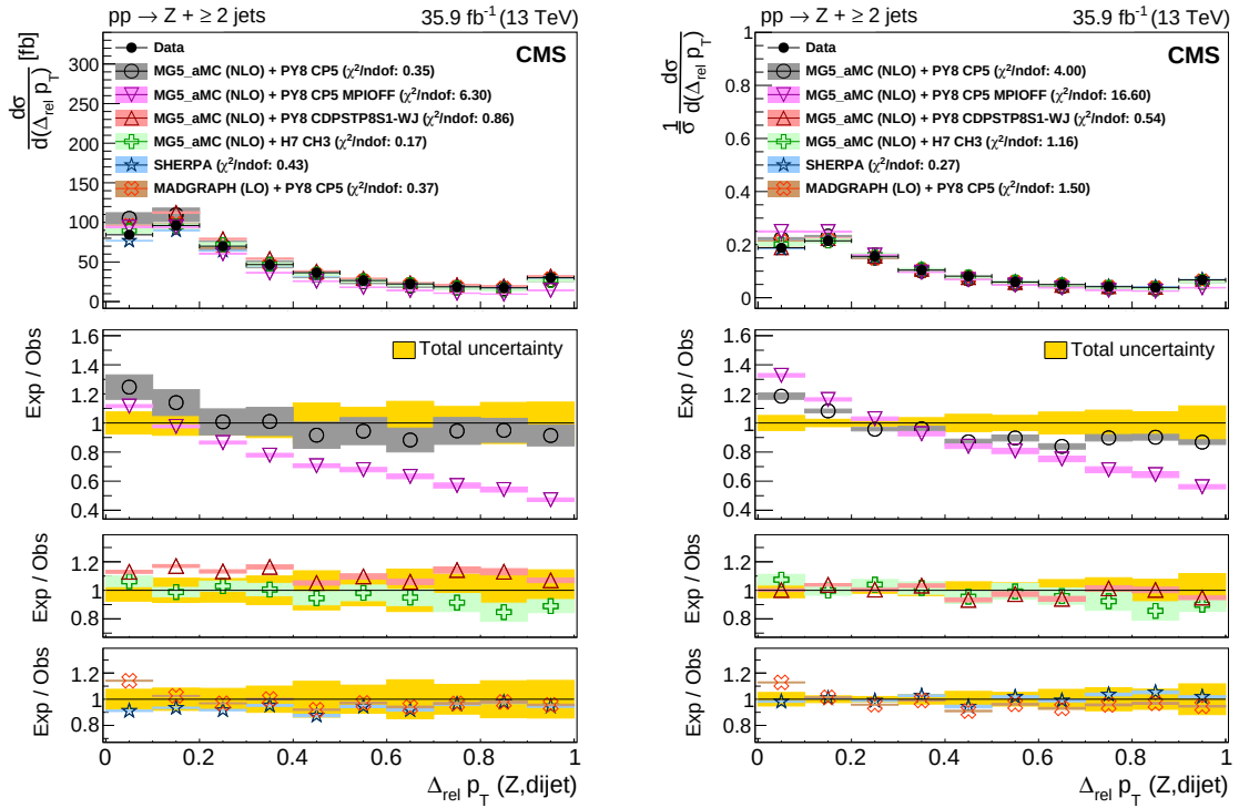
Figure 5: Differential cross sections (left) and area-normalized distributions (right) as functions of the p_T imbalance between the Z boson and the dijet for Z + \geq 2 jet events. The uncertainties in the predictions are shown as coloured bands around the theoretical predictions including statistical, PDF, scale, and tune uncertainties for the NLO MG5_aMC + PYTHIA8 (with CP5 tune) and the statistical uncertainty only for the LO MG5_aMC + PYTHIA8 (with CP5 tune), NLO MG5_aMC + PYTHIA8 (with CDPSTP8S1-WJ tune, CP5 tune with MPI-OFF), NLO MG5_aMC + HERWIG7 (with tune CH3), and SHERPA predictions. In the top panel, the vertical bars on the data points represent statistical uncertainties, whereas in the bottom panels, the total uncertainty in data is indicated by the solid yellow band centred at 1. In the legend, the \chi^2 per degree of freedom is given to quantify the goodness of fit of the model to the data.
