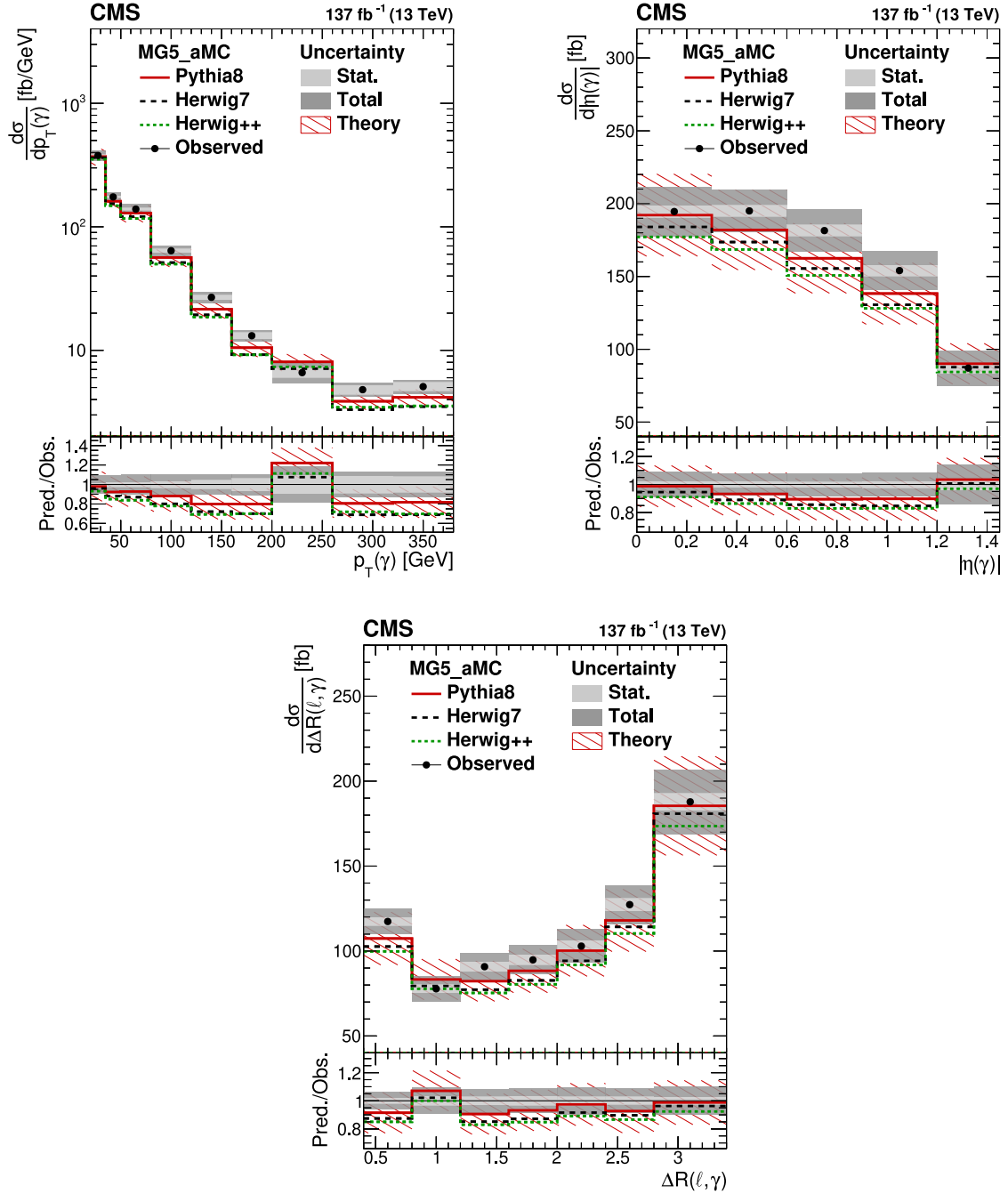
Figure 9. The unfolded differential cross sections for p_T(\gamma) (upper left), |\eta(\gamma)| (upper right), and \Delta R(\ell, \gamma) (lower) compared with simulation obtained from the MADGRAPH5_aMC@NLO event generator interfaced to PYTHIA (red, solid), HERWIG7 (black, dashed) and HERWIG++ (green, dotted) for the parton shower and hadronization. For p_T(\gamma) and \Delta R(\ell, \gamma) , the last bin includes the overflow. The lower panel displays the ratio of simulation to the observation. The inner and outer bands show the statistical and total uncertainties, respectively. Photons radiated from leptons and satisfying \Delta R(\ell, \gamma) > 0.4 are included in the signal and contribute significantly to the first bin of the differential \Delta R(\ell, \gamma) cross section.
