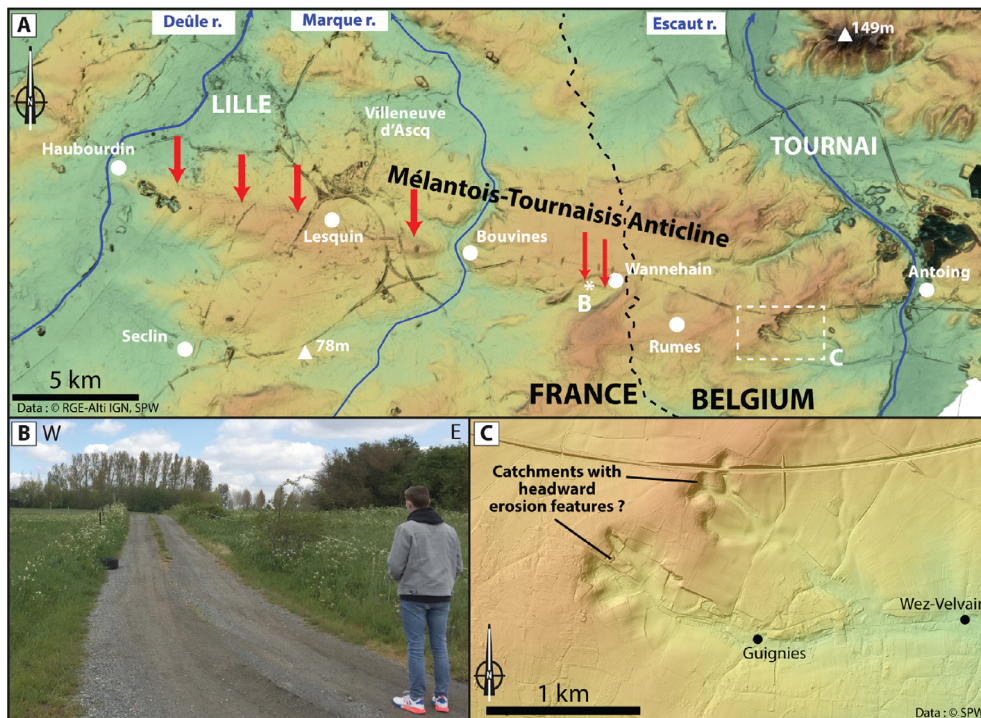
Figure 17. (A) Digital Elevation Model from airborne LiDAR along the Lille-Hazebrouck Fault (see Figure 16) at the hinge of the Mélantois-Tournaisis Anticline (MTA) (data source: IGN-RGE-Alti for France and SPW for Belgium). A several meter WNW-ESE trending topographic scarp is clearly visible between Haubourdin and Lesquin. (B) 1.5 m high topographic scarp observed at Wannehain, corresponding to the eastwards extension of the MTA (B). (C) Catchments with headward erosion features suggesting a recent incision resumption due to local surface uplift (these features are located along the presumably extension of the LHF in Belgium).
