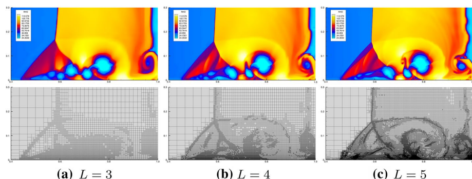
Fig. 15 Shock vortex interaction: adaptive solutions and grids at t = 1 for 3 \leq L \leq 5 using a stretched-dyadic subdivision
