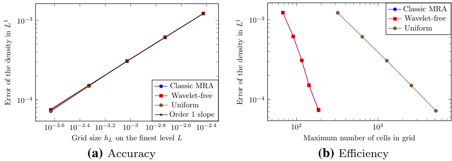
Fig. 8 Sod's test case at time t = 0.25 : comparison of classical approach and wavelet-free approach with the reference scheme using N_0 = 10 and 5 \leq L \leq 9
