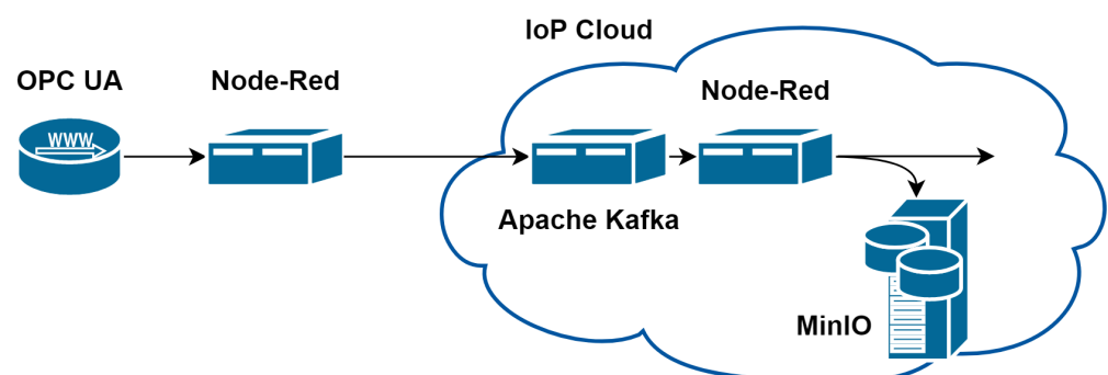
Figure 5. Part of the overall architecture used for load testing.
