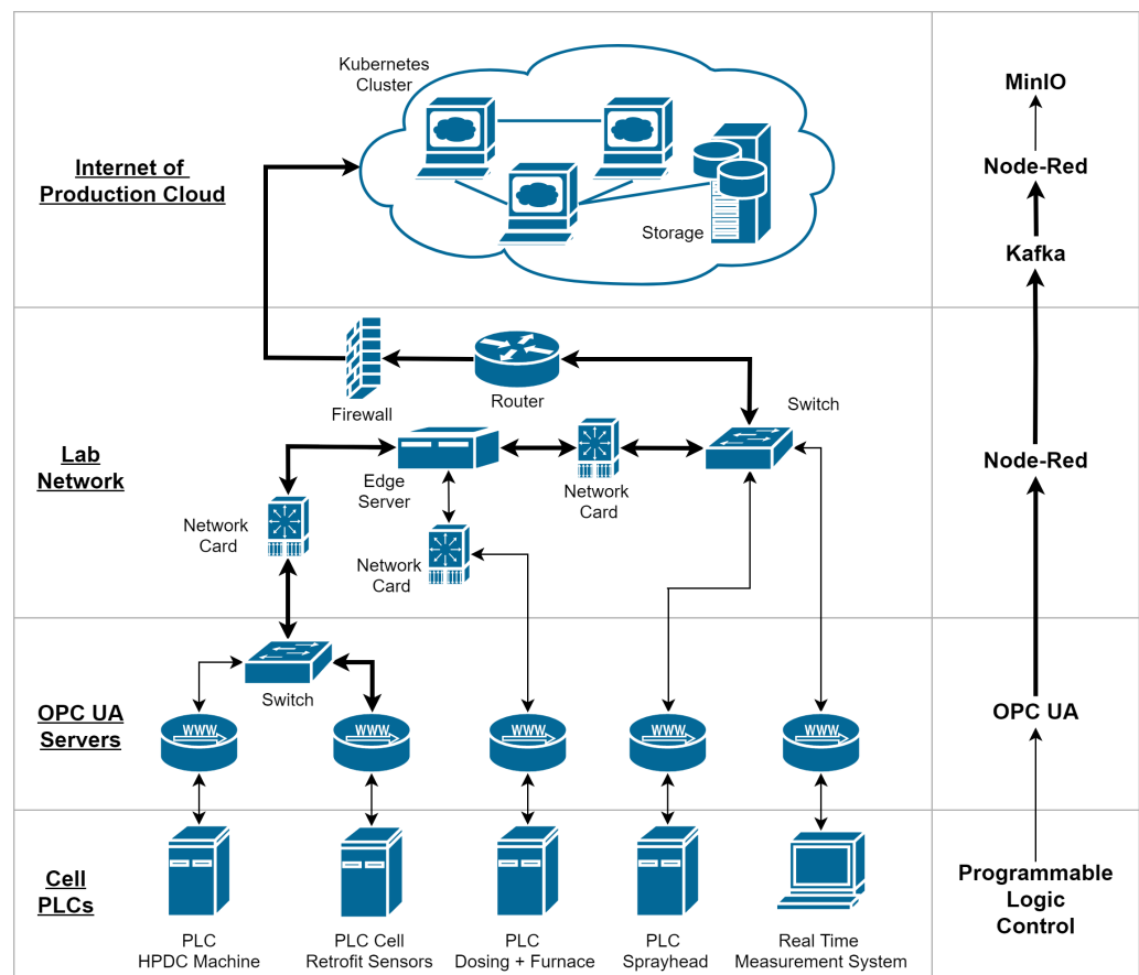
Figure 1. Network layout and technology stack from the HDPC cell to the storage solution.
