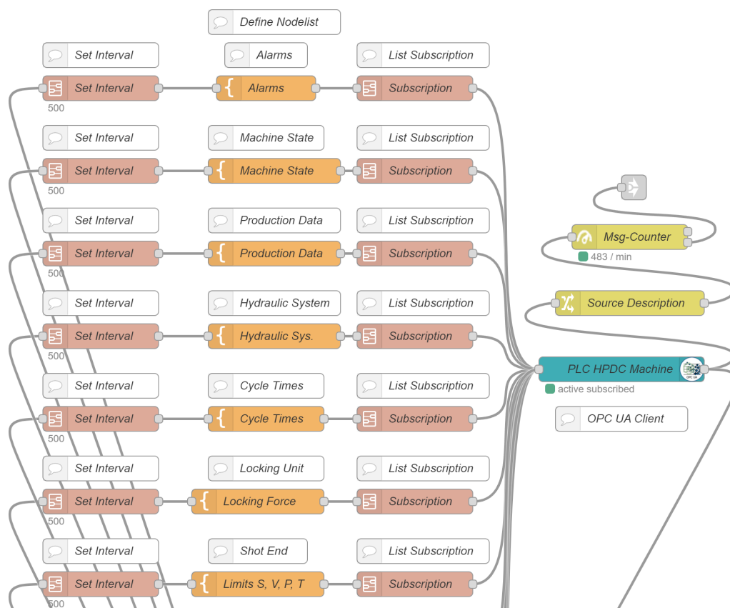
Figure 2. Segment of the flow to access the data from the machine PLC.
