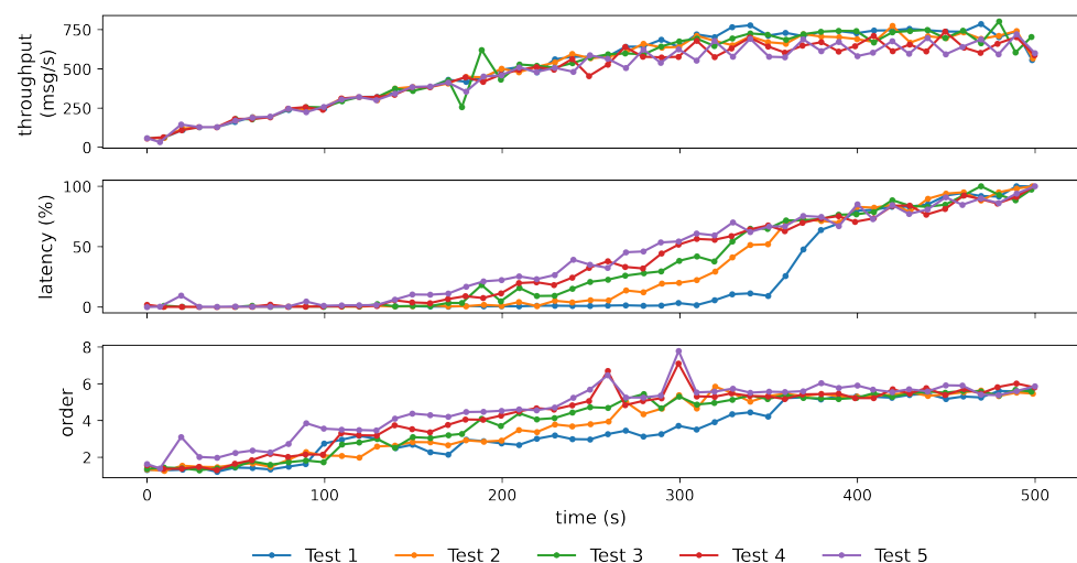
Figure 7. Time dependent metrics of five load tests in identical setups.
