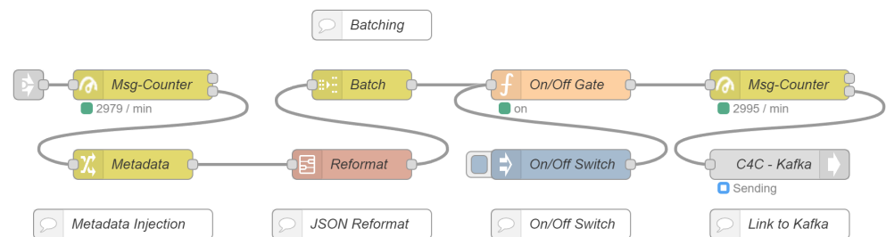
Figure 3. Compounding flow on the edge server that connects to the message broker.
