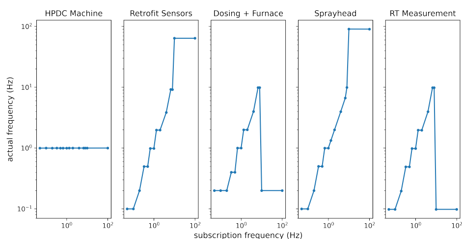
Figure 6. Response to subscriptions to the current time of the OPC UA servers depending on various requested frequencies.
