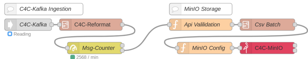
Figure 4. Compounding flow in the cloud that connects the message broker with the data lake.
