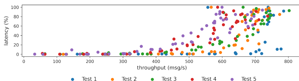
Figure 8. Dependence of latency on throughput measured in five load tests conducted in identical setups.
