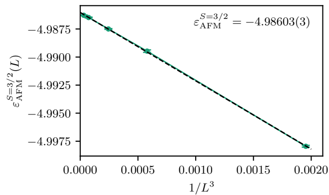
Figure 10: Ground-state energy per site, \epsilon_{\text{AFM}}^{S=3/2}(L) of the spin-3/2 Heisenberg model. The dashed line shows a fit to Eq. (51), which we use to extract the value in the thermodynamic limit.
