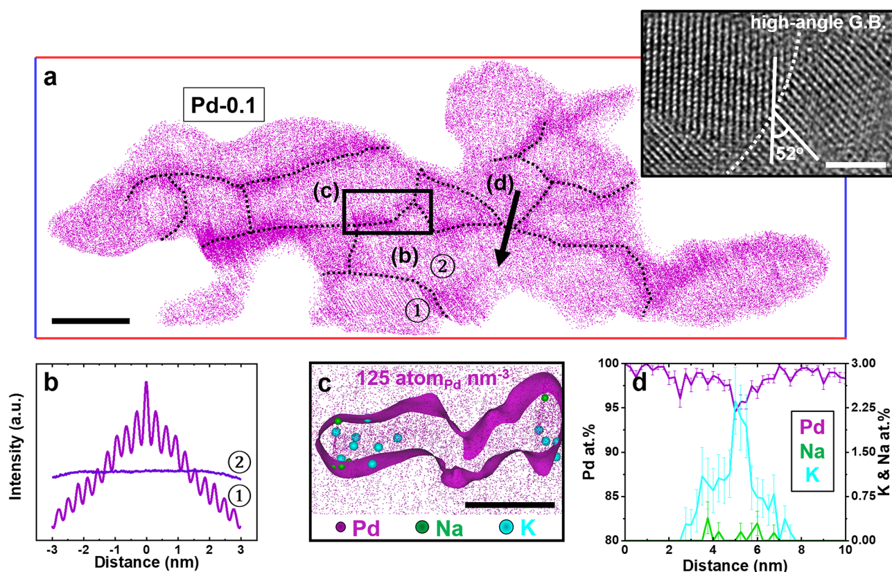
Figure 2. Grain boundary studies for Pd-0.1 nanogels. (a) A 1 nm thin-sliced tomogram from a 3D atom map (Figure S5) of Pd-0.1 gels (iso-composition surface >90 at. % Pd). The scale bar is 10 nm. The dotted black line represents grain boundary features. The inset shows a high-resolution TEM image of Pd-0.1 (scale bar is 2 nm). (b) Spatial distribution maps along the z -axis from the grains of two different nanogels. (c) Extracted grain boundary tomogram with the isodensity surface of 125 Pd atoms/nm 3 . The scale bar is 5 nm. (d) 1D compositional profiles of detected Na, K, and Pd elements.
