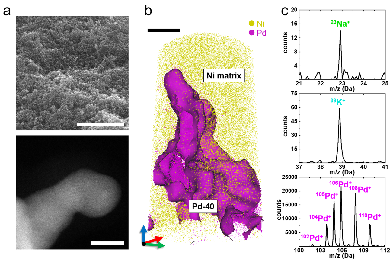
Figure 1. Characterization of Pd-40 nanogels. (a) SEM and HAADF-STEM images of as-synthesized Pd-40 gels. Scale bars are 5 \mu\text{m} and 10 nm for the SEM and STEM images, respectively. (b) 3D atom map of Pd-40 gels embedded in a Ni matrix (scale bar is 10 nm). A one-dimensional composition profile positioned perpendicular to the matrix–MNA interface is shown in Figure S3. (c) Illustration of major and minor peaks in the following three different mass-to-charge ratio ranges: Na, K, and Pd. The overall mass spectrum is presented in Figure S4.
