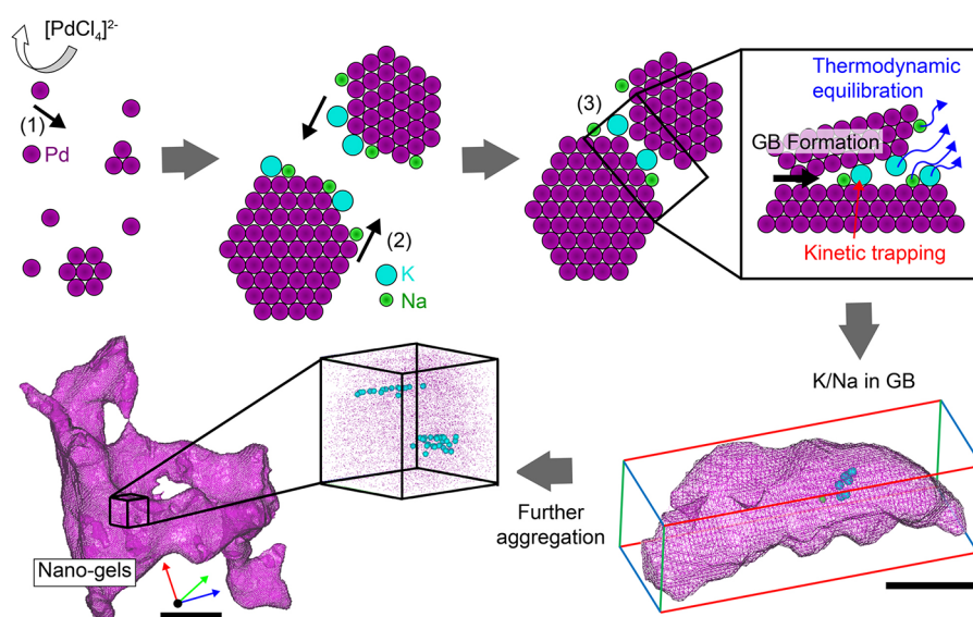
Figure 4. Alkali atom integration mechanism. Schematic illustration of steps comprising the formation mechanism of Pd nanogels, which are as follows: reduction of Pd atoms, formation of a Pd nuclei, coalescence of Pd nanocrystals, aggregation of primary Pd nanogels, and final Pd nanogels. The last two steps are from APT results (scale bars are 5 and 10 nm for the fourth and fifth steps, respectively). Purple wireframes represent the isocomposition surface of Pd at >90 at. %. Green and cyan dots represent Na and K atoms, respectively. During the nanogel formation, (1) the reduction of the Pd precursor to a Pd 0 atom (purple), (2) the absorption of alkali atoms (K (cyan) and Na (green)), and (3) the coalescence of Pd nanocrystals with the integration of alkali atoms into the interface occur rapidly.
