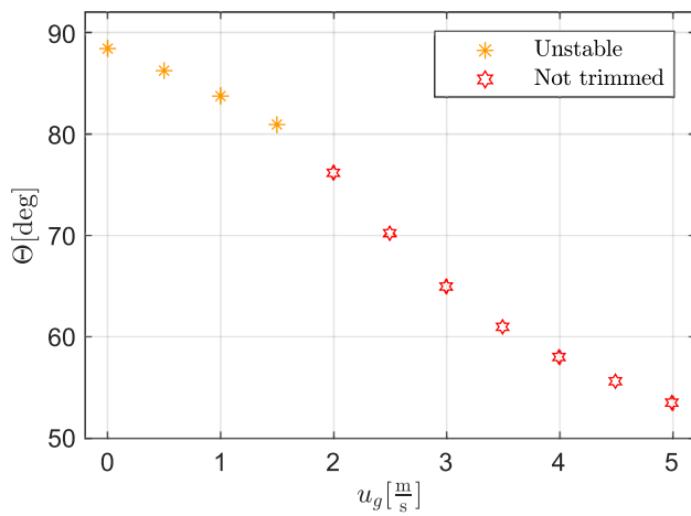
Fig. 10 Pitch angle at w_g = 0 m/s
