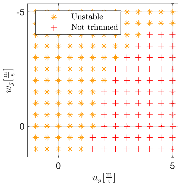
Fig. 9 Trim states during VTOL
