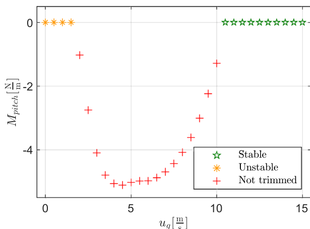
Fig. 8 Resulting pitch moment for w_g = 0 m/s
