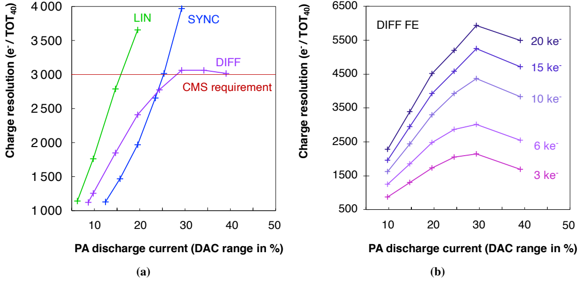
Figure 18. The charge resolution as a function of the PA discharge current (a) measured with a constant charge injection of 6000 e - for the three RD53A AFEs and (b) measured for different input charges for the DIFF AFE only.
