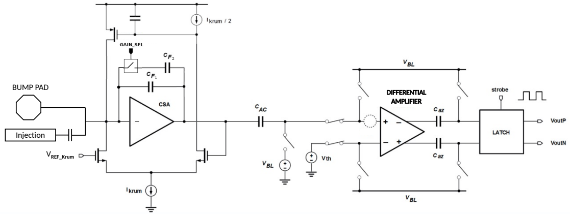
Figure 6. Schematic of the Synchronous front-end implemented in the RD53A chip [13].
