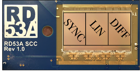
Figure 5. Photograph of the RD53A chip, wire-bonded to a test card, indicating the placement of the three analogue front-ends.
