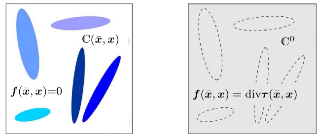
Fig. 5 Left Inhomogeneous microstructure with spatially varying material properties, such as a spatially depending stiffness tensor \mathbb{C}(\bar{x}, x) , while body forces are neglected. Right Homogeneous reference microstructure with a constant reference material behavior \mathbb{C}^0 , while the inhomogeneities are described in terms of the body force f(\bar{x}, x) = \operatorname{div} \tau(\bar{x}, x)
