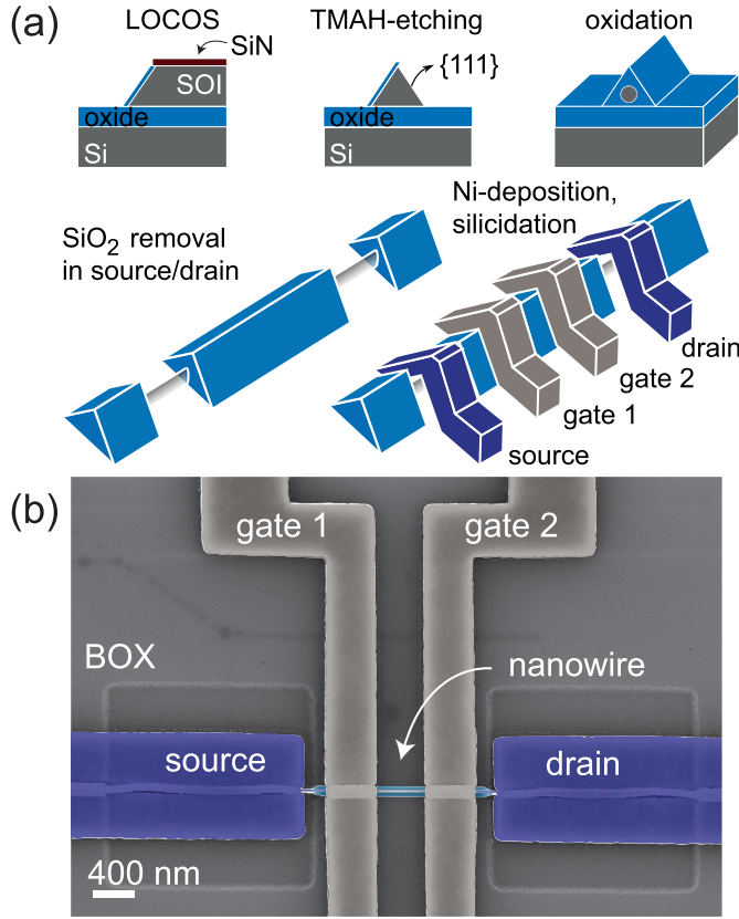
Fig. 4. (a) Schematic illustration of the fabrication process of dual-gate reconfigurable Si nanowire FETs. (b) Scanning electron micrograph of the fabricated device ( d_{nw} \approx 25 nm and d_{ox} > 15 nm) [15].
