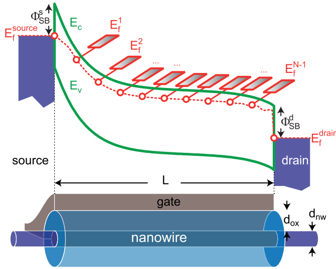
Fig. 1. Conduction and valence bands along the current transport direction of an SB-MOSFET. Metallic source/drain contacts with SB \Phi_{SB}^s and \Phi_{SB}^d are considered. One-dimensional electronic transport is assumed, and scattering is taken into considerations with Buettiker probes. The lower part shows a schematic of the device.
