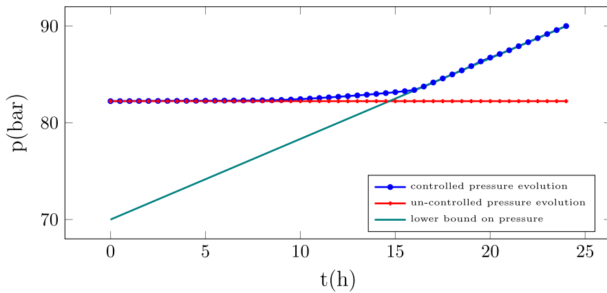
FIGURE 17. Comparison of controlled and uncontrolled pressure at ld_22.
