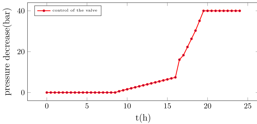
FIGURE 16. Computed optimal control of the valve at nodes 65/66.
