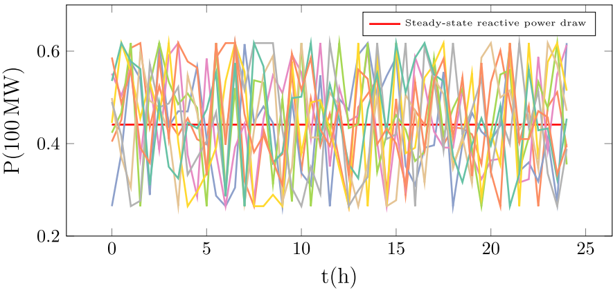
FIGURE 9. Reactive power demand in N1 for deterministic and stochastic demand with \sigma = 0.45 .
