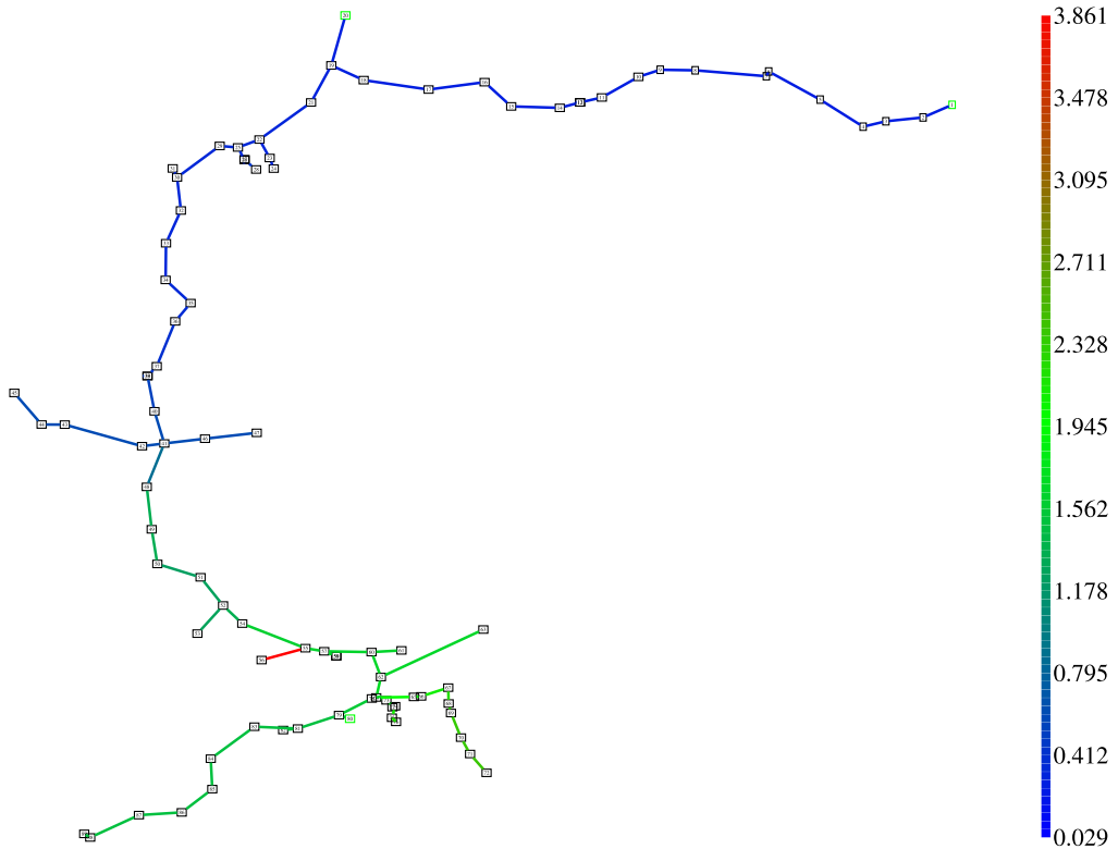
FIGURE 14. Heatmap of the maximal pressure deviation over the course of 24 h, units are in bar.
