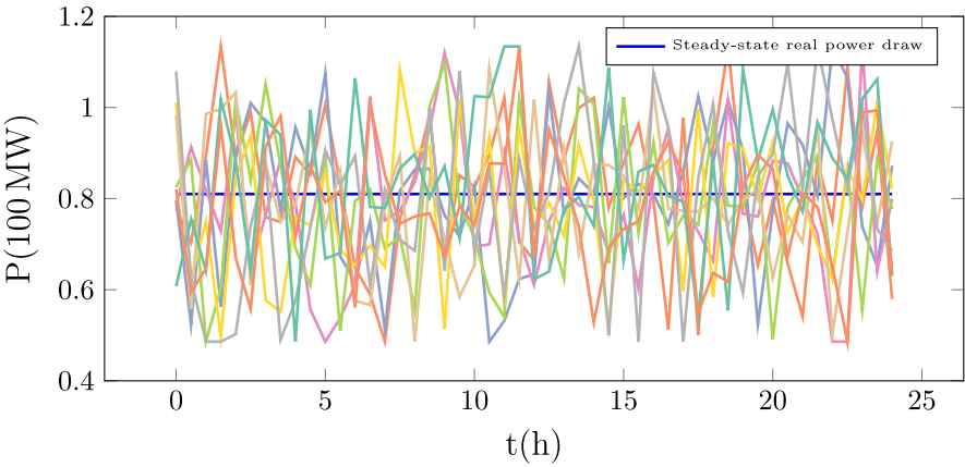
FIGURE 8. Real power demand in N1 for deterministic and stochastic demand with \sigma = 0.45 .
