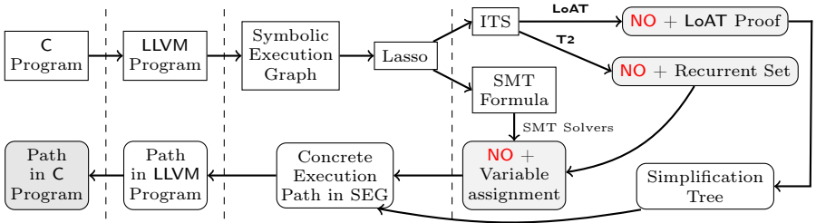
Fig. 1: AProVE's Workflow for Non-Termination Analysis
